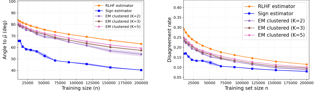
Figure 2: RLHF, EM vs Sign. Angular Estimation error (left) and disagreement rate (right)
