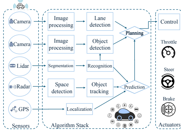
Fig. 1: Holistic overview of the ADS software stack, inspired by [15, 35].
