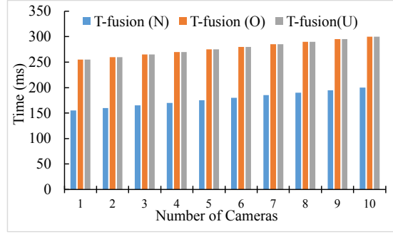
Fig. 8: MRT for three workloads with T-fusion node
