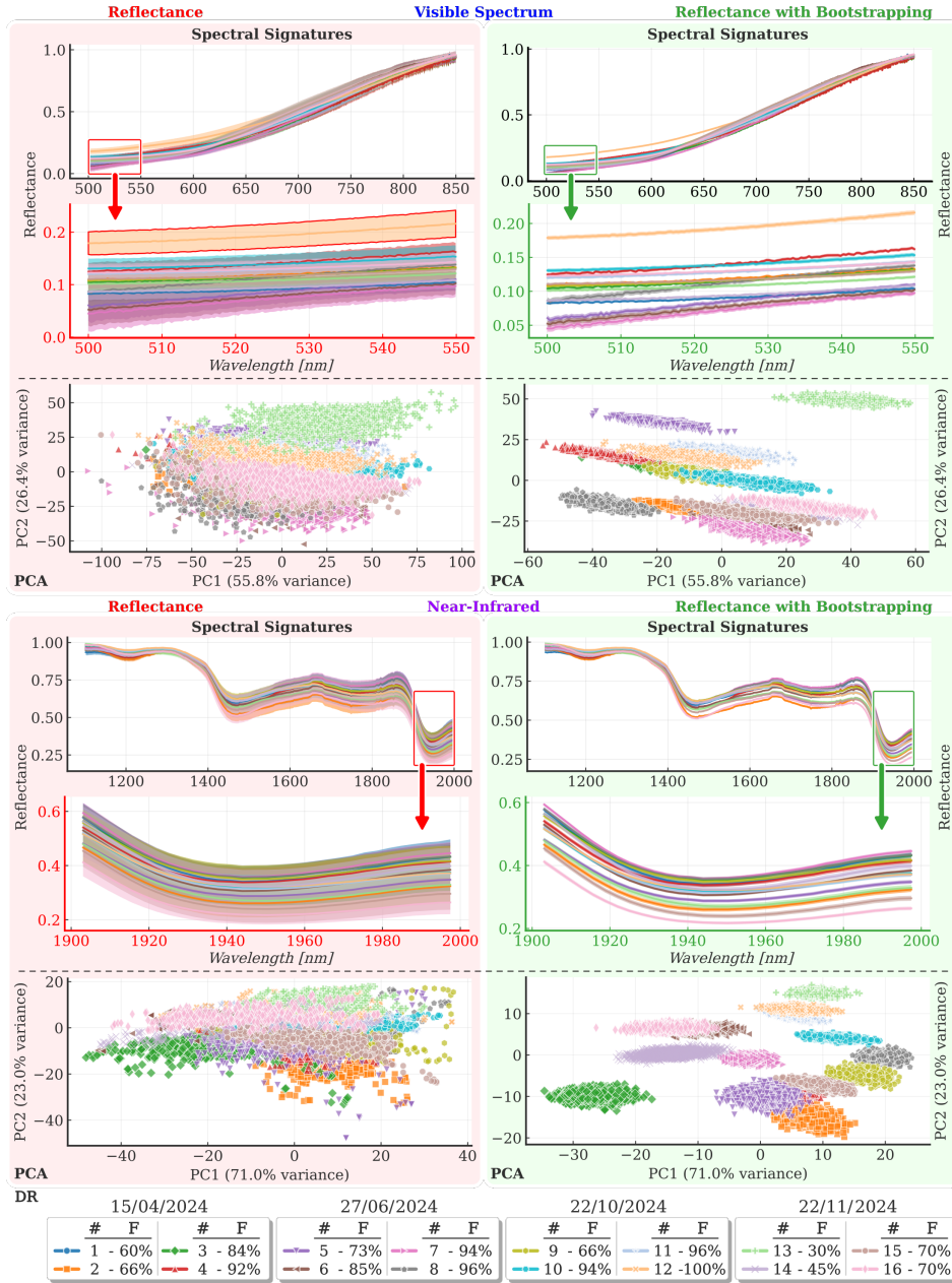
Fig. 5: Raw reflectance vs. reflectance with bootstrapping. Top: reflectance spectra; bottom: PCA projections of cocoa samples from four 2024 dates. Raw data (left) show overlap, especially at 500–550 nm. Bootstrapped averaging (right) reveals clearer batch clustering. DR: Date of Receipt.
