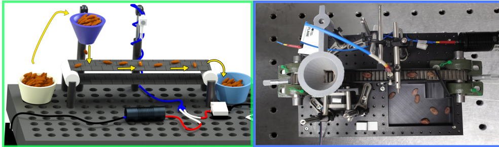
Fig. 3: Automated system for spectral acquisition of cocoa beans. The left panel shows the system design, and the right panel shows its actual construction viewed from above: the conveyor belt, the light source, and the spectrometer for noninvasive data acquisition.
