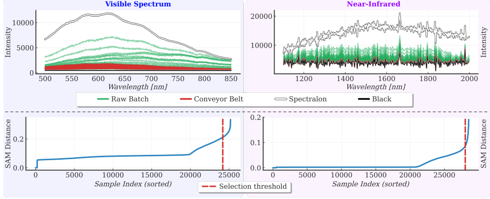
Fig. 4: Raw spectral dataset. Visible (left) and near-infrared (right) intensity spectra for cocoa (green), background (red), and reference targets (black, white). Bottom: SAM distances to conveyor references; red dashed line indicates selection threshold.
