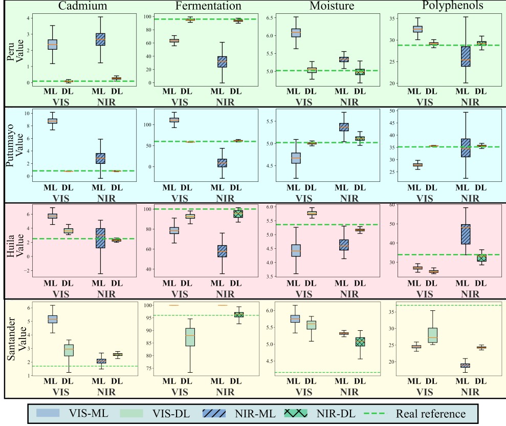
Fig. 6: Predicted versus laboratory values for external cocoa batches using ML and DL models with VIS and NIR spectra. The green dashed line indicates the reference value.
