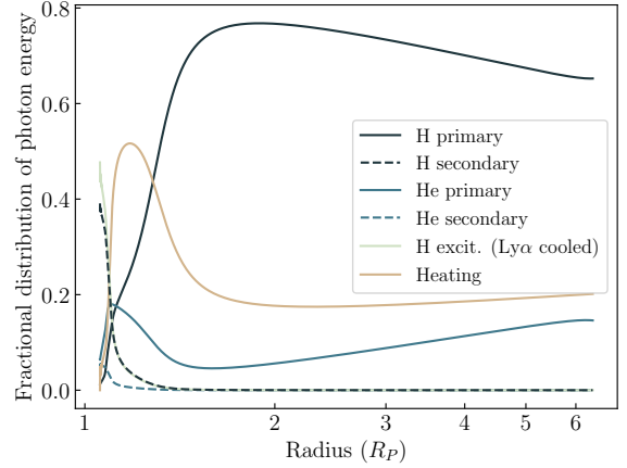
Figure 3. Energy Deposition Fraction for HD 209458b - Fraction of total incident stellar energy into ionizing hydrogen (black), helium (navy), heating (tan), and hydrogen excitation (light green) of which, in our model, 100% is assumed to escape as Lyman- \alpha radiation. Total XUV flux over 13.6-2000 eV is 1095 \text{ ergs s}^{-1} \text{ cm}^{-2} .
