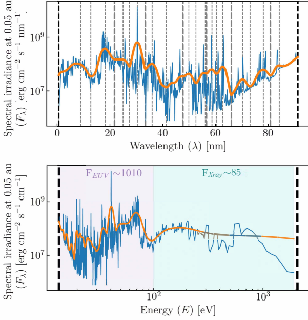
Figure 2. Savitzky-Golay smoothed and binned FISM2 solar spectrum scaled to 0.05 au - Flux at 0.05 au vs. wavelength in nm (top) and vs. energy in eV (bottom). The solid purple and cyan highlights correspond to the EUV (13.6-100eV) and X-ray (>100eV) portions of the spectrum, respectively, and the approximate fluxes of each portion are labeled at the top of the bottom plot in \text{ergs s}^{-1} \text{cm}^{-2} . Bin edges (heavy vertical dashed lines) are automatically set at ionization edges for species present in a given simulation for maximum accuracy in calculating ionization rates (here pure-H). Thin vertical dashed lines are the critical points in the smoothing (Appendix E). We crop our spectra in this investigation at 2000 eV because contributions from higher energies are negligible and most photons that high energy have \tau_\nu = 1 surfaces below the base of the wind and do not contribute to driving the wind. The XUV smoothed spectrum for a pure-H planetary atmosphere (above) results in 59 wavelength bins and the EUV in 66.
