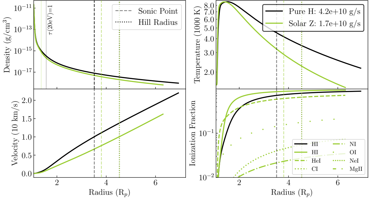
Figure 6. HD 209458b Multispecies - Pure hydrogen (black) and solar abundances of HI, HeI, Cl, NI, OI, NeI, MgII (green) XUV (11.26-2000eV) solutions. Vertical lines: Sonic points (dashed), Hill radius (dotted), \tau(20\text{eV})=1 surfaces (light solid), and solutions end at the Coriolis radius for each simulation.
