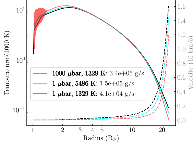
Figure 21. Smoothing high-escape-velocity planet lower BC temperature oscillations - 55 M_{\oplus} , 1.85 R_{\oplus} at 0.05 au with F_{\text{tot}}=1095 \text{ ergs s}^{-1} \text{ cm}^{-2} temperature (right y axis, solid) and velocity profiles (left y axis, dashed). For a lower boundary pressure of 1 microbar, R_{\text{min}} = 1.028 R_P which does not capture the bolometrically heated/cooled region, so T(R_{\text{min}}(1\mu\text{bar})) \neq T_{\text{skin}} = 1324 \text{ K} (red) and results in an order of magnitude higher mass loss than the ground truth (black). Averaging the temperature oscillations tells us the T(R_{\text{min}}(1\mu\text{bar})) = 5486 \text{ K} (cyan) which puts the mass loss rate within a factor of 2. Because neither of these solutions capture the molecular region, there is no higher mean molecular weight or bolometric heating/cooling included. To confirm the validity of this approximation, we lower (black) the base pressure to 1000 microbar ( R_{\text{min}} = 1.016 R_P ) to capture the photoionization base and molecular region, thus making T(R_{\text{min}}(1000\mu\text{bar})) = T_{\text{skin}} = 1324 \text{ K} .
