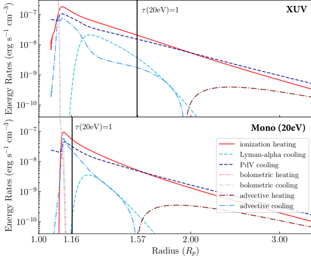
Figure 5. Energy Plot for pure-H XUV vs. Monofrequency HD 209458 b - Energy structure of multi-frequency XUV solution (top panel, cyan solution in Fig. 4) and 20eV monofrequency solution (bottom panel, gray solution in Fig. 4). The \tau(20\text{eV}) = 1 surface for the XUV multispecies is at a higher radius because the deeper penetration of high energy XUV photons puffs up the atmosphere, resulting in higher densities and optical depths at higher radii than in the monofrequency solution.
