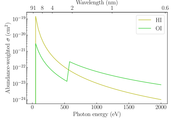
Figure 20. Abundance-weighted Ionization Cross-Sections - Photoionization cross-sections for HI (olive) and OI (lime green) weighted by their fractional abundance (0.79332 and 0.00669, respectively) at 1\times solar metallicity as a function of photon energy (bottom axis) and wavelength (top axis). Frequency-dependent cross sections are derived from coefficients and analytic equations in Verner & Ferland (1996); Band et al. (1990).
