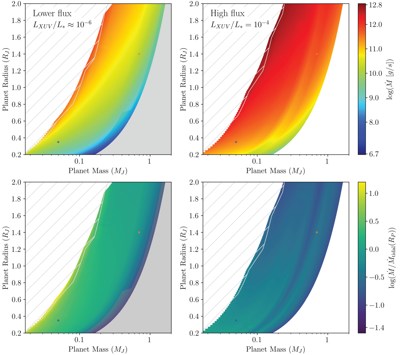
Figure 9. H-He \dot{M} grids for Low and High Fluxes - 2D-linearly-interpolated grid of 663 H-He planets located at 0.05 au around a solar mass, solar luminosity star. Fluxes correspond to an old star ( F_{\text{XUV}} \approx 10^{-6} F_* ) of 1095 \text{ ergs s}^{-1} \text{ cm}^{-2} (left column) and a younger star ( F_{\text{XUV}} \approx 10^{-4} F_* ) of 109500 \text{ ergs s}^{-1} \text{ cm}^{-2} (right column). Locations of a Neptune- and HD 209458b-analog are plotted as blue and orange points, respectively. The grayed out region represents where conductive cooling—which we do not model—would be significant. The hatched region are planets for which R_{\text{sp}} \leq R_{\text{Hill}} (see §5.2). The top row is colormapped to the log of the mass loss rate in g/s and the bottom to the log of the ratio of \dot{M} with the tidally-corrected energy limited \dot{M}(R_P) (Equation 20) with efficiencies calculated on a point-by-point basis in the grid (low-flux \langle \epsilon \rangle \approx 0.37 , high-flux \langle \epsilon \rangle \approx 0.33 ). See §5.1 for a discussion of the bifurcation near 0.1 M_J in the high flux grids.
