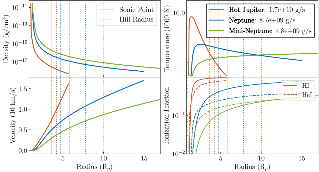
Figure 8. Hot Jupiter, Neptune, and Mini-Neptune H-He Outflows - Wind structure of H-He (0.8:0.2 mass fraction) atmospheres for a 0.7 M_J , 1.4 R_J ( 222.6 M_\oplus , 15.7 R_\oplus ) planet (orange) with escape velocity of at R_P of v_{\text{esc}} = 4.6 \times 10^6 \text{ cm s}^{-1} , a Neptune-sized 17 M_\oplus , 3.9 R_\oplus planet (blue) with v_{\text{esc}} = 2.4 \times 10^6 \text{ cm s}^{-1} , and a mini-Neptune with 5 M_\oplus , 2 R_\oplus (green) with v_{\text{esc}} = 1.77 \times 10^6 \text{ cm s}^{-1} . All three are located at 0.05 au around a 1 M_\odot and 1 L_\odot star, with total flux at 0.05 au of F_{\text{tot}} = 1095 \text{ ergs s}^{-1} \text{ cm}^{-2} (13.6-2000eV). All are plotted in terms of their R_P , but all have different R_P values. The super-Earth’s small thermal inversion below the wind (where larger planets have an isotherm) is the result of bolometric heating/cooling naturally falling off before photoionization heating becomes significant and the wind launches.
