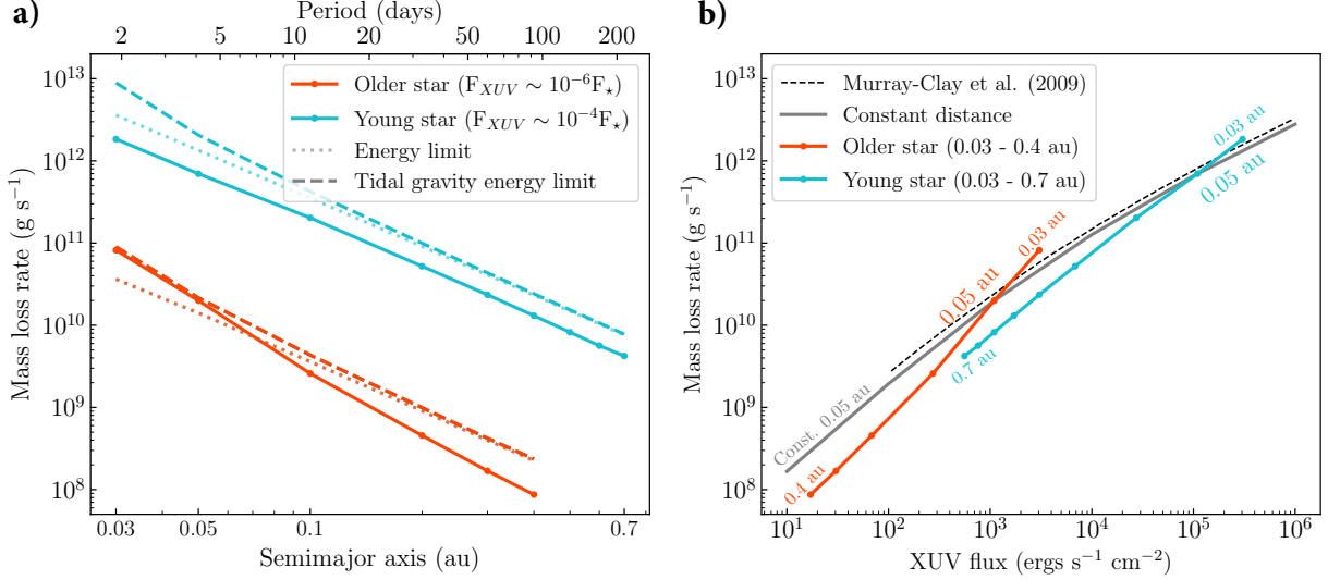
Figure 7. \dot{M} and tidal gravity - (a) \dot{M} for a planet with parameters of HD 209458b and a multi-frequency XUV, H-He atmosphere is plotted as a function of semi-major axis, a , in au (solid lines) for a high XUV activity “young” HD 209458 ( L_{\text{XUV}} \sim 10^{-4} L_{\star} , cyan) and lower XUV flux older HD 209458 ( L_{\text{XUV}} \sim 10^{-6} L_{\star} , orange). Lower/moderate flux is F_{\text{XUV}} = 1095 \text{ ergs s}^{-1} \text{cm}^{-2} and high F_{\text{XUV}} = 1.095 \times 10^5 \text{ ergs s}^{-1} \text{cm}^{-2} at 0.05 au and the stellar spectral shape does not change. Flux scales with a^{-2} . Traditional energy-limited \dot{M} (dotted) and Erkaev et al. (2007)’s tidal-gravity-corrected energy limit \dot{M} (dashed) with our modeled efficiencies (average 0.37, computed point by point as described in Section 3.2) are plotted for both flux regimes. (b) Mass loss is plotted as a function of XUV flux. We reproduce Murray-Clay et al. (2009)’s Fig. 7 (black dashed) for a pure H, 20 eV monofrequency simulation, in which semi-major axis is held constant while flux at 0.05 au is varied. The \dot{M} values are multiplied by the geometric reduction factor of 0.33 for consistency with our current results. The gray line is an update of the previous constant distance line, now with an XUV multi-frequency spectrum and an H-He atmosphere. The computed \dot{M} s for young and older stars from the left are overplotted. The difference in slope is the result of tidal gravity. We assume all planets are tidally-locked, meaning that we use a constant geometric reduction factor.
