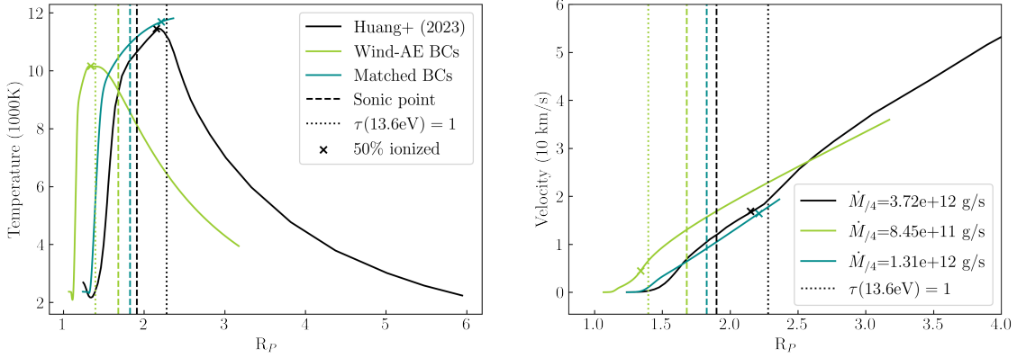
Figure 15. Metals WASP-121 b (Huang et al. (2023)) - WASP 121b: 1.18 M_J , 1.77 R_J , 0.03 \text{ au} , 1.35 M_\odot , 2.6 L_\odot , F_{\text{tot}} = 6.66 \times 10^4 \text{ ergs s}^{-1} \text{ cm}^{-2} . Case B (Huang et al. (2023), Fig. 20) with solar abundances of H I, He I, C I, N I, O I, S I, Mg II, Si II, Ca II, Fe II, K I, and Na I is reproduced in black. Wind-AE models for solar abundances of all of the above species except Fe II, K I, and Na I using our lower BCs (green) and matching BCs (blue) of R_{\text{min}} = 1.24 and \rho(R_{\text{min}}) = 1.39 \times 10^{-11} \text{ g cm}^{-3} . Both have the same input stellar spectrum as black.
