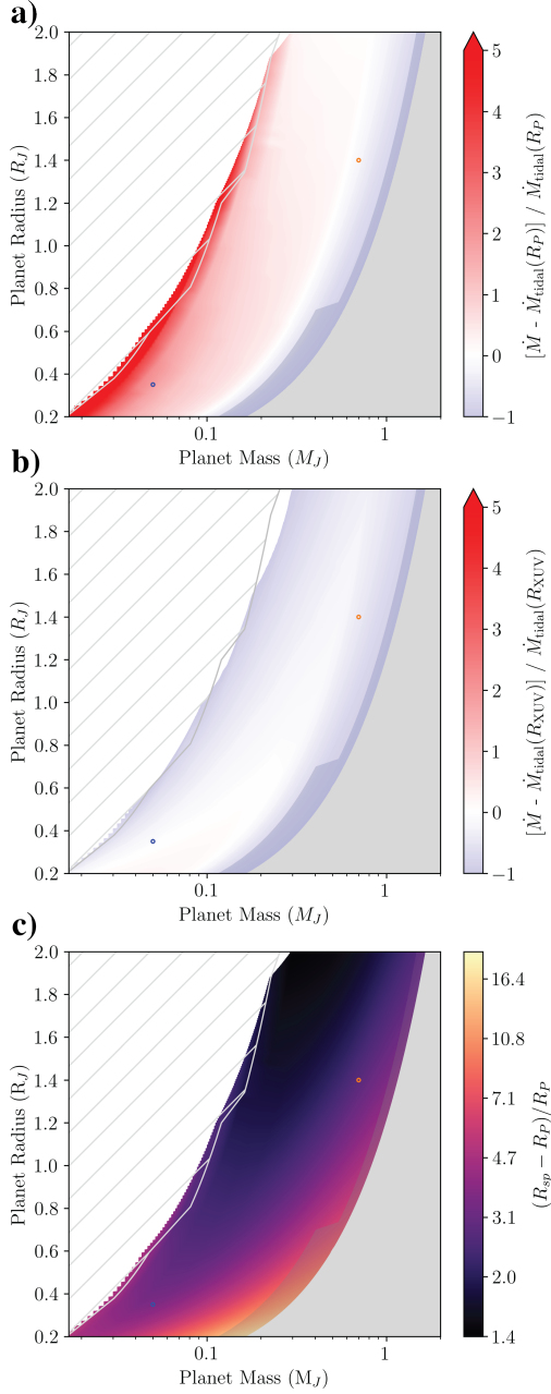
Figure 10. H-He \dot{M} relative to energy limited mass loss rates - (a) Lower flux ( 1095 \text{ ergs s}^{-1} \text{ cm}^{-2} ) fractional difference (\dot{M} - \dot{M}_{\text{tidal}}(R_P))/\dot{M}_{\text{tidal}}(R_P) , from tidally-corrected energy limited mass loss rate computed at R_P . We use the same grid as Fig. 9. Orange and blue dots correspond to an HD 209458b and Neptune-analog, respectively. Red indicates that \dot{M}_{\text{tidal}} underestimates the mass loss rate computed by our model and blue indicates that \dot{M} is less than the energy limit, as is expected. (b) Same colorbar scaling as (a), here we plot (\dot{M} - \dot{M}_{\text{tidal}}(R_{\text{XUV}}))/\dot{M}_{\text{tidal}}(R_{\text{XUV}}) . (c) Height of the sonic point above R_P in units of R_P . All R_{\text{sp}} are below the Hill radii, except at the lowest escape velocity edge (off the left edge of the plot), where the outflow transitions to boil-off or core-powered mass loss—evaluation of our code’s performance in this regime is beyond the scope of this work.
