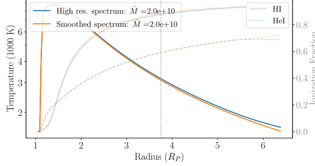
Figure 22. High resolution scaled solar spectrum vs. smoothed - In blue, solutions using the FISM2 LISIRD solar spectrum scaled to an integrated flux of 1095 \text{ ergs s}^{-1} \text{ cm}^{-2} and, in orange, solutions using the smoothed spectrum normalized to the same integrated flux (as in Figure 2). Heavier, darker lines are the temperature profile and lighter, thinner lines are the ionization fraction.
