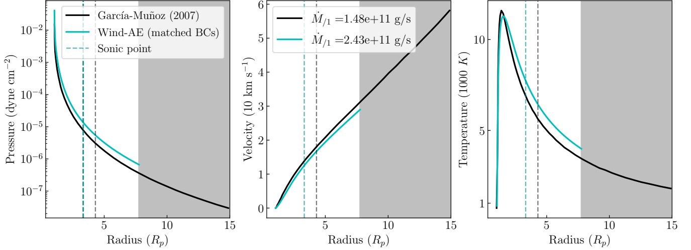
Figure 11. HD 209458b Pure-H García Muñoz (2007) - We reproduce the SP solution of García Muñoz (2007) Figs. 3-4 for an EUV-irradiated pure-H atmosphere (black). Wind-AE solution plotted (cyan) is for a pure-H atmosphere with no Lyman- \alpha cooling, a similar if not identical high activity solar spectrum ( F_{\text{tot}} = 2474 \text{ ergs s}^{-1} \text{ cm}^{-2} integrated over 13.6-165 eV, which loosely simulates H3+ cooling), and BCs matched to those of the black solution ( R_{\text{min}} = 1.03 R_P , T = 730 \text{ K} , \rho = 5.82 \times 10^{-13} \text{ g cm}^{-3} ). Sonic points are dashed lines and the solid gray is the Coriolis radius past which our model is not valid.
