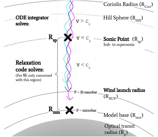
Figure 1. Diagram of wind structure - A thermally-driven, Parker-wind-like outflow is driven by photoionization heating, primarily deposited near the wind launch radius ( R(\tau_{\text{XUV}}) = 1 ). Our relaxation code solves for the structure of this outflow by integrating between two boundary conditions, the minimum radius of the simulation ( R_{\text{min}} ) and the sonic point ( R_{\text{sp}} ), identified by large black ‘x’s. Shorter wavelengths of incident stellar irradiation, like x-rays, are represented by the magenta wave and penetrate deeper into the atmosphere than the longer wavelength dark purple (higher-energy EUV) and cyan (lower-energy EUV). Magnitude of the local velocity, v , relative to the local sound speed, c_s , is given in the middle column. Important planetary radii in the wind’s structure are identified in text in the righthand column (gray semicircle, R_p ; heavy solid, R_{\text{min}} ; light solid, R_{\text{XUV}} ; dashed, R_{\text{sp}} ; dotted, R_{\text{Hill}} ; heavy solid, R_{\text{Cori}} ).
