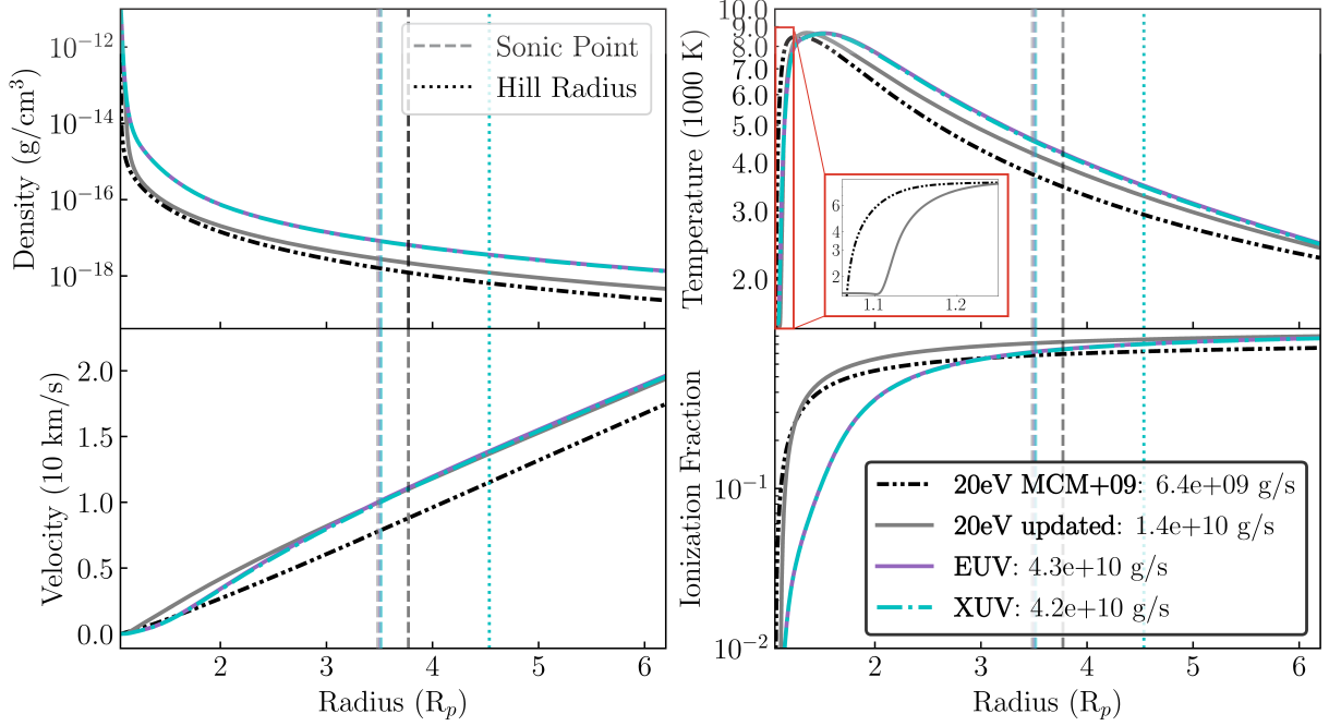
Figure 4. Multi-frequency Profiles for a pure-H HD 209458 b - Black dash-dotted is the original 20eV monofrequency and pure-H Murray-Clay et al. (2009) model ( R_{\min} = 1.037 R_P , \rho(R_{\min}) = 2.7 \times 10^{-11} \text{ g cm}^{-3} , T(R_{\min}) = 1000 \text{ K} ). Gray solid is also monofrequency 20eV, but with our updated physical lower BC and bolometric heating and cooling at the base ( R_{\min} = 1.057 R_P , \rho(R_{\min}) = 1.8 \times 10^{-11} \text{ g cm}^{-3} , T(R_{\min}) = 1534 \text{ K} ). The remaining plots all use the updated BCs. Purple is the EUV multi-frequency (13.6-100 eV) version. Because no metals are present, X-rays (cyan, dash-dotted, XUV 13.6-2000 eV) contribute relatively little to the profiles or mass loss rates of a pure-H atmosphere so the solutions overlie the EUV. Stellar spectra in all simulations are normalized to 450 \text{ ergs s}^{-1} \text{ cm}^{-2} between 13.6 and 40 eV (in keeping with Murray-Clay et al. (2009)). Our model is not valid past the Coriolis radius (upper limit of x-axis). The sonic point and Hill sphere are given by dashed and dotted lines respectively.
