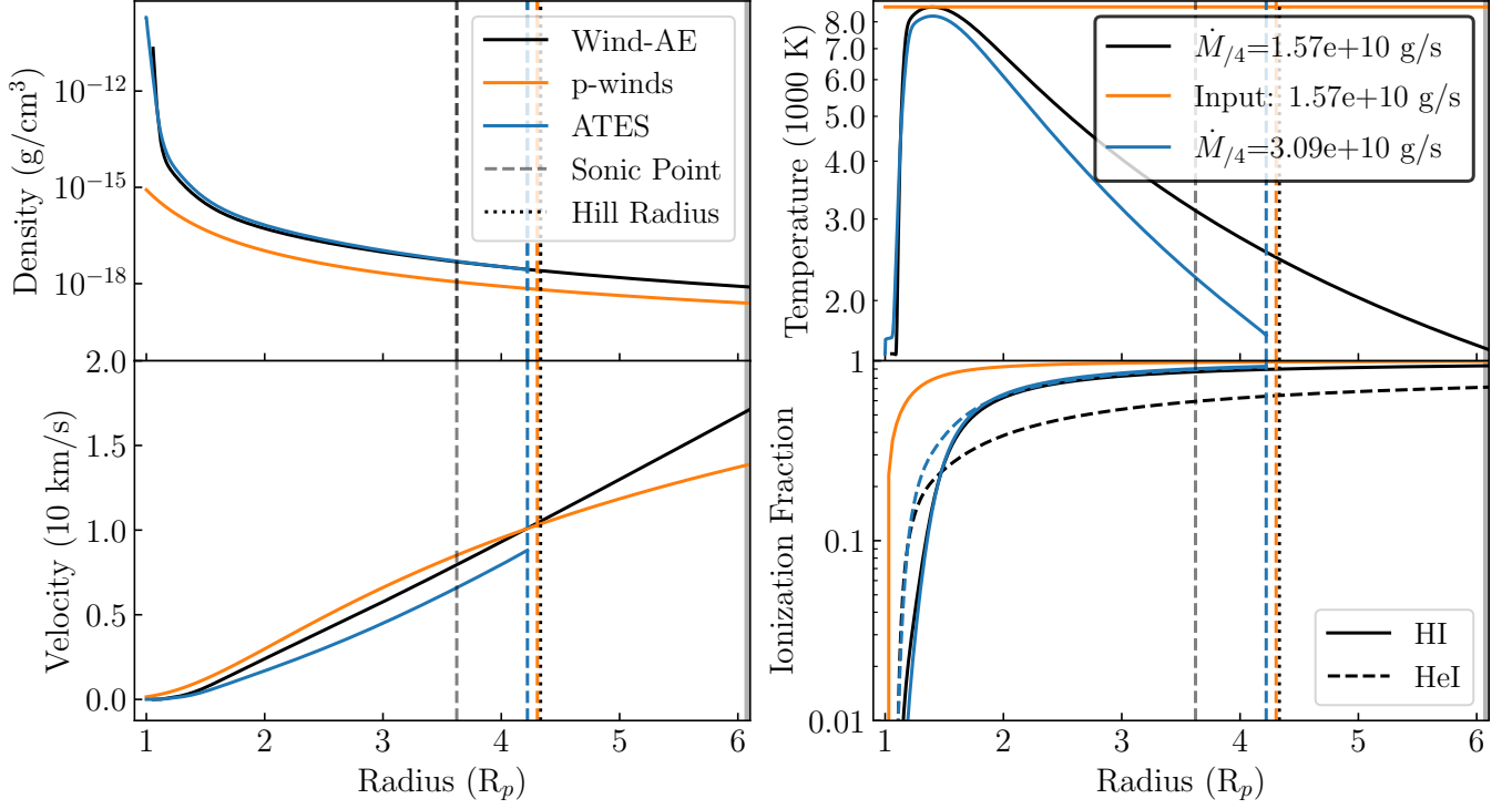
Figure 12. HD 209458b H-He comparisons with ATES and p-winds - Wind-AE H-He (black), ATES H-He (blue, Caldioli et al. 2022 ), and p-winds pure-H (orange, Dos Santos et al. 2022 ) profiles for HD209458b. Inputs to p-winds are T = 8616 and \dot{M} = 1.57 \times 10^{10} \text{ g s}^{-1} (the \dot{M}_{/4} computed by Wind-AE). Sonic points are plotted as dashed vertical lines and the Hill radius as dotted vertical. All three employ different approximations to solar spectra.
