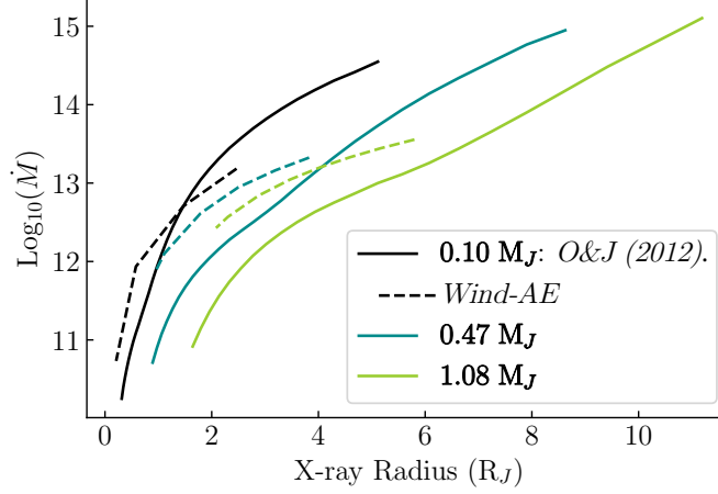
Figure 17. Owen & Jackson (2012) Mass Loss Grid - Solid lines are slices at 0.1 M_J (black), 0.47 M_J (dark cyan), and 1.08 M_J (green) through the mass loss grid for planets at 0.1 au irradiated by a 1 M_\odot star with X-ray luminosity L_X = 10^{30} ergs \text{cm}^{-2} from Owen & Jackson (2012) Figure 5. Note that the radii in that figure are not optical transit radii, but the approximate \tau(1 \text{ keV}) = 1 radius. So we plot the log of geometrically-averaged \dot{M}_{/3} in \text{g s}^{-1} as a function of \tau(1 \text{ keV}) = 1 for planets of the same masses (dashed). The dashed solutions do not extend to higher X-ray radii because planets with higher R_P 's enter the low escape velocity regime in which the relaxation code is currently not well characterized (see §5.2).
