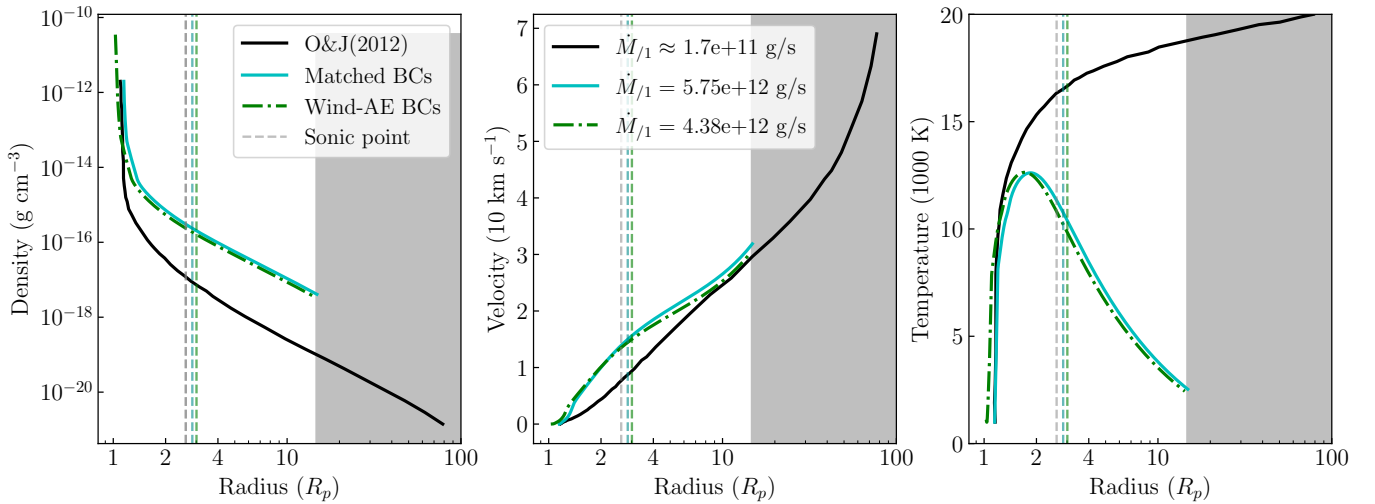
Figure 16. Profiles for Planets in the High X-ray Flux Limit - Reproduction of Owen & Jackson (2012) Fig. 4 (black), a model that does not contain PdV or Ly- \alpha cooling. Density, velocity, and temperature results are given for a 1 M_J , 1.73 R_J (dark) and 5 R_J (light) planet at 0.1 \text{ au} irradiated by a 1 M_\odot star with X-ray luminosity L_X = 10^{30} \text{ ergs s}^{-1} \text{ cm}^{-2} . Wind-AE profiles are plotted for planets with physical BCs (green) and BCs that match those of the black (cyan). To match L_X = 10^{30} \text{ ergs cm}^{-2} , our planets are irradiated by a scaled solar spectrum of total flux 13.6-2000 eV of 3.57 \times 10^5 \text{ ergs s}^{-1} \text{ cm}^{-2} . Sonic points are plotted as dashed vertical lines.
