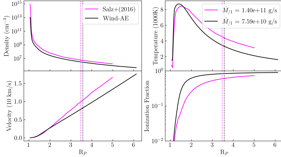
Figure 13. Pure-H HD 209458b TPCI Model - Salz et al. (2016) (TPCI, magenta) has lower BCs of T(R_{\min}) = 1000\text{K} , R_{\min} \sim 1.05R_P , \rho(R_{\min}) \sim 1.6 \times 10^{-9} \text{g cm}^{-3} . We have confirmed that these boundary conditions are not the source of the profile differences.
