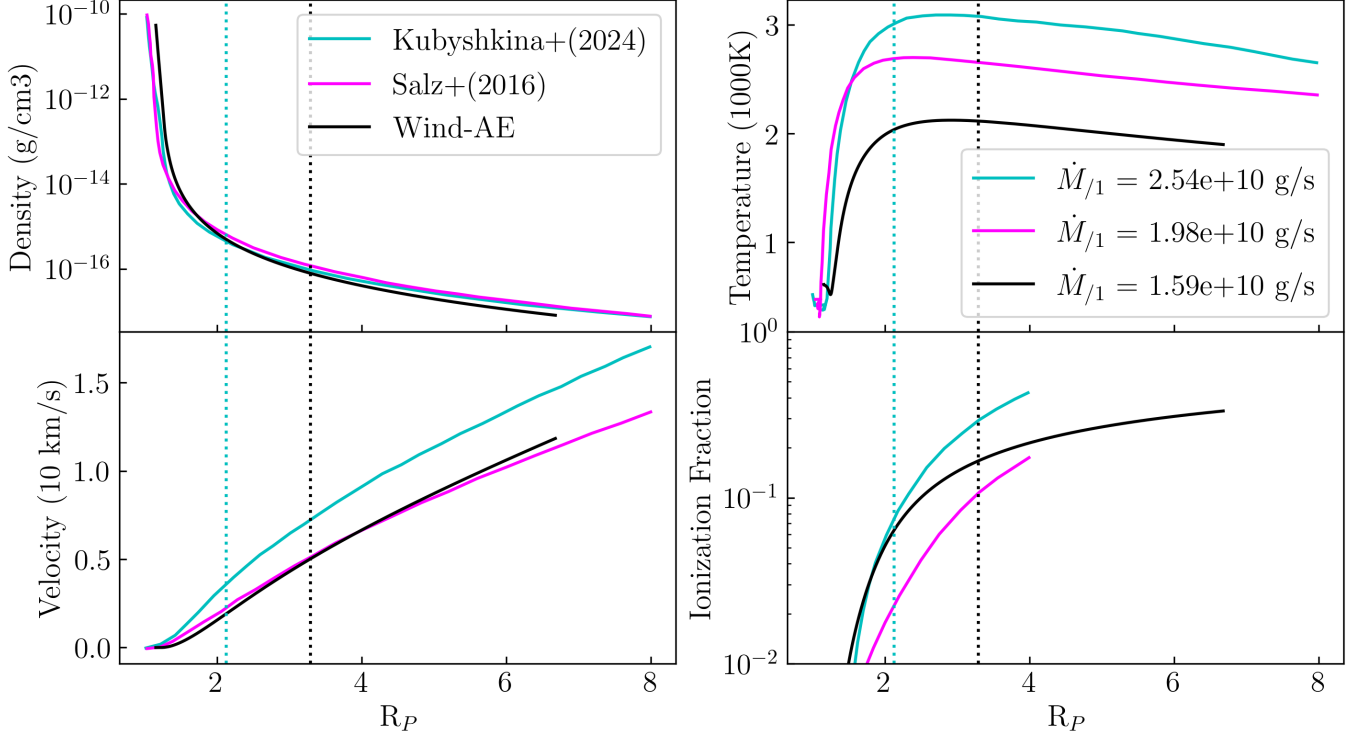
Figure 14. H-He GJ 1214b CHAIN and TPCI Models - GJ 1214b: 6.36 M_{\oplus} , 2.69 R_{\oplus} , 0.014 \text{ au} , 0.18 M_{\odot} , 3.51 \times 10^{-3} L_{\odot} , 886 \text{ ergs s}^{-1} \text{ cm}^{-2} . Kubyshkina & Fossati (2022) CHAIN solar spectrum solution (cyan) and Salz et al. (2016) TPCI solution (magenta) are reproduced here.
