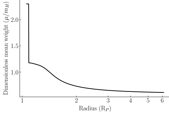
Figure 19. Mean Weight Complementary Error Function Transition - The transition from mean molecular weight \mu(r < R_{\text{XUV}}) = 2.3m_H to mean atomic weight as governed by Equation 14 for HD 209458b. Here the erfc decays over 1 scale height at R_{\text{XUV}} .
