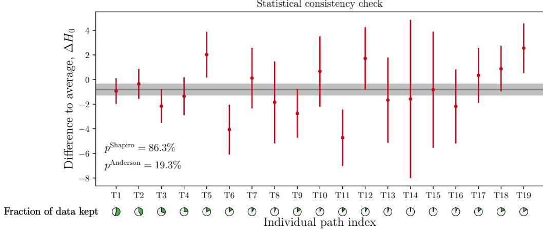
Figure 13. The statistical consistency of various individual paths through the network. These represent a set of paths that are highly correlated, and often only take a tiny part of the network into account. They are used for a statistical consistency check and should not be interpreted as valid variants in the sense of section 2.1.4. We also show the simple weighted mean of these paths in grey purely for visual purposes, reminding that due to their correlations (and selection effects) it need not necessarily agree with the baseline result. For details on the pie charts, see Fig. 12.
