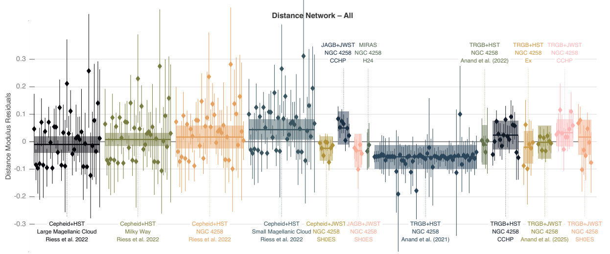
Figure 9. Residuals for host and calibrator distances for the “everything” solution. The groupings, also distinguished by color, correspond to calibrators measured by the same authors with common method and anchor. The error bars reflect the individual calibrator errors; the shaded areas for each group indicate the combined uncertainty in the anchor distance and its reference value, which are in common for all calibrators in the same grouping.
