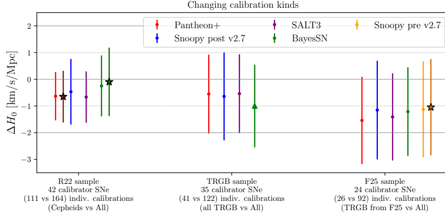
Figure 16. Comparison of H_0 between different ways of calibrating a given set of hosts and a given SN fitter. It is computed as the result with the hosts calibrated through any means minus the result with the hosts calibrated through a specific calibration type (such as only Cepheids, only TRGB, or only F25 TRGB). The results with the star mark the literature results for the given (reduced) set of calibrating a given set of hosts. The triangle shows a case where for the BayesSN fitter only 32 out of the 35 hosts were calibrated due to several missing supernovae.
