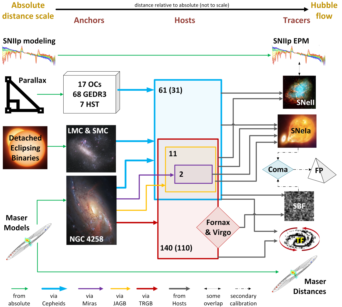
Figure 2. The complete Distance Network, with all possible pathways illustrated. Anchors are objects that establish an absolute scale based on the methods shown to their left. Primary distance indicators (Cepheids, TRGB, Miras, JAGB) transfer the absolute scale to hosts (i.e., galaxies), the ensemble of which calibrates secondary distance indicators in the Hubble flow (tracers). Exceptions are Megamasers and astrophysically modeled SNe II, both of which serve as primary distance indicators and are capable of reaching the Hubble flow without intermediate steps. Green arrows illustrate direct connections between anchors or tracers and the method used to determine the absolute scale. Blue, violet, yellow, and red arrows show which calibrators constrain host distances; line width qualitatively distinguishes the attainable precision. Among hosts, rectangles qualitatively indicate overlap among objects measured via multiple methods. Diamond shapes represent groups. Dark gray arrows tie subsets of hosts whose distance is constrained by different calibrators to tracers. Any given arrow may represent multiple data sets, e.g., HST or JWST photometry of Cepheids, or optical vs. infrared photometry of SNe Ia. The number of hosts is labeled for Cepheids, TRGB, JAGB, and Miras, with the number of hosts exclusively available to each method shown in parentheses.
