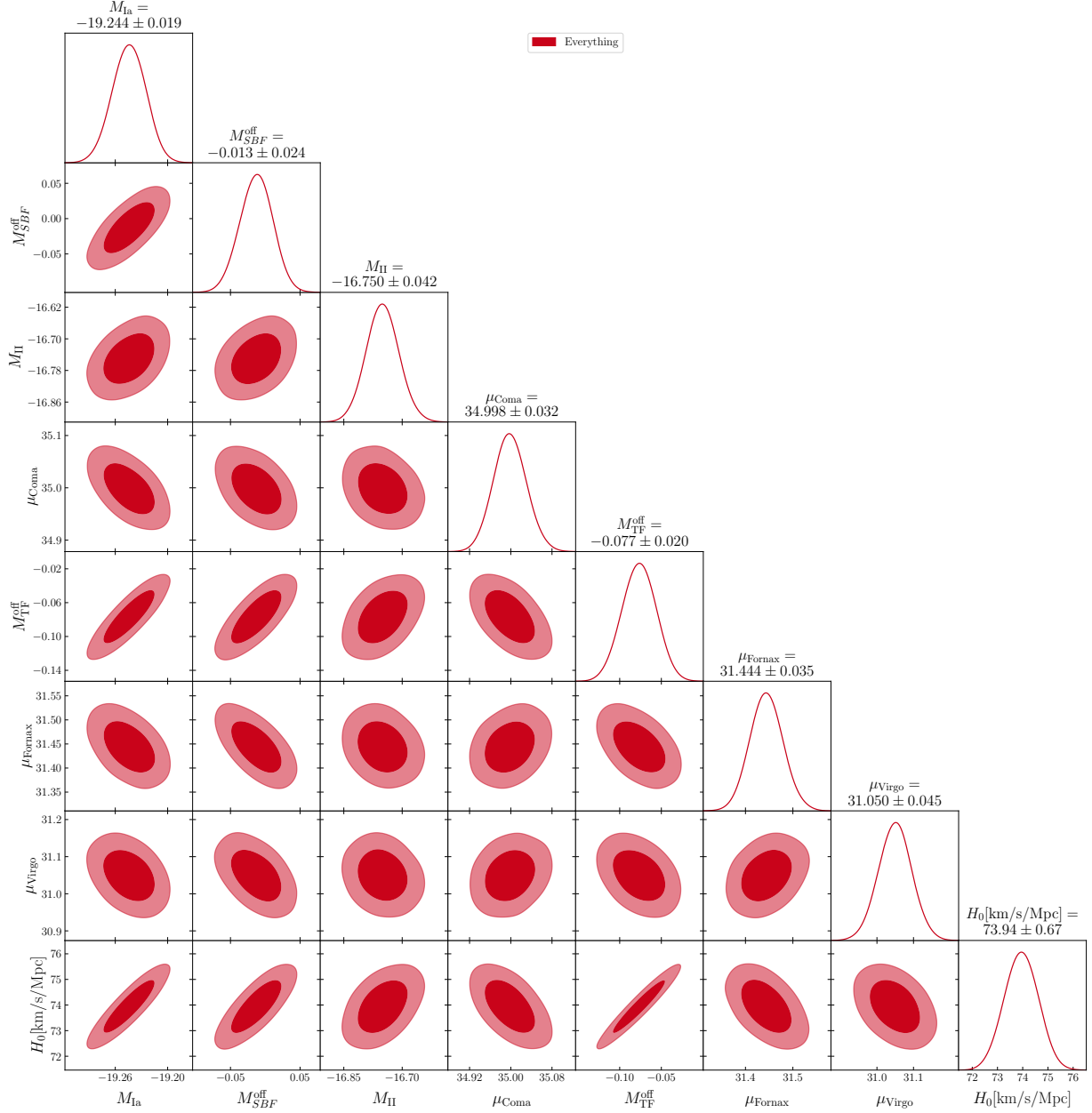
Figure 11. Corner plot illustrating the main optimization parameters for the all-inclusive solution, using the naming convention of Appendix B.3.1. Parameters related to individual host distances are not included. Note that this solution is not an alternative result to the baseline solution, but rather a variant to check the impact of further data on our result, see also Section 5. We show it here to highlight the existing correlations between the various (most important) solution parameters. Deviations from the analytically calculated result are due to the numerical precision of a finite-length chain.
