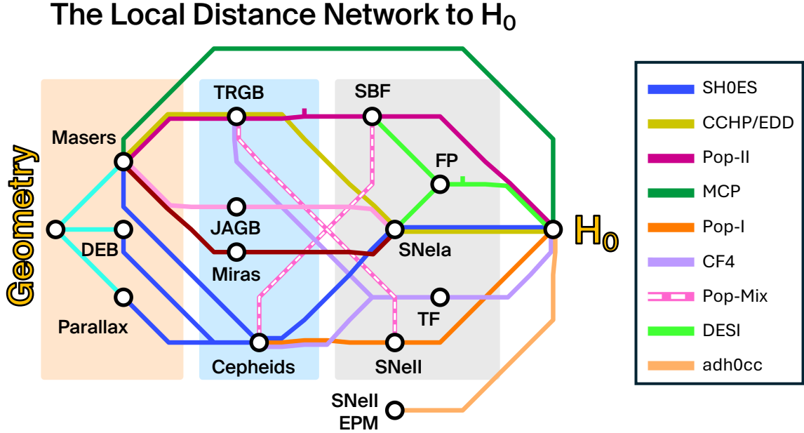
Figure 1. Conceptual overview of the Local Distance Network, a many routes approach. Different methods for distance determination may connect the absolute scale determined by geometric means to H_0 . A non-exhaustive list of baseline linkages discussed in the literature or the paper is labeled on the right. Links to geometric distances provided by Masers, DEB, and Parallax are indicated as available in our analysis. Background rectangles in orange, light blue, and gray indicate where Rung 1, Rung 2, and Rung 3 of a traditional distance ladder would fall. Unlabeled tickmarks represent Groups (Fornax & Virgo for the TRGB to SBF, Coma for FP). Example references: A. G. Riess et al. (2022a, SH0ES), W. L. Freedman et al. (2025, CCHP), G. S. Anand et al. (2021, EDD), G. S. Anand et al. (2024a, Pop-II), D. W. Pesce et al. (2020a, MCP), T. de Jaeger et al. (2022, Pop-I), E. Kourkchi et al. (2020, CF4), K. Said et al. (2025, DESI), C. Vogl et al. (2025, adh0cc). Appendix C.1 replicates a subset of these routes.
