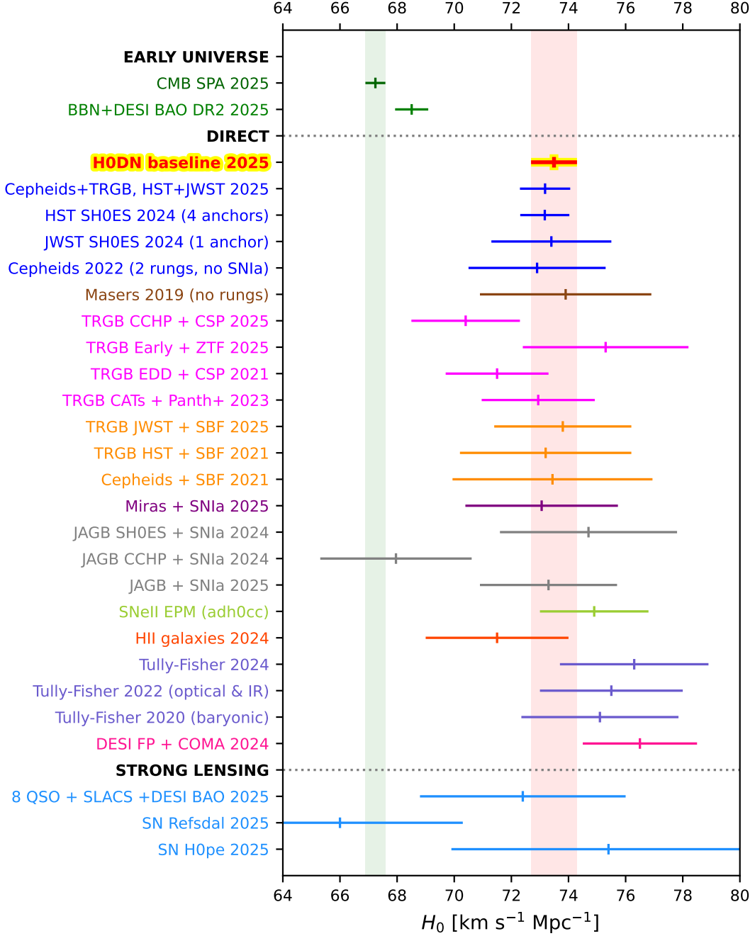
Figure 7. Comparison of the baseline result with previous literature results, based on early universe indirect inferences using the flat \Lambda CDM model, based on direct measurements in the late universe, and based on strong lensing results (which involve additional modeling).
