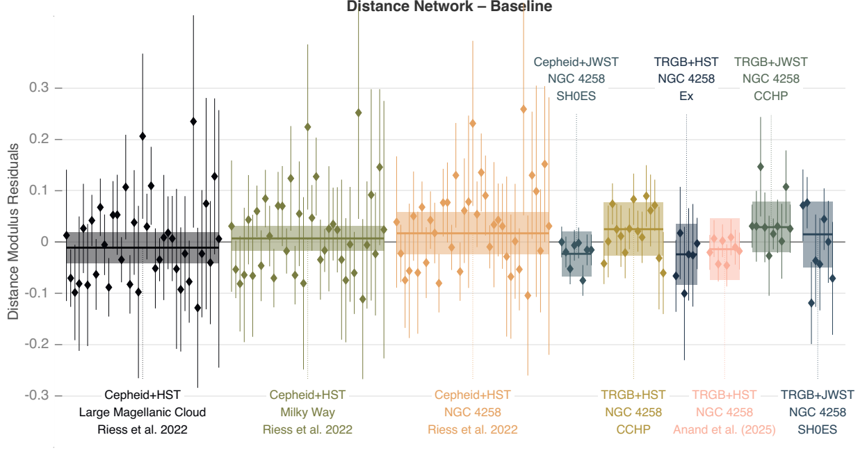
Figure 4. Residuals for each category of host distance measurements from the Baseline solution. Each panel represents a group of measurements of host distances that share the same method, anchor, and authors, and shows the deviation of those measured host distances from the full distance network value. Error bars represent the individual uncertainty of each measurement, while the shaded regions for each group shows the common (fully correlated) uncertainty due to the reference system.
