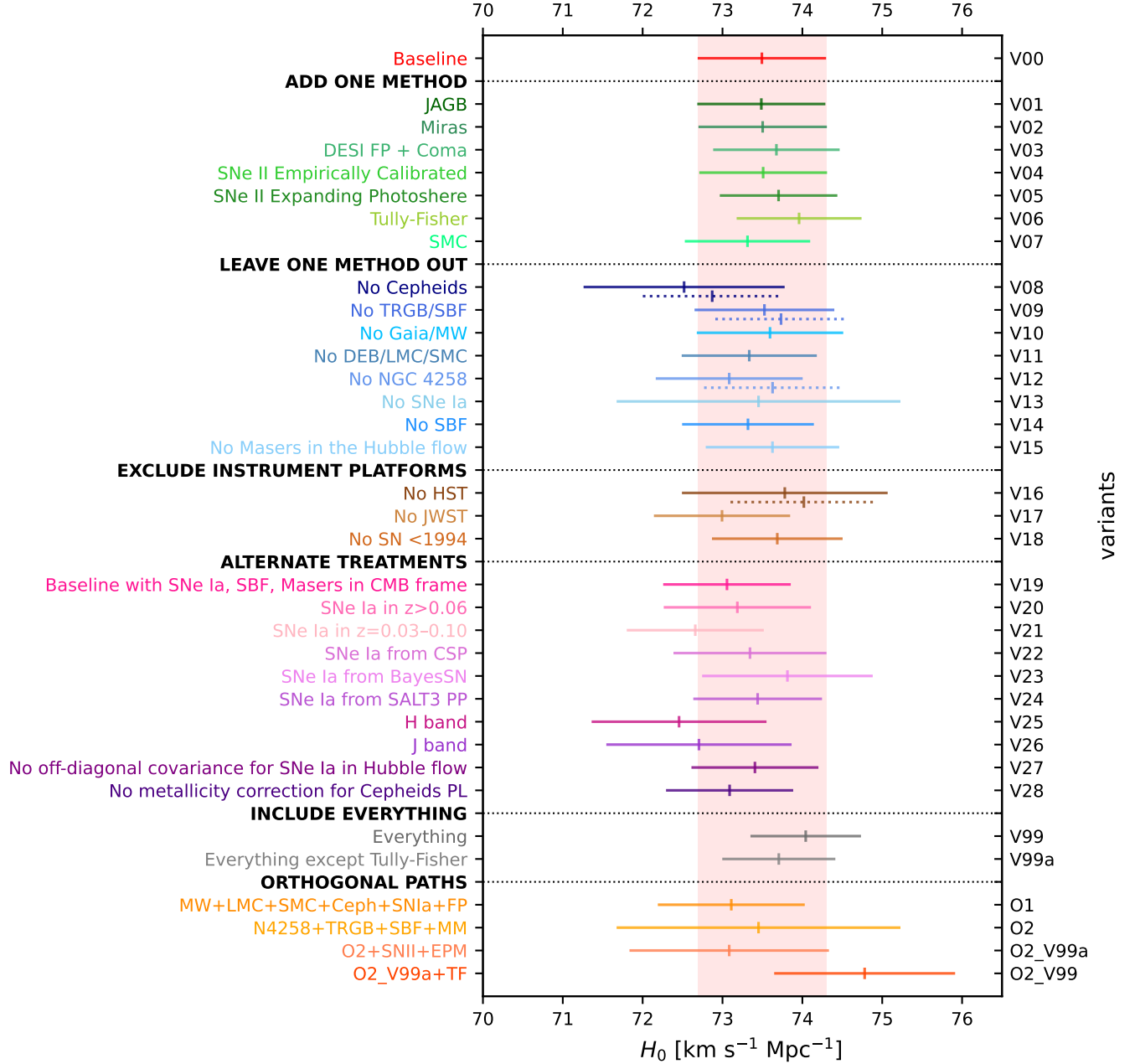
Figure 8. Baseline and variants results from Table 4. For some variants, a labeled change has a secondary consequence (i.e., removing the identified primary distance indicator also results in the loss of calibration to some SN Ia). In these cases a dashed line immediately below such variants provides a custom baseline—i.e., the same SNe are removed before the removal of the primary indicator—is shown to provide a custom reference of impact for that variant; see text for details.
