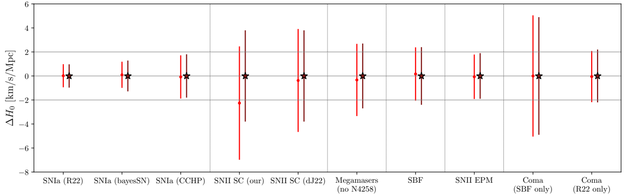
Figure 17. All literature comparisons for the given configuration/method (see x-axis label and main text). The light red results are the results for the given configuration/method coming from the Distance Network, while the dark red results are those available in the literature (differences are always zero but illustrates literature uncertainties), see also Table 9.
