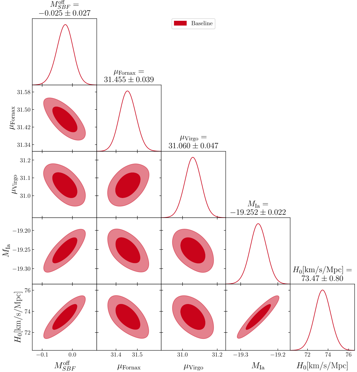
Figure 6. Corner plot for the baseline solution, illustrating the correlations between H_0 , the calibration of SNe Ia and SBF, and the distance to Fornax and Virgo, which contribute to the SBF calibration. The parameters use the naming convention of Appendix B.3.1. Deviations from the analytically calculated result are due to the numerical precision of a finite-length chain.
