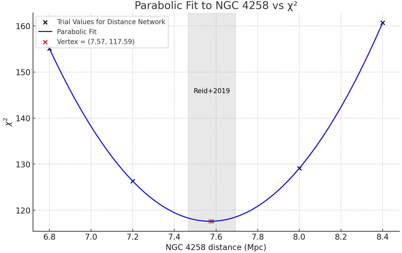
Figure 18. Trial values for the distance to NGC 4258 and associated \chi^2 values. Besides the M. J. Reid et al. (2019) measure at D = 7.58 \pm 0.11 Mpc (shown as grey band) we also tried increasing or decreasing the distance by \pm 5\% and 10\% (black crosses). The result is a large internal inconsistency in the distance network (due to other geometric anchors) which is highly significant. See also Table 10 for impact to H_0 . The global minimum (vertex) is marked by a red cross.
