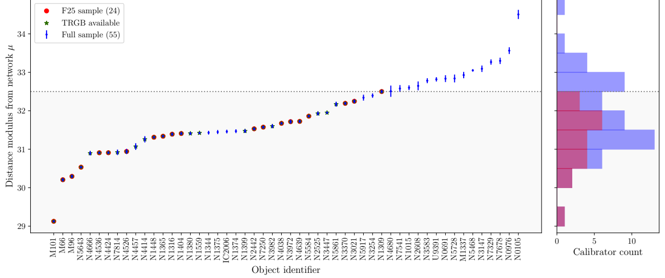
Figure 15. The full network sample (blue) and the F25 sample of calibrator hosts (red) in comparison. The grey region marks the maximal extent of the F25 sample. The green stars mark hosts with TRGB distances available. The left hand side shows an ordered scatterplot of the distance moduli, while the right hand side shows the corresponding histogram. Note that while F25 calibrates 24 SN Ia, these are located in only 20 hosts (hence only 20 points are marked red). The 11 additional hosts marked with green stars would correspond to potentially 10 additional SNe Ia (with the 11th host NGC 1399 calibrating SBF, not SNe Ia). One additional SN Ia (2021pit) is present in an already F25-calibrated host (N5643) but not within the CSP sample. In total that makes 24+10+1=35 calibrators that are available for SNe Ia calibrated through TRGB. Even within the sample of the CSP I&II supernovae only, there would still be 4 additional CSPI&II calibrators to be gained using TRGB observations of nearby hosts within the range of the F25 sample—with 7 additional TRGB-calibratable SNe Ia not present within the CSP I&II samples. The 4 “missing” TRGB-F25 calibrators are 2012ht in NGC 3447, 1998aq in NGC 3982, 1992A in NGC 1380, and ASAS14-lp in NGC 4666.
