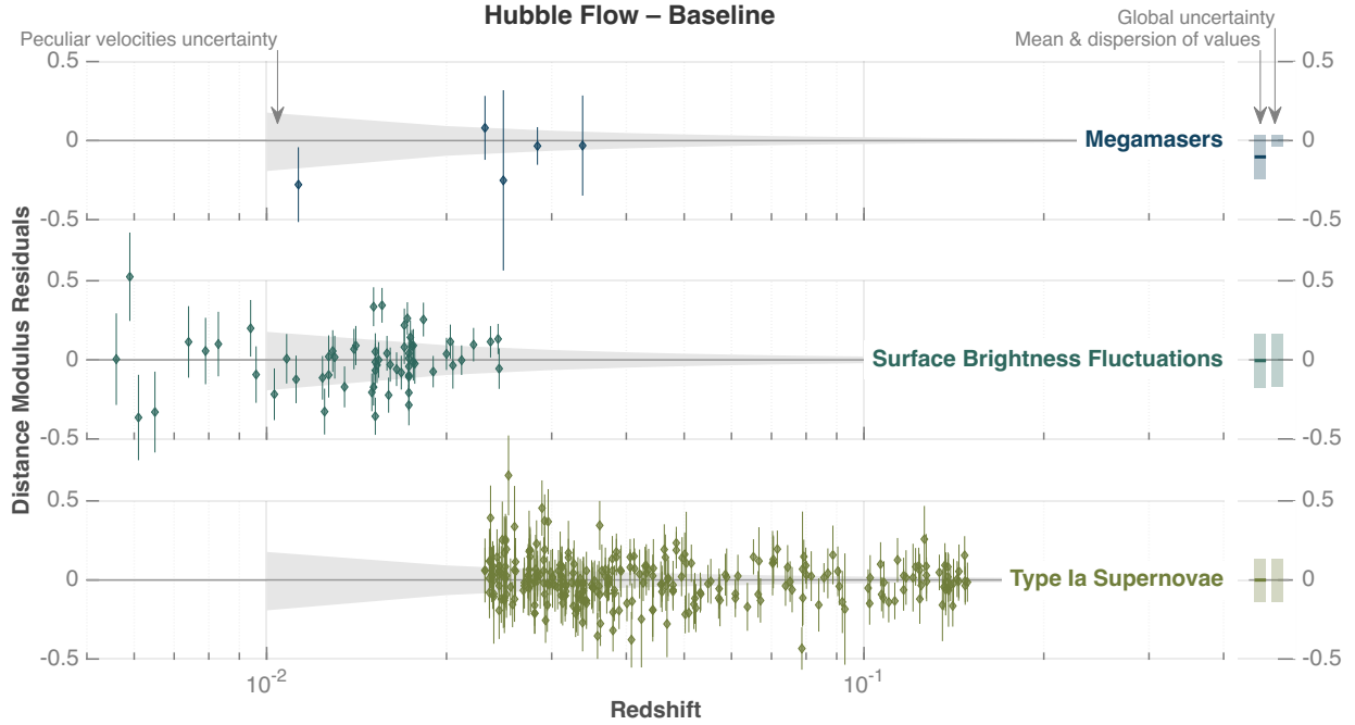
Figure 5. Residuals in distance modulus as a function of redshift for objects in the Hubble flow in the Baseline solution. Error bars reflect the individual source scatter, without the common calibration uncertainty. The shaded region in each plot indicates the effect of a velocity uncertainty of 250 \text{ km s}^{-1} . The bars at the right show the mean and dispersion for each group of sources and the calibration uncertainty, which is a common error mode for all points in each panel.
