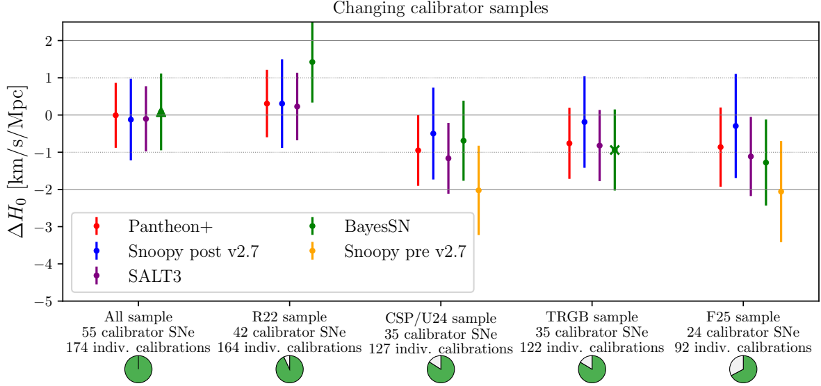
Figure 14. Comparison of the impact of supernova type Ia calibrator samples (sets of hosts) on the Hubble constant inference H_0 , each one relative to the baseline result, for the various light curve fitting codes. The triangle shows a case where for the bayesSN fitter only 52 out of the 55 hosts was calibrated due to several missing supernovae in the fit, and the cross one where only 32 out of 35 hosts were calibrated. For details on the pie charts, see Fig. 13. In this case we take 100% of the pies to be the case involving all supernovae data instead of the baseline.
