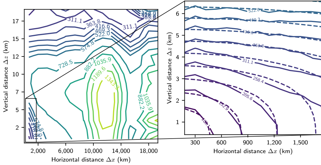
Figure 7: Empirical two-dimensional horizontal/vertical structure function calculated from IGRA radiosonde data (solid; labels in \text{m}^2\text{s}^{-2} ). For the inset, a fit (dashed) was performed using Eqn. 9, with best-fit parameters described in text.
