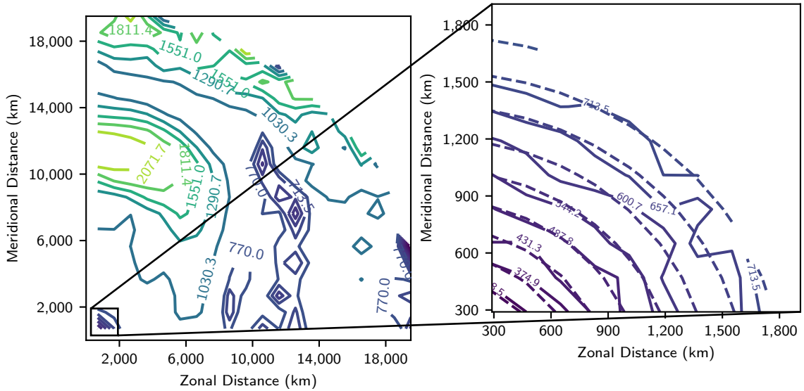
Figure 8: As in Fig. 7, but for isoheight statistics calculated as a function of meridional and zonal direction.
