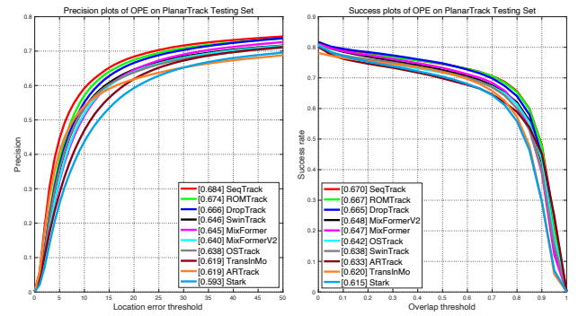
Figure 15: Performance of evaluated generic visual trackers on PlanarTrack BB using bounding box-based precision and success plots. To facilitate clearer analysis, we exclusively present the top 10 trackers. Best viewed in color.
