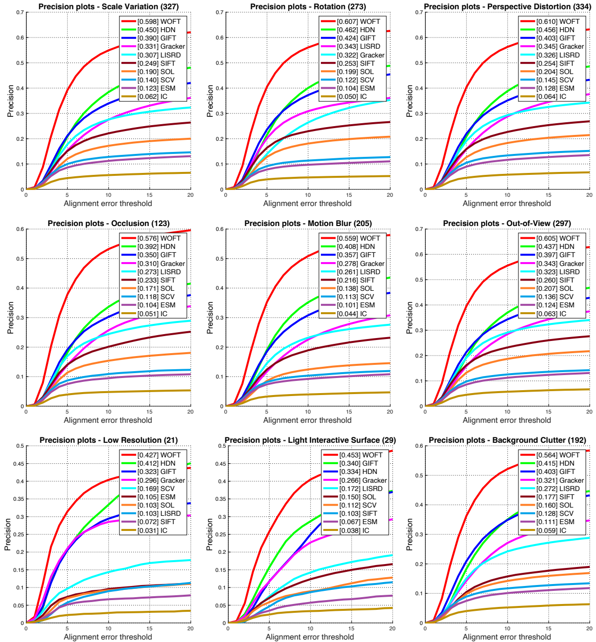
Figure 12: Precision plots of trackers on each challenging factor using P@15 score. Best viewed in color
