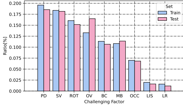
Figure 8: Distribution of challenging factor on training and testing sets.
