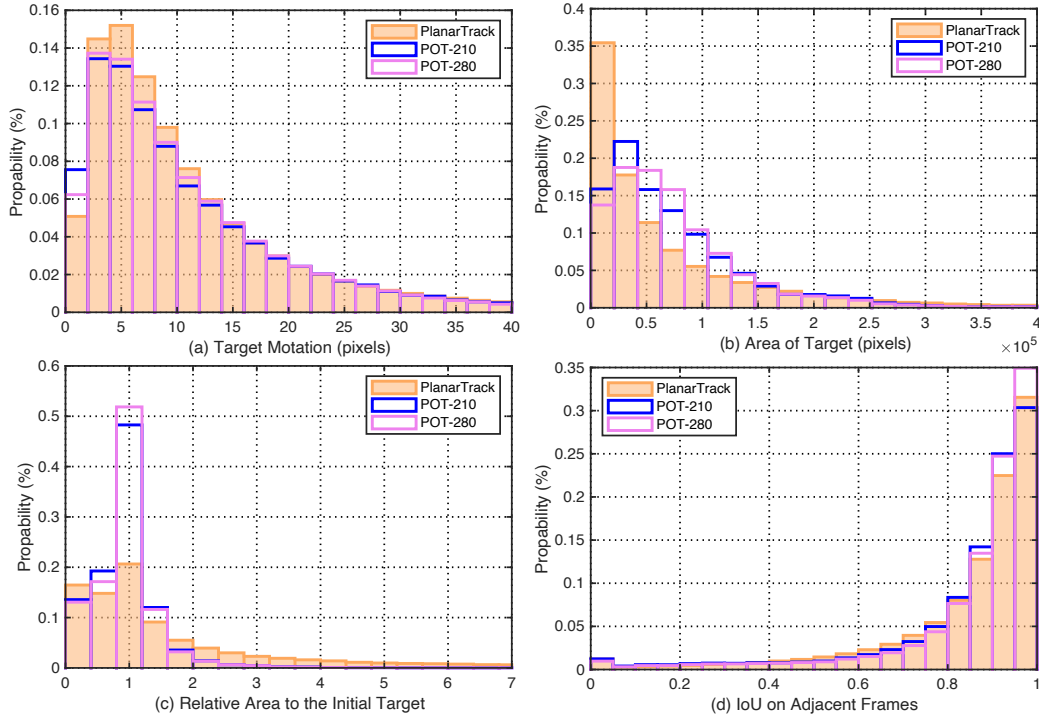
Figure 5: Statistics of planar target motion, size, relative area compared to initial object and IoU of targets in adjacent frames in PlanarTrack and comparison with the recent POT-210/280 (Liang et al., 2018, 2021). We can see the targets in our dataset have smaller sizes and faster and more challenging motions.
