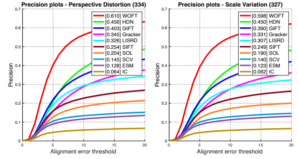
(a) Evaluation on the two most common challenging factors using precision.
