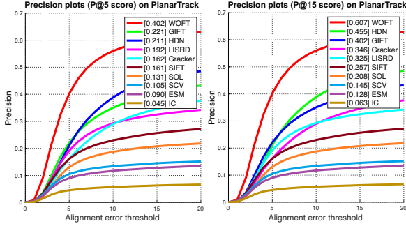
Figure 10: Precision plots of all planar trackers on PlanarTrack Tst using P@5 score and P@15 score, respectively.
