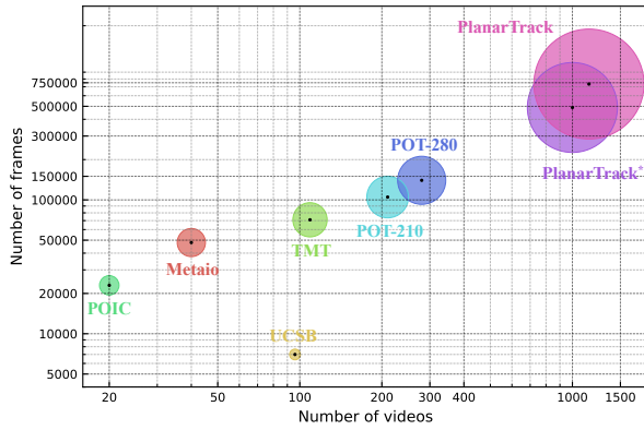
Figure 2: Summary of planar object tracking datasets, containing POT-280 (Liang et al., 2021), POT-210 (Liang et al., 2018), TMT (Roy et al., 2015), UCSB (Gauglitz et al., 2011), Metaio (Lieberknecht et al., 2009), POIC (Chen et al., 2017), our PlanarTrack and PlanarTrack* from conference version (Liu et al., 2023). The circle diameter is in proportion to the number of frames of a dataset. Our PlanarTrack is the largest benchmark.
