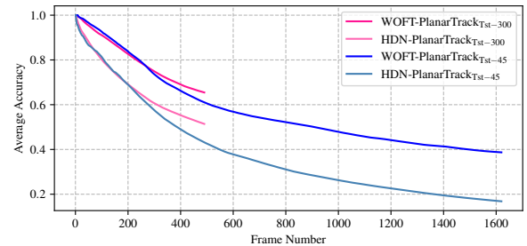
Figure 9: Accuracy changes of two planar trackers WOFT and HDN with respect to frame number.
