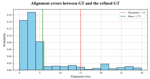
Figure 6: Distribution of alignment error between the GT and the refined GT of PlanarTrack.
