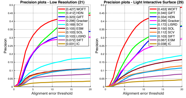
(b) Evaluation on the two most difficult challenging factors using precision.
