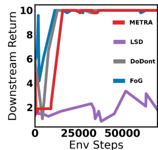
Figure 9: Downstream task performance.
