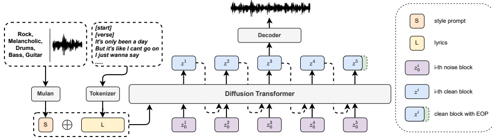
Figure 1: Overview architecture of our proposed DiffRhythm 2. Either text description or audio can specify the style prompt.
