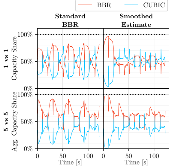
Figure 10: Evaluation of the BBR adaptation using a moving average of the minimum-RTT estimate ( \tau^{\min} ) with \theta = 1/6 ). As a result of the adaptation, the oscillation is successfully dampened.
