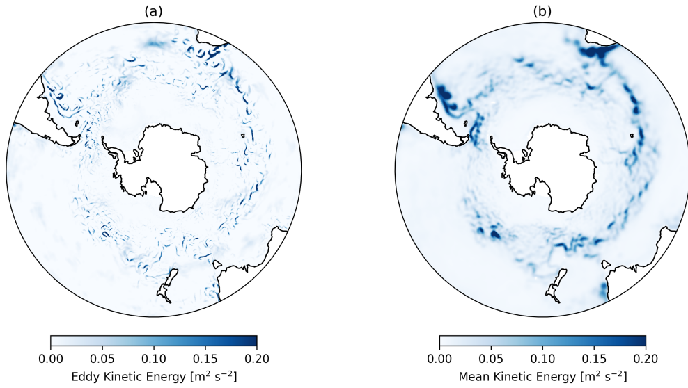
Figure S1: Results from a \frac{1}{4} -degree, 1-year simulation with a CNN-based parameterization of backscatter. (A) shows the resolved eddy kinetic energy on December 31 and (B) the mean kinetic energy (averaged over December). The Southern Ocean shown here is one of the regions where we expect a significant amount of energy to be exchanged between the eddy-field and the mean field.
