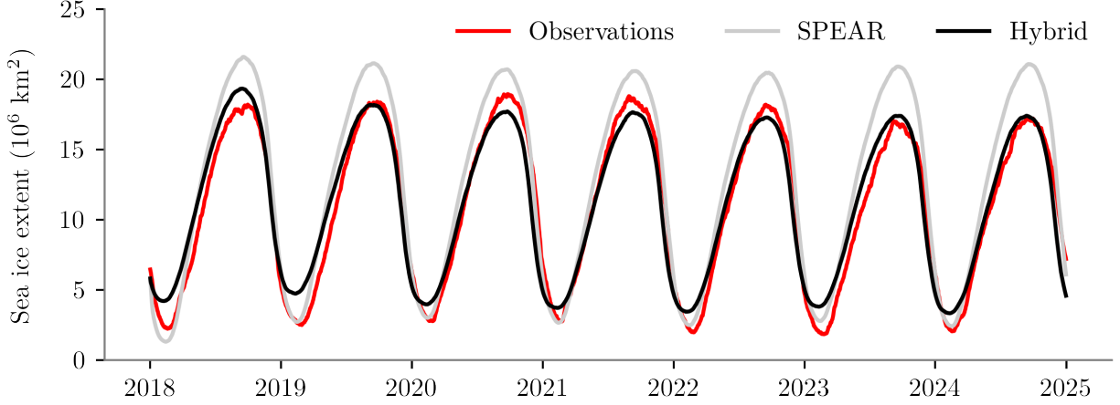
Figure 8: Pan-Antarctic sea ice extent from fully-coupled simulations. A 7-year continuous integration of the fully-coupled GFDL SPEAR climate model (gray) and an equivalent hybrid version of SPEAR (black) which performs online sea ice bias correction using ML.
