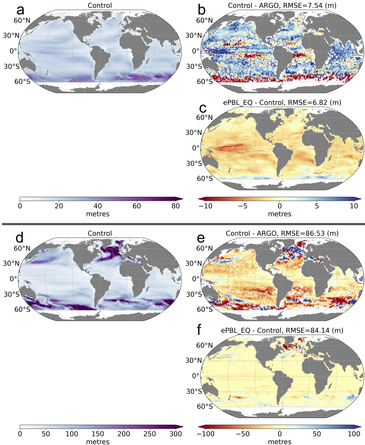
Figure 9: Mixed layer depths from fully-coupled SPEAR simulations. Summer MLD: (a) Summer MLD averaged over years 1970-2013 in SPEAR run that uses baseline ePBL scheme, (b) Bias in summer MLD between run with baseline ePBL and ARGO data, (c) Difference between ePBL with enhanced diffusivity (44) and baseline scheme showing the response of the enhancement. 28 Winter MLD: d-e-f are the same as in a-b-c , respectively, but for winter MLD.
