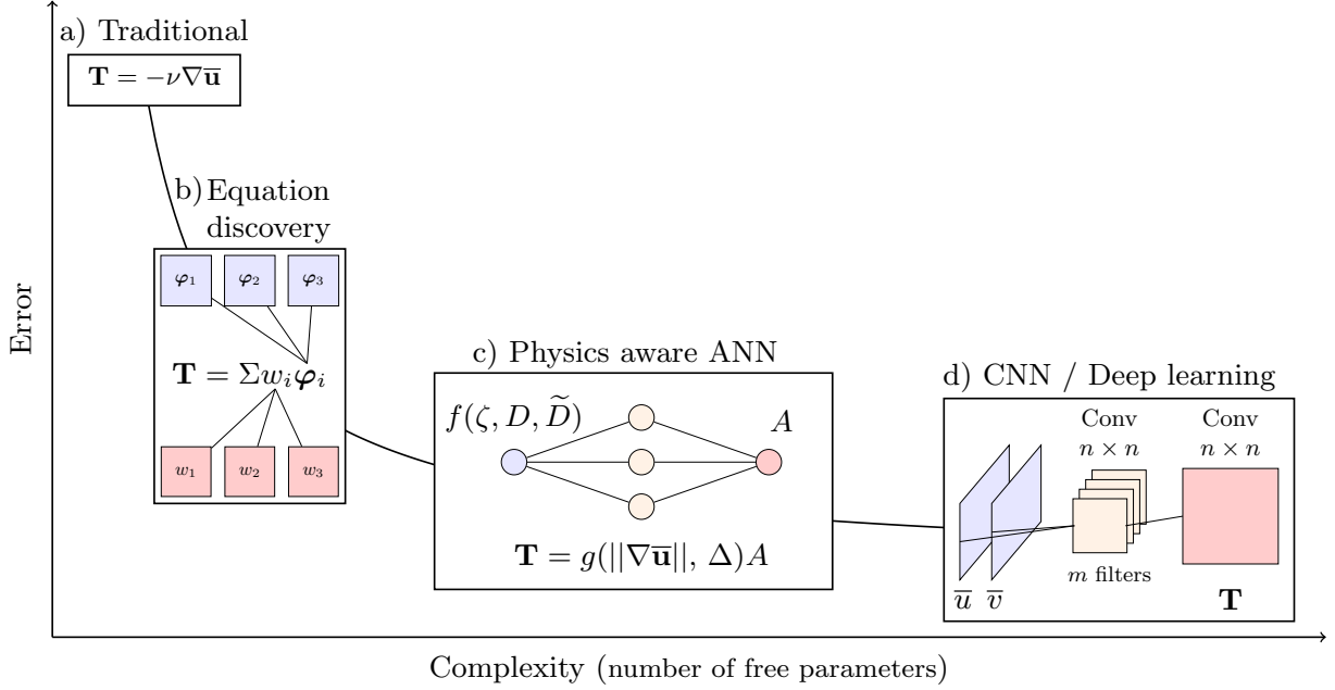
Figure 2: Schematic of Structural Error vs. Complexity. Panel a–d are organized on a structural error vs complexity curve, which generally transitions from high error and low complexity (e.g., small number of free parameters) to low error and high complexity. Here, each panel uses the case of parameterizing the momentum stress tensor ( \mathbf{T} ) in different ways as an example. Panel a) illustrates a more traditional approach to flux parameterization, where the stress tensor is simply a function of the velocity gradient, for anti-viscosity (30). Panel b) shows equation discovery methods, where the basis functions \boldsymbol{\varphi} may be chosen or discovered functions of the velocity field, such as vorticity \boldsymbol{\varphi}_1 = \boldsymbol{\zeta} = \nabla \times \bar{\mathbf{u}} , shearing deformation \boldsymbol{\varphi}_2 = \mathbf{D} = \partial_y \bar{u} + \partial_x \bar{v} , and the stretching deformation \boldsymbol{\varphi}_3 = \tilde{\mathbf{D}} = \partial_x \bar{u} - \partial_y \bar{v} (8, 32). Panel c) shows physics-aware ANNs, where as an example the inputs are also hand chosen (e.g., \boldsymbol{\zeta} , \mathbf{D} , \tilde{\mathbf{D}} ), and the outputs from the network are dimensionalized using some physics-informed function g of an appropriate norm of the input fields, \|\nabla \bar{\mathbf{u}}\| and the grid-spacing \Delta . Panel d) shows CNNs where the input fields are chosen to be some variables, e.g., filtered velocity fields, with minimal inductive bias.
