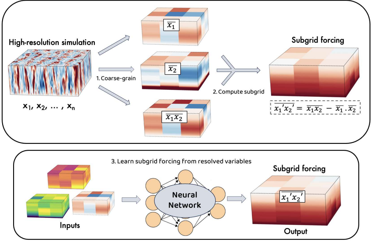
Figure 1: Schematic of learning subgrid processes from high-resolution simulation. Here, x_n represents the physical variables (e.g., velocities at a grid point) simulated by a high-resolution model. A coarse-graining procedure, which relies on spatial filtering, is applied to the high-resolution data to explicitly compute the subgrid forcing and input variables on a coarse-resolution mesh. The overbar represents a spatial average, and the prime represents the fluctuation from the mean. A neural network is then trained to predict the subgrid processes (e.g., \overline{x_1'x_2'} ) from coarse-resolution variables (e.g., \overline{x_1} ).
