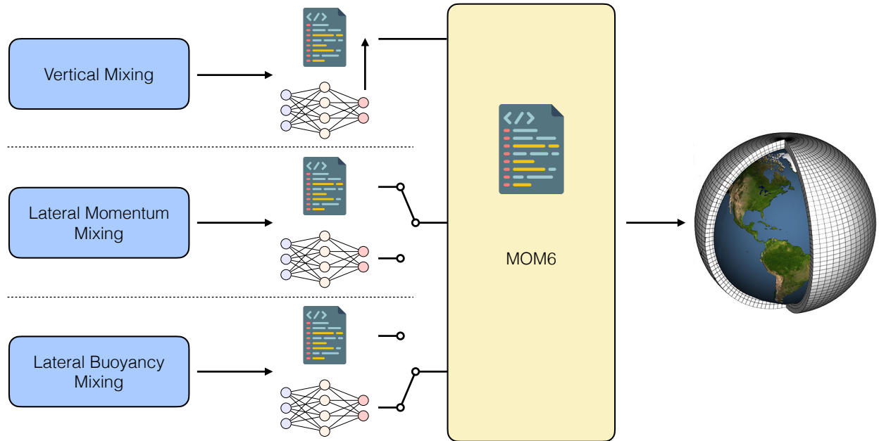
Figure 3: Schematic of an ANN module, written in Fortran, in MOM6 being used for multiple parameterizations within the GCM. The ANN module is created to perform the inference for multi-layer ANN models trained in PyTorch or other ML libraries. The weights, biases, and others parameters are stored in a NetCDF file, which communicate the information to the Fortran module. For ocean vertical mixing, the module computes the vertical profile of diffusivity, while for the lateral momentum mixing parametrization it computes the full eddy momentum flux.
