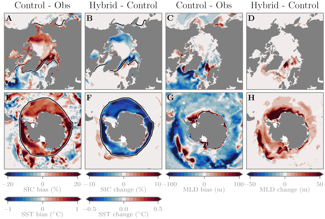
Figure 7: Changes in online ocean and sea ice biases from machine-learned sea ice bias correction. (A) Arctic sea ice concentration (SIC) and sea-surface temperature (SST) biases from a 5-year control simulation (2018–2022). The model’s climatological sea ice edge is shown by the black contour. Poleward of this contour are SIC biases, and equatorward are SST biases. (B) The change in SIC and SST due to ML-based sea ice bias correction. Note that the colorbar is half the magnitude of Panel A. (C) Mixed-layer depth (MLD) biases in the control simulation. (D) The change in MLD due to ML-based sea ice bias correction (positive values indicate a deeper mixed layer in the hybrid simulation). (E–H) Same as A–D but for Antarctic.
