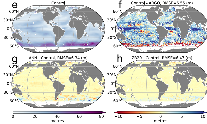
Figure 4: Summer Mixed Layer Depth (MLD) in meters: Changes induced by ML parameterizations for ePBL and lateral momentum fluxes. (A, E) Summer MLD, found using the potential anomaly criterion (47), in the control run for ePBL with JRA forcing and for mesoscale parameterization with CORE IAF, respectively; (B) Bias of control with respect to ARGO; (C) Difference between ePBL_NN and control; (D) Difference between ePBL_EQ and control; (F) Difference between ANN and control; (G) Difference between ZB20 and control.
