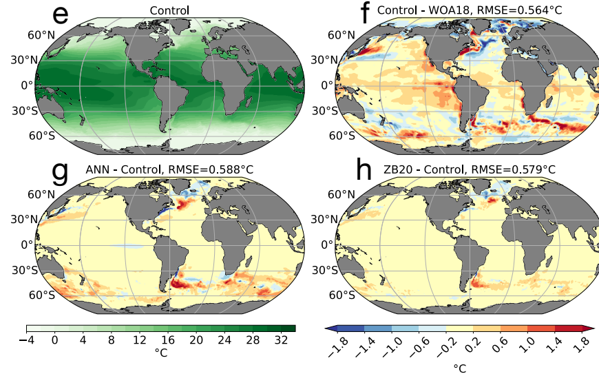
Figure 6: Annual Mean Sea Surface Temperatures in °C. Same captions as Fig. 4. Note again that the biases in SSTs under different forcings are shared by the models, except in the Tropics. The repeat forcing from IAF lead to larger biases in the ENSO region in particular, as expected
