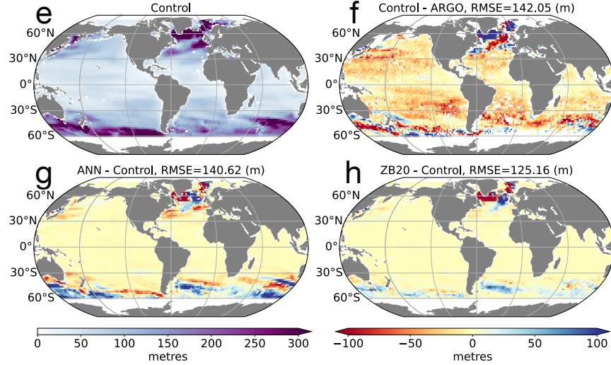
Figure 5: Winter Mixed Layer Depth: Changes induced by ML parameterizations for ePBL and lateral momentum fluxes. Panels are the same as Fig. 4 but for winter MLD. Note that control biases exhibit the same patterns under different forcing conditions (JRA vs. CORE IAF, but with varying magnitudes.
