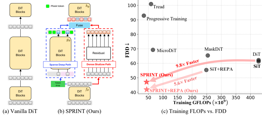
Figure 1: Sparse-dense residual fusion improves the efficiency of diffusion transformer training. SPRINT decouples the computationally heavy middle blocks of DiT into a sparse-deep path and a dense-shallow residual path. Notably, on ImageNet-1K 256 2 , SPRINT achieves up to 5.6× and 9.8× lower training cost compared to vanilla models, while improving generation quality.
