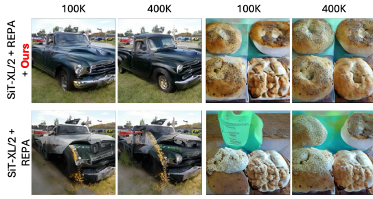
Figure 5: SPRINT improves visual scaling. Qualitative comparison of images generated without classifier-free guidance at 400K iterations using two SiT-XL/2 REPA models, with SPRINT applied to the model in the upper row.
