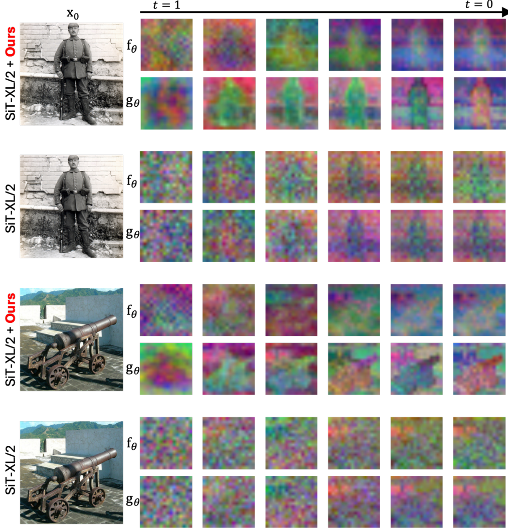
Figure 32: SPRINT improves feature semantics (additional examples) . We visualize PCA features of f_\theta and g_\theta from two SiT-XL/2 models at 400K iterations. The top rows show the model trained with SPRINT, while the bottom rows show the baseline. Compared to the baseline, features from SPRINT exhibit clearer semantic structure across both images.
