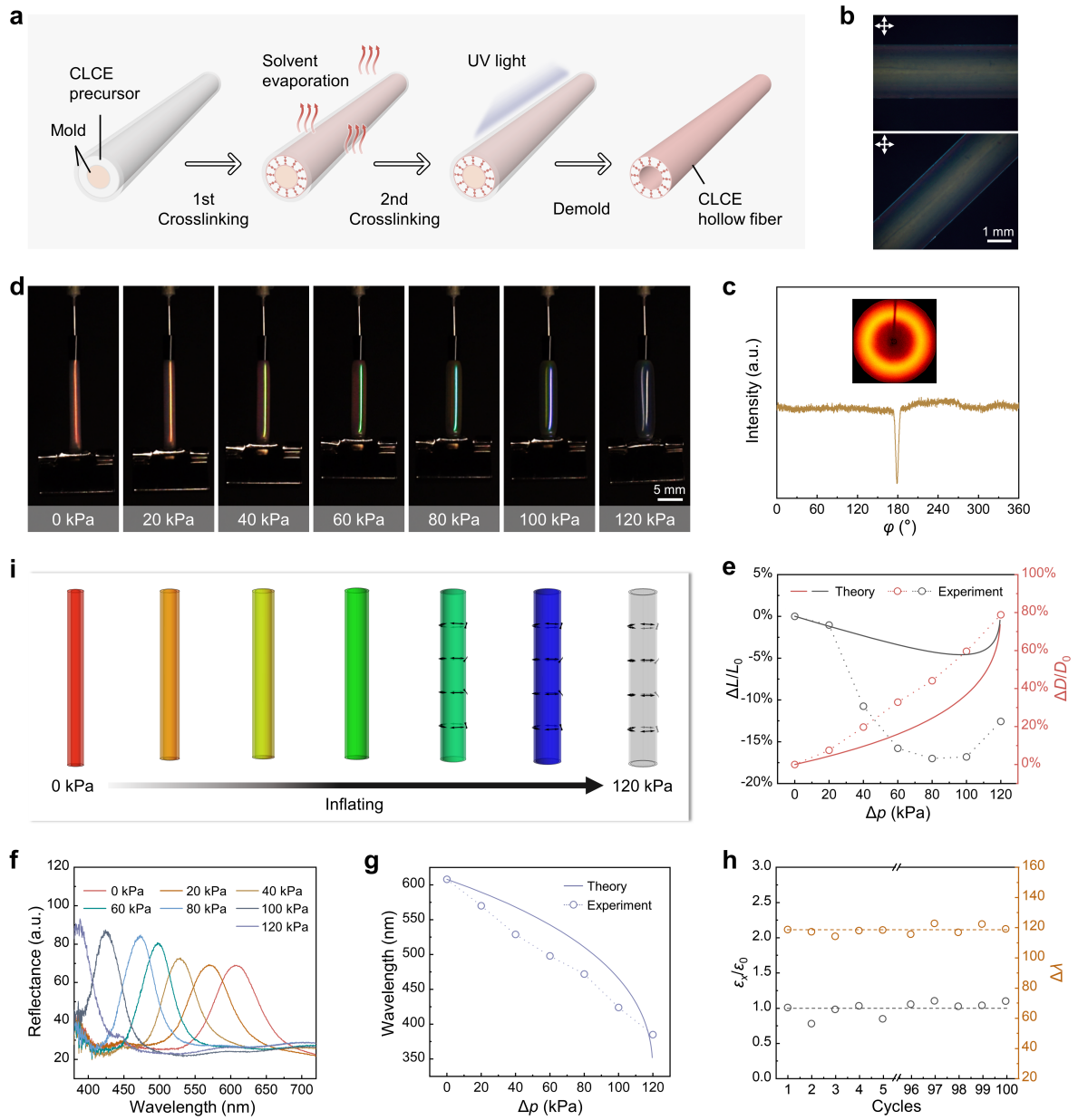
Figure 2. Characterization of pneumatic response performance of polydomain CLCE hollow fiber. a) Schematic of fabrication process for CLCE hollow fiber via an anisotropic deswelling-assisted template method. b) POM of polydomain CLCE hollow fiber viewed between crossed polarizers. The fiber-axes were aligned parallel to and at 45° to the polarizer, respectively. c) XRD pattern and intensity of azimuthal scan of polydomain CLCE hollow fiber. d) Images of a red polydomain CLCE hollow fiber inflated at different pressures. e) Axial and radial deformation ratios of the polydomain CLCE hollow fiber as a function of pressure. f) Reflectance spectra of the CLCE hollow fiber corresponding to (d). g) The reflection wavelength of the polydomain CLCE hollow fiber at different pressures. h) Cyclic performance
