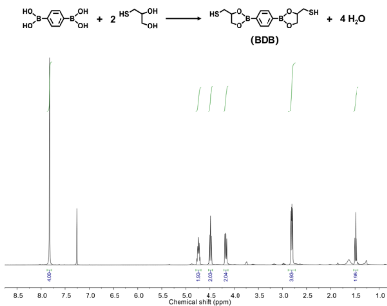
Figure S1. Reaction scheme and 1 H NMR spectrum of BDB.
