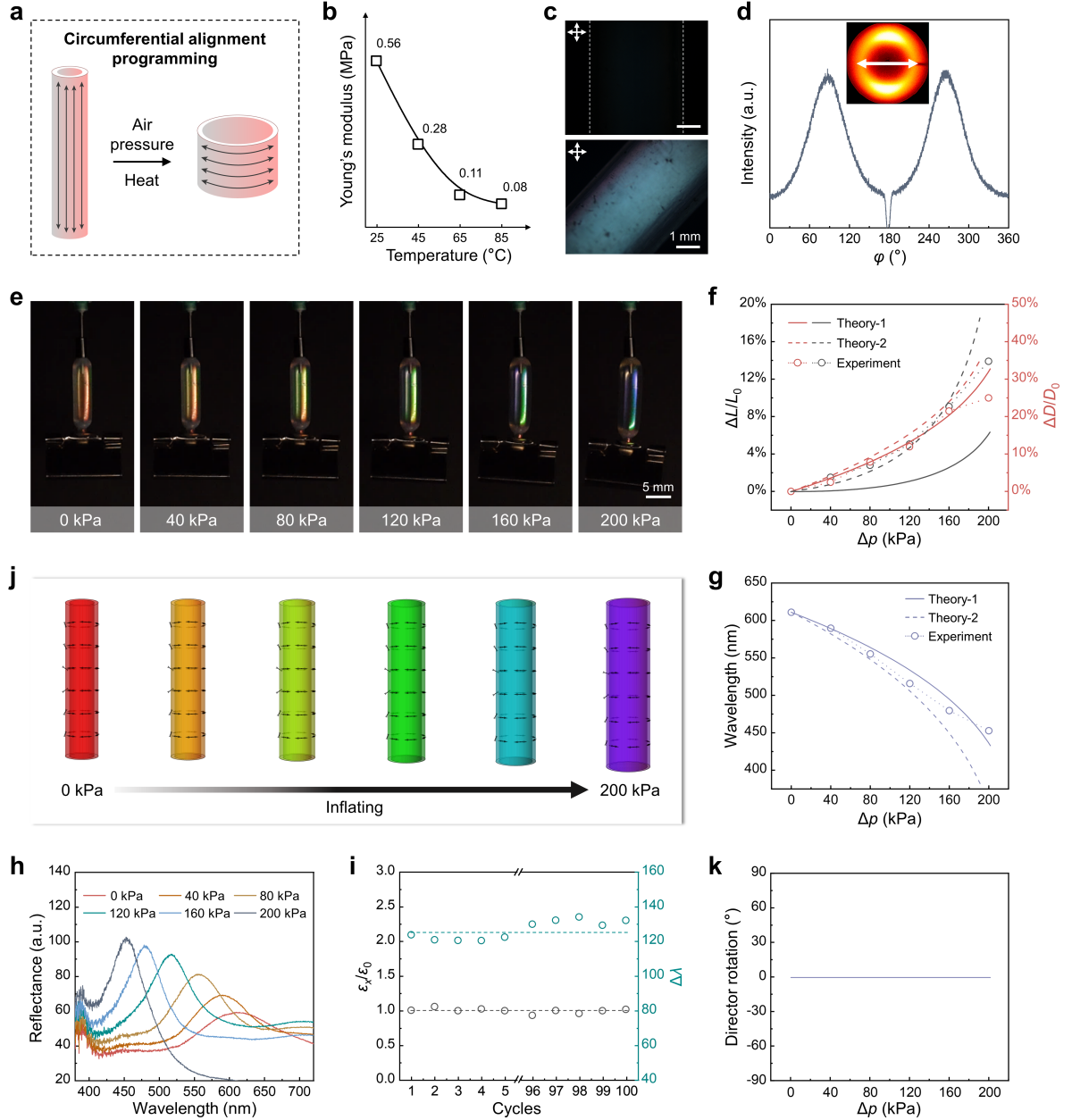
Figure 4. Characterization of pneumatic response performance of circumferentially aligned CLCE hollow fiber. a) Schematic diagram of the programming process for obtaining CLCE hollow fiber with circumferential alignment. b) The Young's modulus of the monodomain CLCEs at different temperatures. During the test, the load direction was perpendicular to the alignment. c) POM images of CLCE hollow fibers with circumferential alignment. d) XRD pattern and azimuthal scan intensity of the CLCE hollow fiber with circumferential alignment. e) Images of a red CLCE hollow fiber with circumferential alignment inflated at different pressures. f) Axial and radial deformation ratios of the CLCE hollow fiber with circumferential alignment as a function of pressure. g) The reflection
