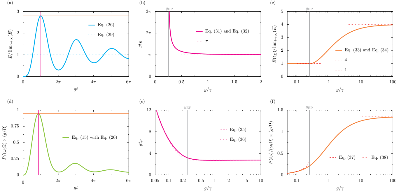
FIG. 2. Performance of the quantum battery with linear coupling. Panel (a): the energy E (cyan line) stored in the quantum battery, in units of the asymptotic result \lim_{t \rightarrow \infty}(E) , as a function of time t (in units of 1/g ) [cf. Eq. (26)]. Dotted line: the steady state energy [cf. Eq. (29)]. The instant in time (pink line) and specific energy (orange line) of the energetic maximum is marked. In this column we take the charger–battery coupling strength g = \gamma/2 , where \gamma is the decay rate of the charger. Panel (b): the optimal charging time t_E (pink line) in units of 1/g , as a function of the dimensionless ratio g/\gamma [cf. Eq. (31) and Eq. (32)]. Dotted line: the asymptote t_E = \pi/g of the dissipationless limit. Panel (c): the maximum energy E(t_E) (orange line) as a function of g/\gamma [cf. Eq. (33) and Eq. (34)]. Dashed line: the steady state result [cf. Eq. (29)]. Dotted line: in the dissipationless limit, the result is four times the steady state result [cf. Eq. (30) when t = \pi/g ]. Panel (d): the charging power P (green line) of the quantum battery, in units of \omega_b \Omega^2/g , as a function of time t [cf. Eq. (15) with Eq. (26)]. The instant in time (pink line) and specific power (orange line) of the power maximum is marked. Panel (e): the optimal time t_P (pink line) as a function of g/\gamma . Dashed line: the weak coupling limit [cf. Eq. (35)]. Dotted line: the strong coupling limit [cf. Eq. (36)]. Panel (f): the maximum power P(t_P) (orange line) as a function of g/\gamma . Dashed line: the weak coupling limit [cf. Eq. (37)]. Dotted line: the strong coupling limit [cf. Eq. (38)]. In this figure the vertical grey lines in panels (b, c, e, f) mark the location of the exceptional point g_{EP} [cf. Eq. (28)], and the energies E referred to in the top row of panels are exactly equivalent to ergotropies \mathcal{E} since the quantum battery is in a minimum uncertainty state [cf. Eq. (40)].
