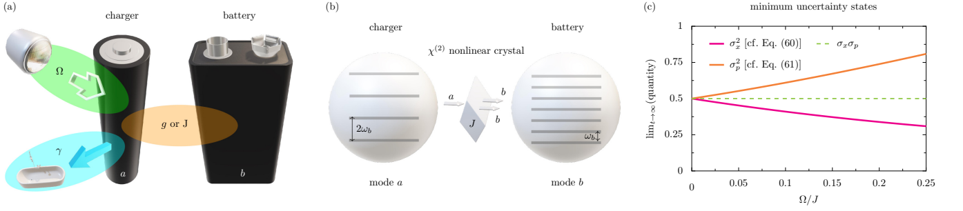
FIG. 1. The bosonic quantum battery as a driven-dissipative system. Panel (a): the general setup of the two-component quantum battery, complete with its charger and battery pieces (modes a and b ). The charger is driven by laser light with an amplitude \Omega (green region), and it suffers from dissipation at the rate \gamma into its surrounding heat bath (blue region). Two flavours of interaction (orange region) are considered: either (i) linear coupling (of strength g ) or (ii) nonlinear coupling (of strength J ). These couplings enable excitation transfer from the time t = 0 from the charger mode a into the battery mode b , where the energy is eventually stored in once the interaction is turned off at t = T . Panel (b): The nonlinear quantum battery is modelled as two quantum harmonic oscillators interacting via a nonlinear coupling of strength J , which is mediated by (for example) a \chi^{(2)} nonlinear crystal. The emission of one photon of frequency 2\omega_b from the charger (mode a ) leads to two photons of frequency \omega_b impinging on the battery (mode b ). Panel (c): the quadrature variances \sigma_x^2 and \sigma_p^2 in the steady state ( t \rightarrow \infty ) as a function of the dimensionless ratio \Omega/J for the nonlinear quantum battery [cf. Eq. (60) and Eq. (61)]. Dashed green line: guide for the eye at the minimum uncertainty.
