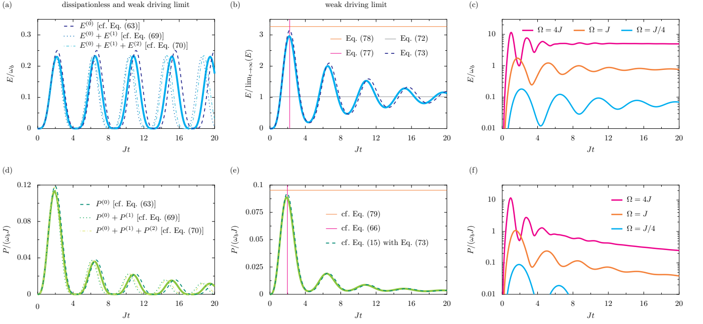
FIG. 3. Dynamics of the quantum battery with nonlinear coupling. Panel (a): the energy E stored in the quantum battery in the dissipationless limit (solid cyan line) and in units of the energy level spacing \omega_b , as a function of time t (in units of 1/J , the inverse of the coupling rate J ). Dashed, dotted and dash-dotted lines: three approximate results, derived with perturbation theory of increasing order [cf. Eq. (62)], along with Eq. (63), Eq. (69) and Eq. (70)]. Panel (b): the stored energy E (solid cyan line) in units of the steady state energy, within the weak driving regime \Omega \ll J . Dashed blue line: the approximate behaviour [cf. Eq. (73)]. Vertical pink line: the optimal charging time t_E [cf. Eq. (77)]. Horizontal orange line: the approximate maximum stored energy E(t_E) [cf. Eq. (78)]. Thin grey line: the approximate steady state energy \lim_{t \rightarrow \infty}(E) [cf. Eq. (72)]. Panel (c): a semi-logarithmic plot of the dynamic energy E in units of \omega_b . Panels (d, e, f): the charging power P of the quantum battery, in units of \omega_b J , corresponding to the stored energies of the above panels (a, b, c) respectively [cf. Eq. (15)]. In panel (e), the vertical pink line corresponds to the optimal charging time t_P [cf. Eq. (66)] and the horizontal orange line represents the maximum power P(t_P) [cf. Eq. (79)]. Within this figure, in the first two columns \Omega = J/4 and in the final two columns \gamma = J/2 .
