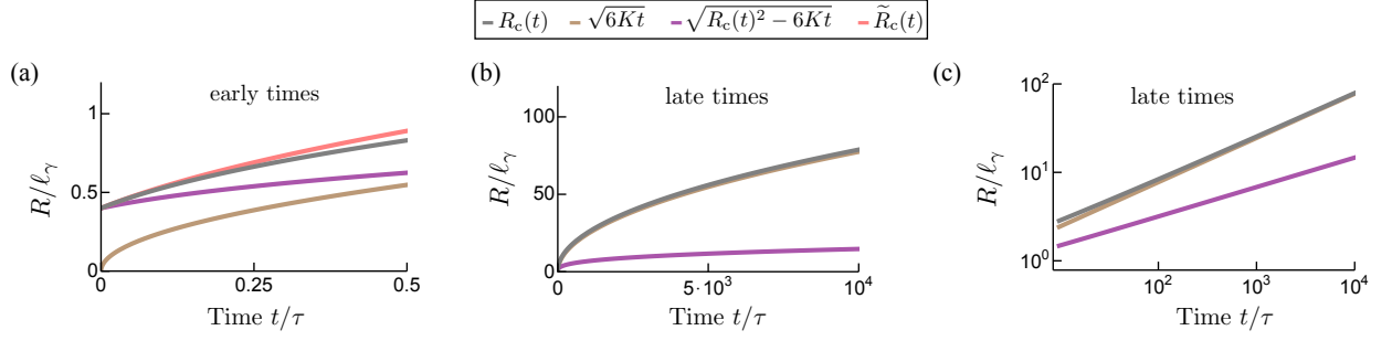
FIG. 9. Early and late time behavior of the critical radius. The solution R_c(t) , Eq. (45), is shown in gray, the leading order term \sqrt{6Kt} , which is also the t \rightarrow \infty approximation, Eq. (46), in brown, the t^{1/3} contribution, Eq. (D1), in purple, and the t \simeq 0 approximation \tilde{R}_c(t) , Eq. (D3), in pink. The chosen parameter values are consistent with the numerical simulation of emulsion kinetics, Fig. 6, with \Phi(0) = 0.1 , R_c(0)/\ell_\gamma = 0.4 , J\tau/c_{\text{in}}^{(0)} = 10^{-6} and K\tau/\ell_\gamma^2 = 10^{-4} , where \tau = \ell_\gamma/k . (a) At early times, \tilde{R}_c(t) successfully approximates the solution Eq. (45). (b) At late times, the solution converges to the leading order term approximation \sqrt{6Kt} (c) Log-log plot to visualize the long time asymptotic behaviour.
