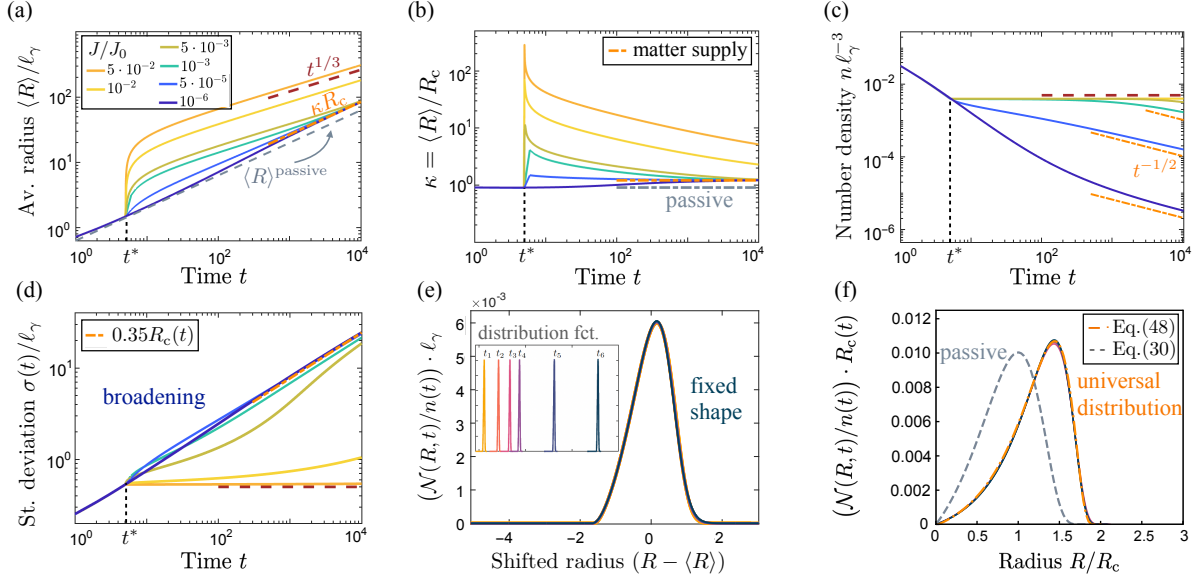
FIG. 6. Universal coarsening kinetics in an emulsion with constant matter supply in the interface-resistance-limited regime. (a) The average radius after an initial transient acceleration \propto t^{1/3} , converges to a new power law that is independent of the supply strength (orange dashed line, Eq. (50)). The supply is switched on at t^* , with time rescaled as t \rightarrow t/\tau , and \tau = \ell_\gamma^2/D^{\text{out}} . (b) The parameter \kappa converges to a constant value that is supply independent, \kappa \approx 1.19 . It is above the passive value \kappa = 8/9 (gray-dashed). (c) The droplet number density follows the power law \propto t^{-1/2} (orange dashed-dotted line). For a very high supply, the droplet number density is transiently constant (red dashed). (d) The standard deviation is increasing for all supply strengths. The droplet size distribution function stays transiently constant in shape in the interface-resistance-limited regime and converges at late times to the universal behavior Eq. (55) with R_c(t) in Eq. (46) (orange-dashed). (e) Droplet size distribution function \mathcal{N}(R, t)\ell_\gamma/n(t) at early times for a supply density such that droplet dissolution transiently ceases. Droplets in this regime are transiently decoupled, and the emulsion evolves with a constant standard deviation. The distribution function drifts in space with a fixed shape. The color code represents the different times at which the distributions were calculated, with yellow for early and blue for the late times. (f) Late time asymptotic behavior of the droplet size distribution function, when the average radius converges to Eq. (50). In the regime of broadening, the scaled droplet size distribution is universal, \mathcal{N}(R, t)R_c(t)d\rho/n(t) = h(\rho)\rho d\rho/4 . For the passive case (gray dashed), we use Eq. (30). The analytical solution matches the numerical time-series results. The solution for the passive case is indicated in the gray-dashed line. Results were obtained solving Eqs. (18), (23) for different values of constant matter supply density J , with the parameters given in Table III.
