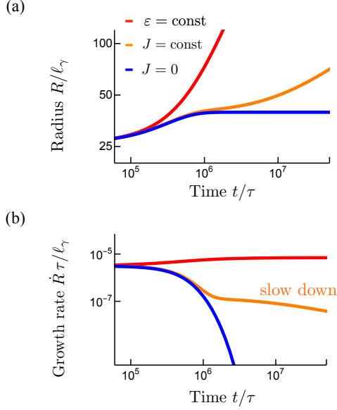
FIG. 8. Single droplet in a system coupled to a material reservoir. Results for the interface-resistance-limited regime. (a) Growth of the droplet for the three supply cases. In the presence of matter supply, the radius grows indefinitely, while in the passive case, the growth ceases close to equilibrium. \tau = \ell_\gamma/k in the log-log plot, \ell_\gamma denotes the capillary length. (b) Growth speed of the droplet radius R as a function of time in the log-log plot. For the constant supersaturation, the growth speed plateaus at a constant value. Results were obtained solving Eqs. (13b) for the interface-resistance-limited regime with the parameters given in Table I.
