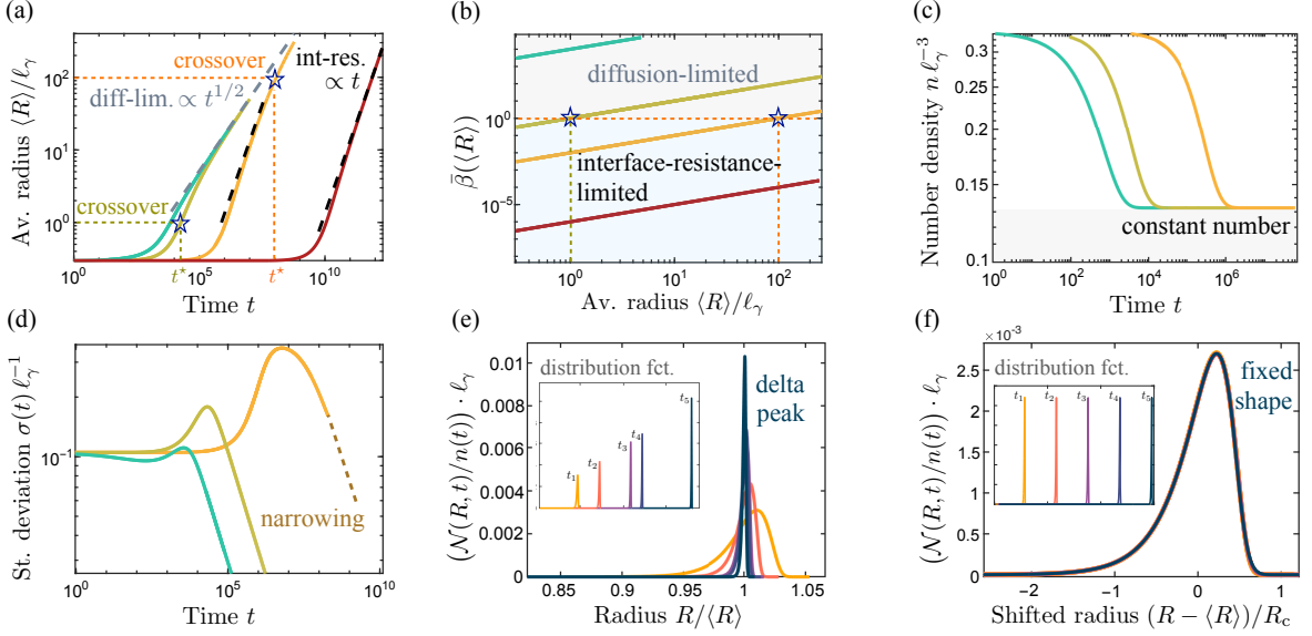
FIG. 4. Coarsening kinetics in an emulsion with constant supersaturation. (a) Average radius as a function of time t = t/\tau , \tau = \ell_\gamma^2/D^{\text{out}} . The solid lines correspond to different initial choices of \beta(\langle R(0) \rangle) . Depending on the initial choice, the growth of emulsion is determined by diffusion- or interface-resistance-limited transport, with the average radius following t^{1/2} or t power law, respectively. The star marks the crossover between the two regimes for a particular initial condition. (b) The crossover from the interface-resistance to diffusion-limited regime happens when \beta(\langle R \rangle) \geq 1 , indicated by the star. (c) After all droplets smaller than the critical radius have dissolved, the droplet number density saturates at a constant value. (d) After an initial regime of droplet dissolution, the standard deviation decreases. (e) In the diffusion-limited regime, the droplet size distribution function narrows towards a delta peak and is not universal. (f) In the interface-resistance-limited regime, the droplet size distribution drifts with increasing velocity in space, maintaining a fixed shape and a constant standard deviation. Results were obtained solving Eqs. (18), (32a) for constant supersaturation \varepsilon , with the parameters given in Table III.
