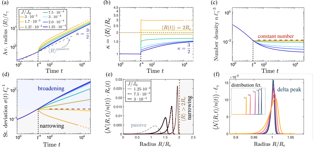
FIG. 5. Non-universal coarsening kinetics in an emulsion with constant matter supply in the diffusion-limited regime. (a) Average radius for different values of constant supply density J . The supply is switched on at t^* , with time rescaled as t \rightarrow t/\tau , and \tau = \ell_\gamma^2/D^{\text{out}} . (b) The average radius rescaled by the critical radius for different values of supply. The droplet size distribution function narrows for \kappa > 2 (red dashed line). For the supply such that \kappa < 3/2 , the coarsening converges to a broadening distribution function, for which \kappa relaxes to \kappa = 3/2 [35]. Since, in this limit, the asymptotic solution of the distribution function depends on the number density at the time the supply starts, we term it semi-universal. For \kappa > 3/2 , its value depends on the matter supply J/n(t^*) = 4\pi\ell_\gamma c^{(0)}D^{\text{out}}(\kappa - 1) . (c) Droplet number density converges to a constant value (red dashed line). (d) Standard deviation crosses from the broadening to the narrowing regime with the increasing supply density J . The color code for the supply strength is indicated in (a). (e) The droplet size distribution function collapsed for a supply in the broadening regime via rescaling of the spatial coordinate by the critical radius. The choice of supply strength corresponds to the broadening regime. The color code represents different times for measuring the distribution function, while the line style corresponds to the strength of the supply density. (f) The droplet size distribution function narrows towards a delta peak for a supply in the narrowing regime. The color code represents the measurement times, with yellow indicating early times and blue indicating late times. Results were obtained solving Eqs. (18), (23) for different values of constant matter supply density J , with the parameters given in Table III.
