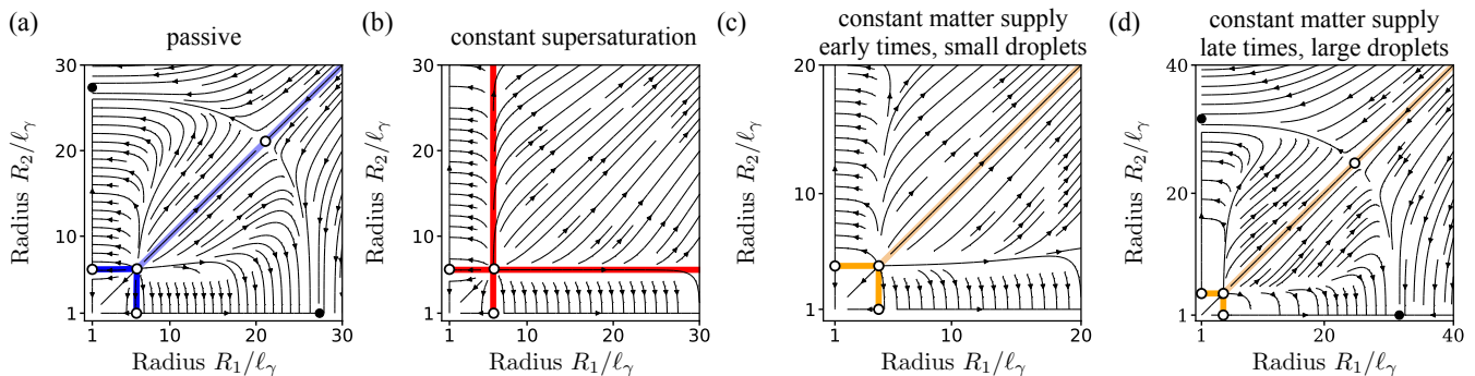
FIG. 3. Dynamics of two droplets in the diffusion-limited regime. Phase portrait of two droplets with radii (R_1, R_2) in the (a) passive, (b) constant supersaturation, and (c, d) the case with constant matter supply. Black lines and arrows indicate the flow field lines (\dot{R}_1, \dot{R}_2) , and colored solid lines the separatrices. A separatrix splits the phase portraits into domains that differ in the asymptotic behaviour at long times. Solid disks represent stable fixed points, and open circles are unstable fixed points. (a) In the passive case, there are three domains of dynamics. Droplets with radii smaller than the critical radius always shrink and dissolve, and there are two domains within which either R_1 or R_2 will not dissolve but reach the steady state. (b) For the constant supersaturation, there are three domains where one or both droplets shrink. The domain in the upper right corner describes the growth of both droplets. This growth is indefinite, and there is no stable fixed point. (c) At early times and for the constant supply, the dynamics are similar to those of the constant supersaturation. This similarity arises because droplet material is in excess, and the small droplets grow initially indefinitely. (d) At a late time and for the constant supply, the dynamics are similar to the passive case since droplets grew to large sizes where the constant matter supply is growth-limiting. As a result, there are two stable fixed points and a single droplet persisting over large times. Results were obtained solving Eqs. (14b), (15) for the diffusion-limited regime with the parameters given in Table II.
