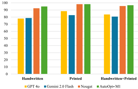
Figure 4: BLUE Score
