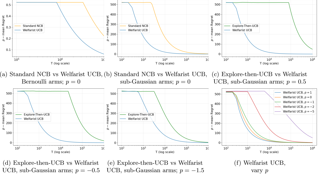
Figure 1: Numerical results for Welfarist UCB. (a) illustrates the comparison between the Nash regret ( p = 0 ) from Welfarist UCB and Standard NCB for Bernoulli rewards. (b) shows that Welfarist UCB achieves Standard NCB under sub-Gaussian rewards. (c), (d) and (e) show that Welfarist UCB outperforms Explore-Then-UCB for the general p -mean regret in all three regimes. (f) shows the ablation on p ; as p decreases, we get more fairness, but the regret also increases.
