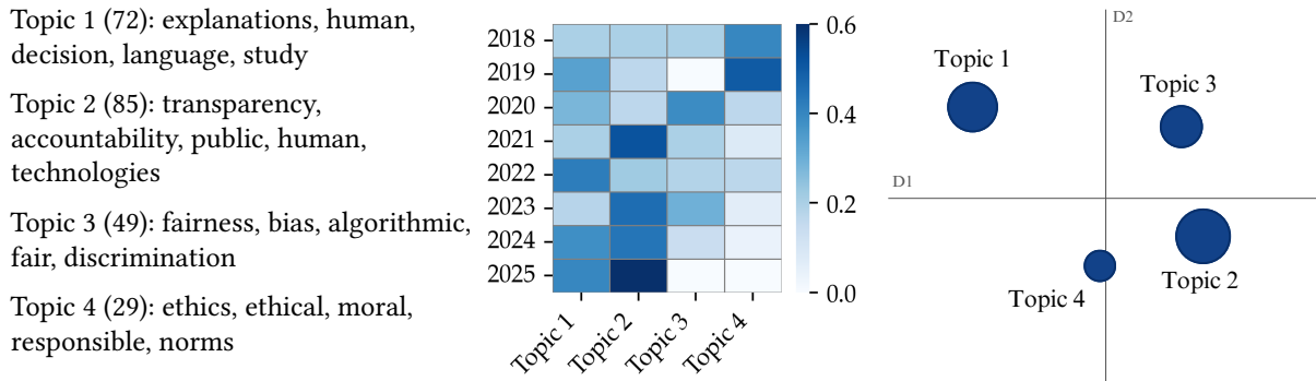
Fig. 3. Visualizations of topics generated using BERTopic applied to the initial keyword-based selection of articles ( N = 235 ). First, the heatmap (left) shows normalized topic distributions, grouped by year. Values refer to the proportion of documents associated with the topic. Second, the intertopic distance plot (right) shows the relative positions of topics in a 2D space. 3
