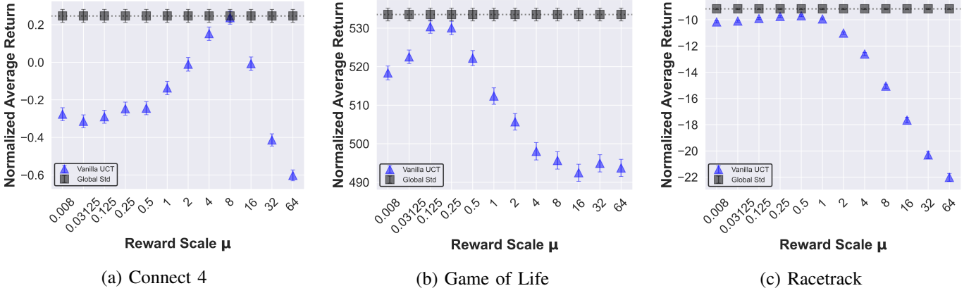
Fig. 4: Global Std is invariant to the reward scale of the environment, and scaling an environment’s reward function by \mu is equivalent to dividing the exploration constant by \mu in Vanilla UCT. Using this fact, the hypothetical performances of Global Std and Vanilla UCT for 500 iterations are shown for three different environments when their respective reward function is scaled by a constant \mu . To better compare performances, if the reward function is scaled by \mu , then the average return is divided by \mu . For all environments, the value C = 8 was used for Vanilla UCT, and for Global Std, the best performing C value for the non-scaled environment (i.e., \mu = 1 ) was used. Note that by construction, Global Std is invariant to the reward scale, while any fixed exploration constant, as in Vanilla UCT, is highly scale dependent.
