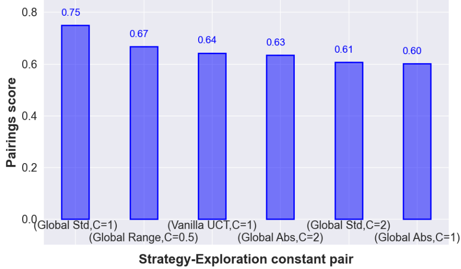
Fig. 6: The best 6 normalized pairings score for all considered \lambda -strategy and exploration constant C pairs. The score was constructed by considering all iteration budgets and all two-player games . One of our methods, Global Std with C = 1 , performs best overall, showing that Global Std even yields a small performance boost over Vanilla UCT in a constant reward scale setting.
