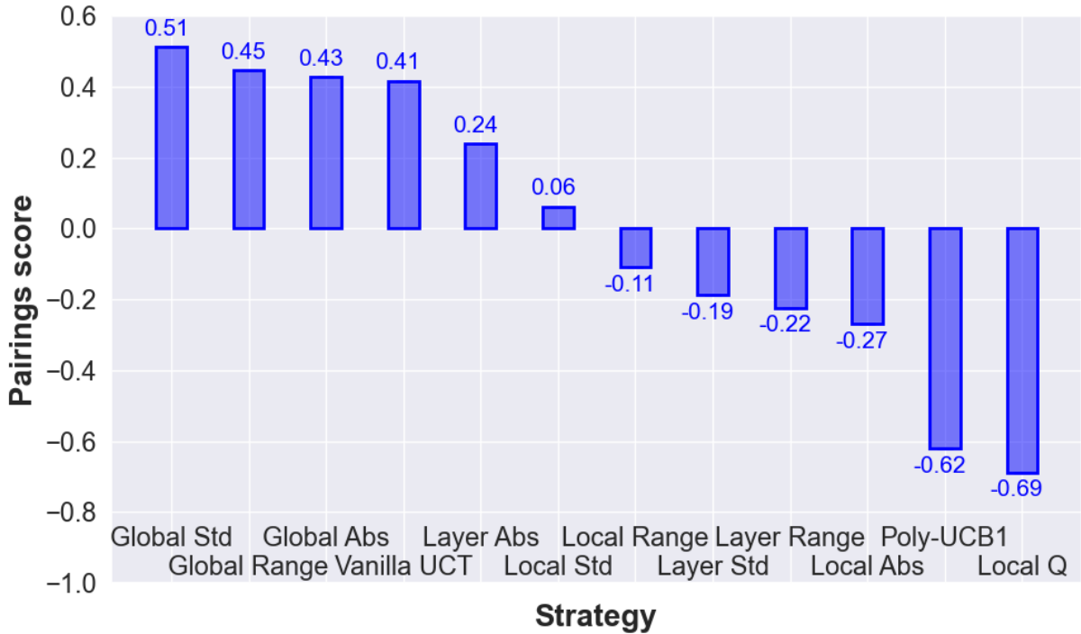
Fig. 5: The normalized pairings score for all considered \lambda -strategies. The score was constructed by considering all iteration budgets and all two-player games . Per pairing, the maximum performance over all C values (i.e. \{0.125, 0.25, 0.5, 1, 2, 4, 8, 16, 32, 64\} for all strategies and additionally 256 and 1000 for Vanilla UCT) was used per iteration-environment pair. One of our methods, Global Std, performs best overall.
