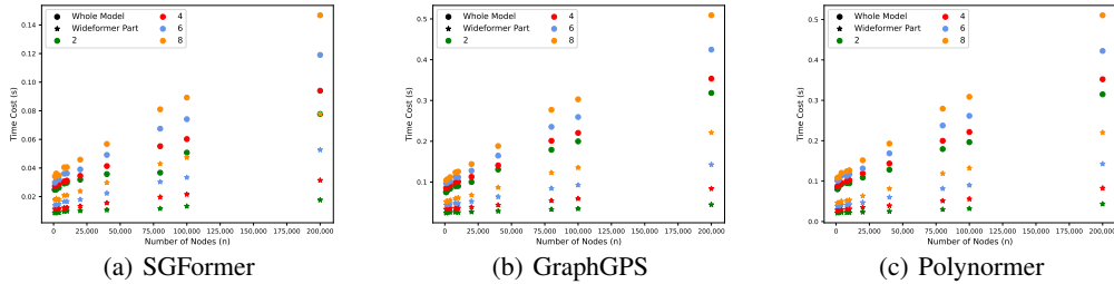
Figure S9: Time Cost. Different colors of the points denote the number of clusters m . The point shape “•” denotes the whole model with Wideformer. “*” denotes the Wideformer part.
