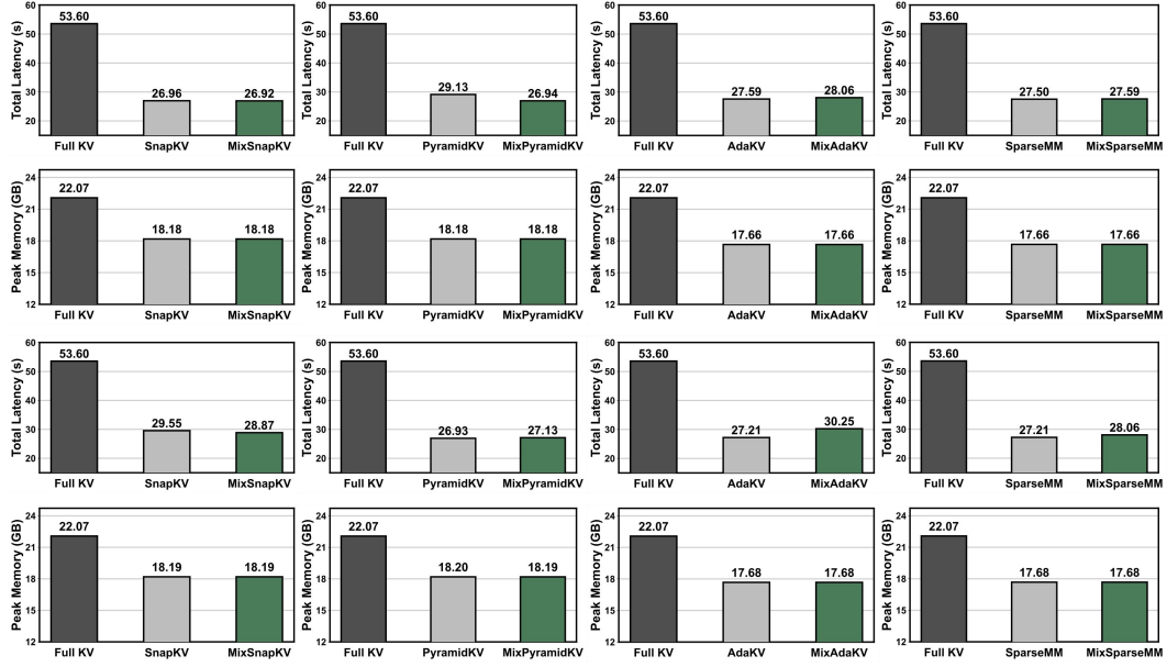
Figure 5: More efficiency comparisons of total latency and peak memory. The top two rows of bars correspond to a budget of 128, while the bottom two rows correspond to a budget of 256.
