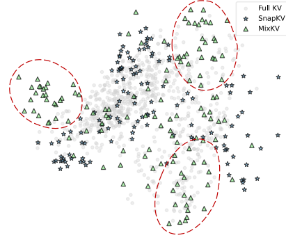
Figure 3: t-SNE visualization of KV cache distributions under different settings. “Full KV” represents the original KV distribution of Qwen2-VL without compression, serving as the reference distribution.
