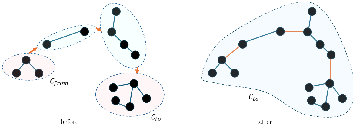
Figure 2: Merging C_{from} into C_{to} . The newly added edges (in orange) are given the rank r of the merge
