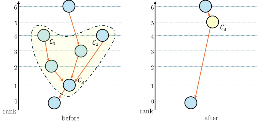
Figure 3: Tree pruning: Components C_1 and C_2 have the same rank 4, their least common ancestor is C_3 . All components with ancestor C_3 and rank at most 4 get merged together and the resulting component has rank 5. The orange edges inside the new component get added to T(C_3) with rank 5.
