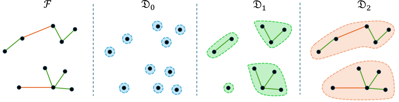
Figure 4: Component decompositions for a given set of requests and edges. Green edges have rank 1 while orange edges have rank 2.
