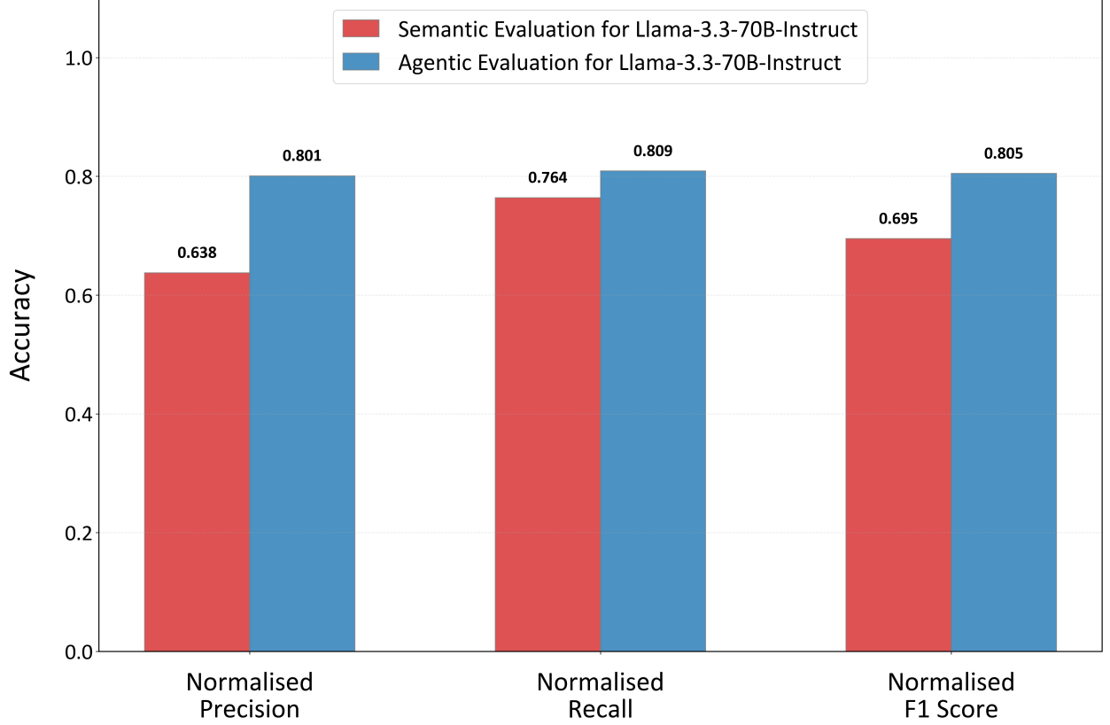
Figure 3: Normalised classification metrics (Precision, Recall, and F1-score) for model Llama-3.3-70B-Instruct (best performing model considering only normalised metrics) to showcase the performance of ComProScanner’s performance capability for the considered models using: semantic evaluation through the PhysBERT model (red bars), and agentic evaluation through the Gemini-2.5-Pro reasoning model (blue bars).
