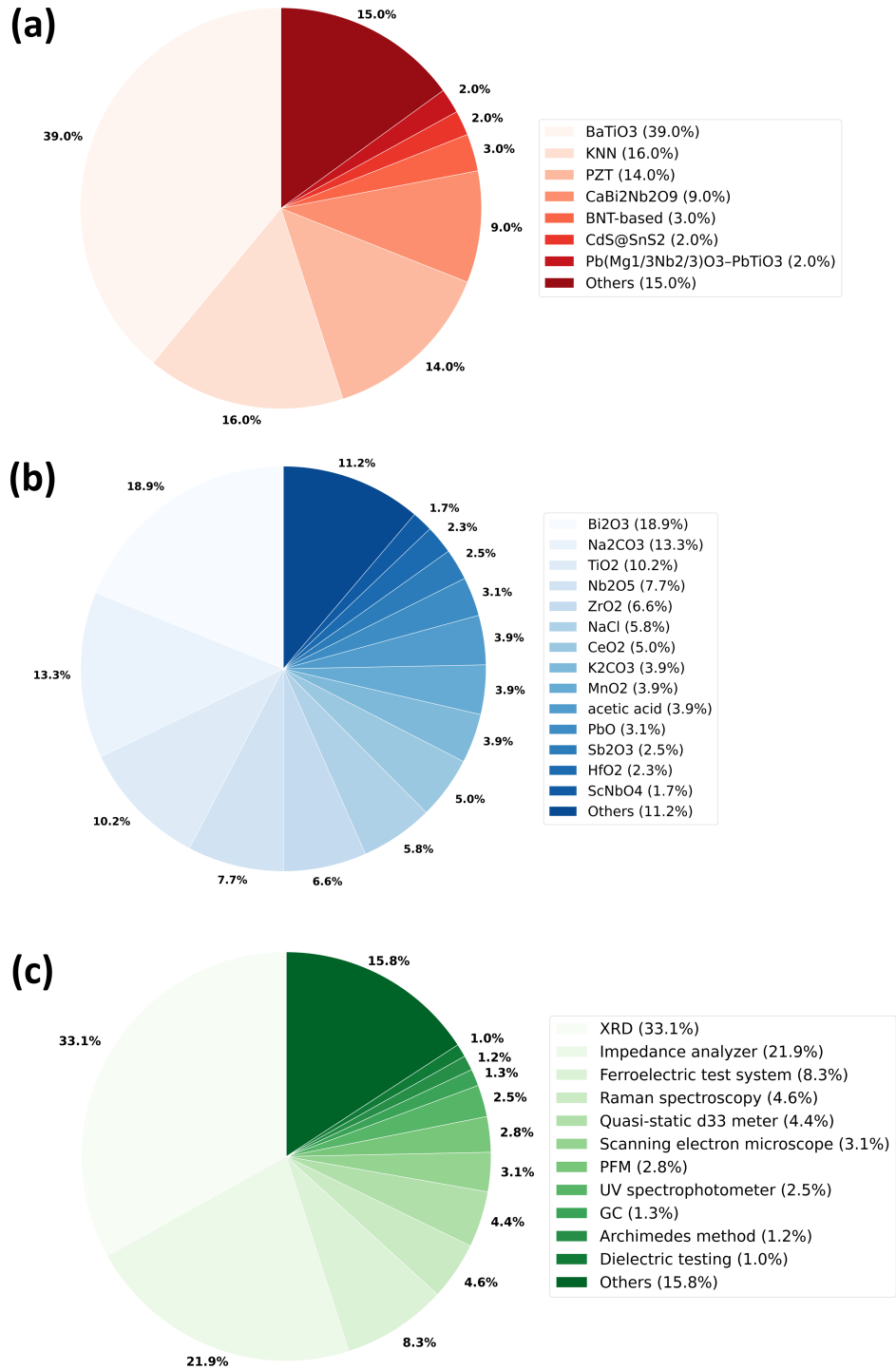
Figure 5: Distribution of various data types across the evaluated 100 articles: (a) piezoelectric material families, (b) synthesis precursors, and (c) characterisation techniques. Similarity thresholds of 0.8 were applied for families and precursors, whilst 0.78 was used for characterisation techniques to group semantically similar items.
