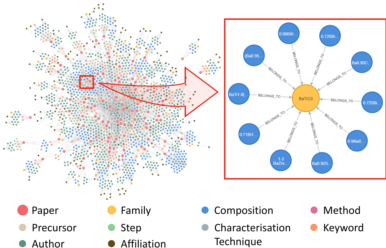
Figure 6: Generated neo4j knowledge graph from both composition-property, and synthesis data as well as metadata information extracted from 100 articles using the ComProScanner package. The inset shows 10 randomly chosen items from the 79 compositions associated with \text{BaTiO}_3 family node using cypher query.
