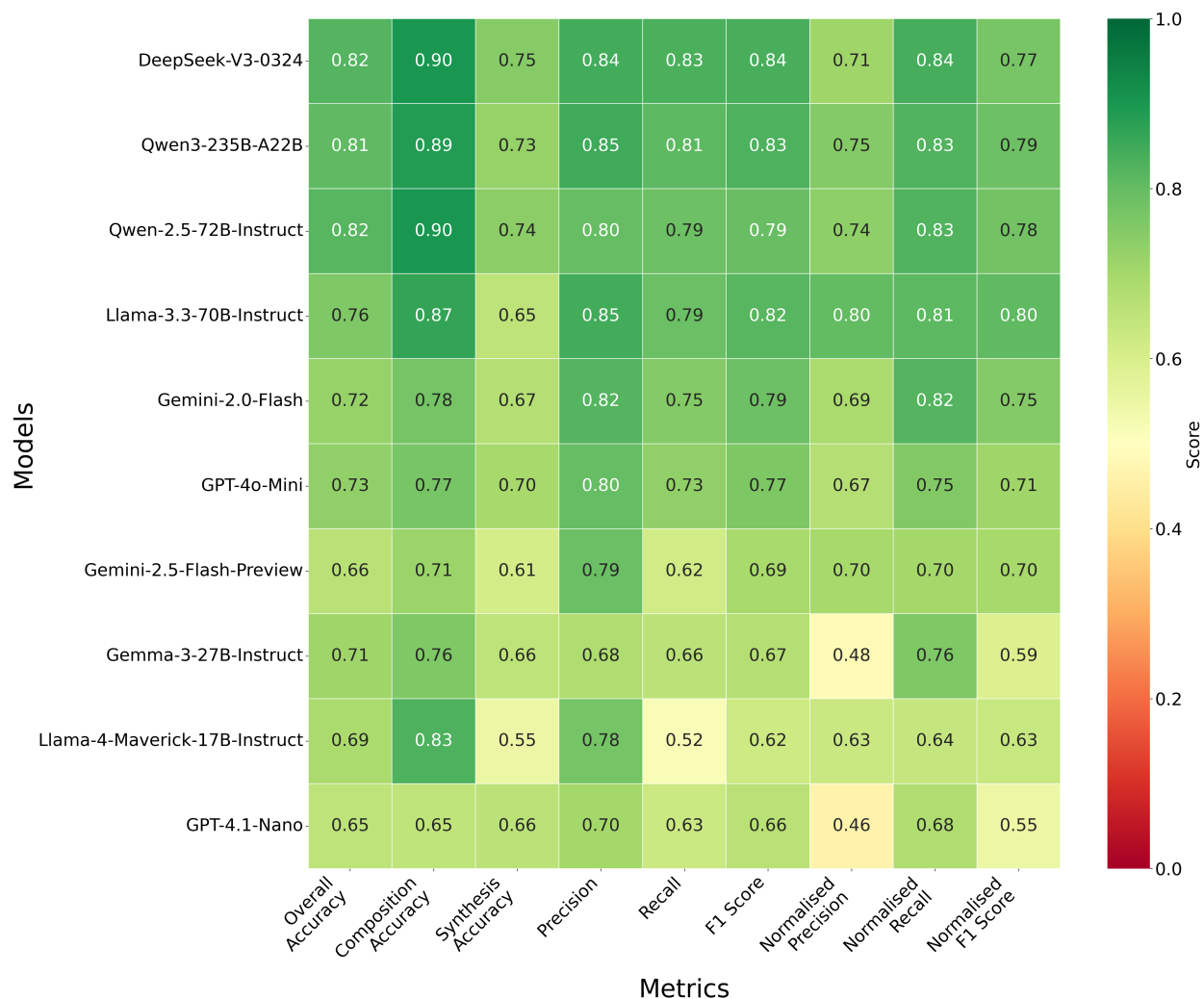
Figure 4: Confusion matrix from agentic evaluation, showcasing all 9 evaluation parameters, such as weight-based overall accuracy (average of composition accuracy and synthesis accuracy), weight-based composition accuracy and weight-based synthesis accuracy, classification metrics (Precision, Recall, and F1-score), and normalised classification metrics (normalised Precision, normalised Recall, and normalised F1-score), across 10 different LLMs used in this study.
