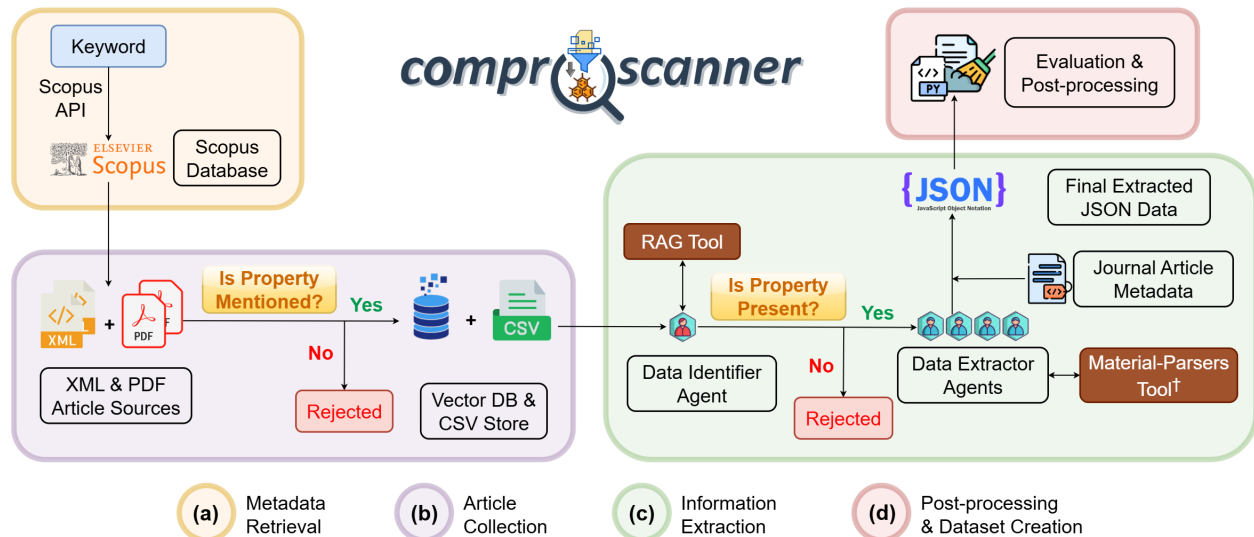
Figure 1: Overall workflow diagram of ComProScanner framework, separated in four distinct operational phases, distinguished with four different colour regions: (a) metadata retrieval (yellow), (b) article collection (purple), (c) information extraction (green), and (d) evaluation, post-processing, and dataset creation (brown).
