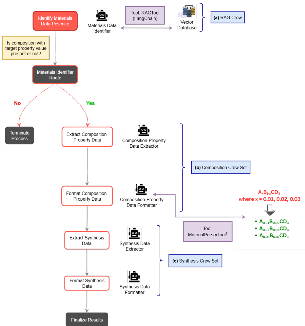
Figure 2: Comprehensive workflow diagram of the CrewAI-based extraction system in ComProScanner, comprising five specialised agents. The process begins with a property identifier agent ((a) RAG Crew) that leverages Retrieval-Augmented Generation (RAG) technology to filter relevant articles. The remaining four agents are strategically organised into two parallel functional subgroups: one dedicated to composition data extraction ((b) Composition Crew Set) and the other focused on synthesis information collection ((c) Synthesis Crew Set). Each subgroup implements a sequential two-agent architecture—the first agent extracts raw data while the second performs formatting and standardisation. The workflow integrates two essential tools: RAGTool for discriminating between mere property mentions and actual quantitative property values, and MaterialParserTool for accurate processing of complex chemical formulations.
