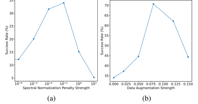
Fig. 7: Ablation on piece assembly task Effect of various (a) spectral normalization penalty strength parameters \lambda and (b) data augmentation threshold parameters T on the piece assembly task. Spectral normalization is applied assuming no data augmentation, while data augmentation ablations are done using the optimal level of spectral normalization \lambda = 0.1
