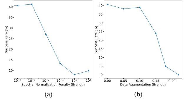
Fig. 8: Ablation on mug cleanup task Effect of various (a) spectral normalization penalty strength parameters \lambda and (b) data augmentation threshold parameters T on the mug cleanup task. Spectral normalization is applied assuming no data augmentation, while data augmentation ablations are done using the optimal level of spectral normalization \lambda = 0.001
