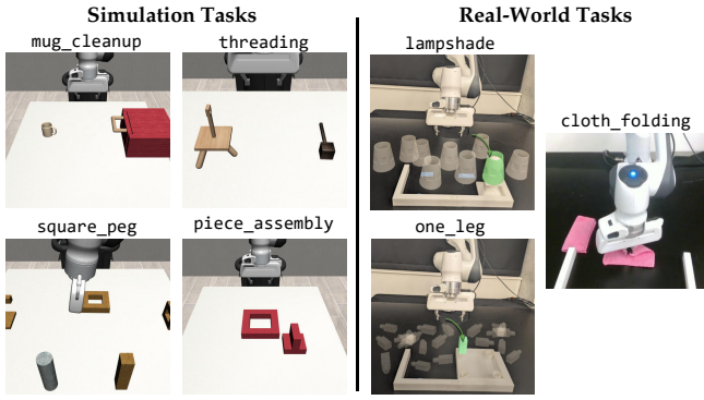
Fig. 4: Depiction of tasks in sim and the real world.
