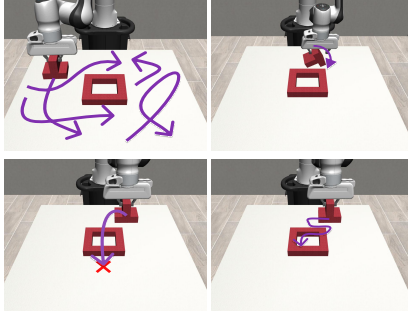
Fig. 9: Visualizations of types of play data for the piece-assembly task. (top left) high coverage play data — the block is randomly picked up and moved around the table (top right) partial tipping — the block is tipped over to its upright position (bottom left) failure — the block is attempted to be inserted, but misses (bottom right) suboptimal — the block is inserted into the hole, but in an inefficient manner
