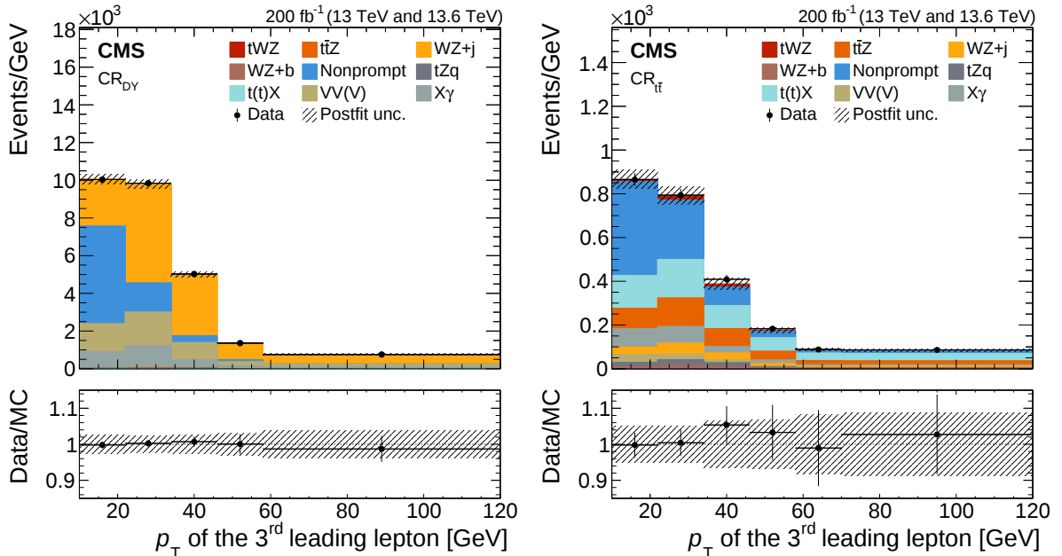
Figure A.1: Distribution in the p_T of the 3 rd leading lepton for the \text{CR}_{\text{DY}} (left) and \text{CR}_{\text{tt}} (right) after a fit to data. The dashed band shows the postfit uncertainty. The results from fits to 13 and 13.6 TeV data are combined for illustration purposes. The ratio of data to the predictions from MC simulations is shown below the distributions.
