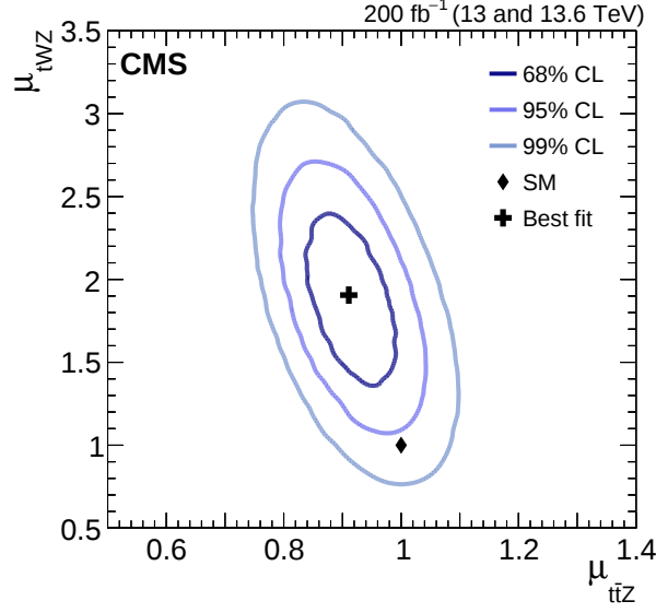
Figure 3: Likelihood scan of the signal strengths for tWZ and t\bar{t}Z production. The black cross shows the best fit value, while the black diamond indicates the SM expected value. The contours in different shades of blue correspond to the 68, 95, and 99% confidence level.
