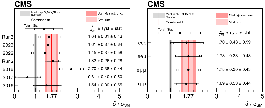
Figure A.2: Values of the signal strengths for tWZ production obtained from the different data-taking periods (left), and from events with different lepton flavors (right): three electrons ( eee ), two electrons and one muon ( ee\mu ), one electron and two muons ( e\mu\mu ), and three muons ( \mu\mu\mu ). If there are more than three leptons in an event, the three p_T -leading leptons are used to determine the flavor. The combined results from 13 TeV data (Run 2) and from 13.6 TeV data (Run 3) are also shown. The result from the combined fit to 13 and 13.6 TeV data is shown as a red line with the corresponding uncertainty shown as a red band. The SM prediction is shown as a gray band.
