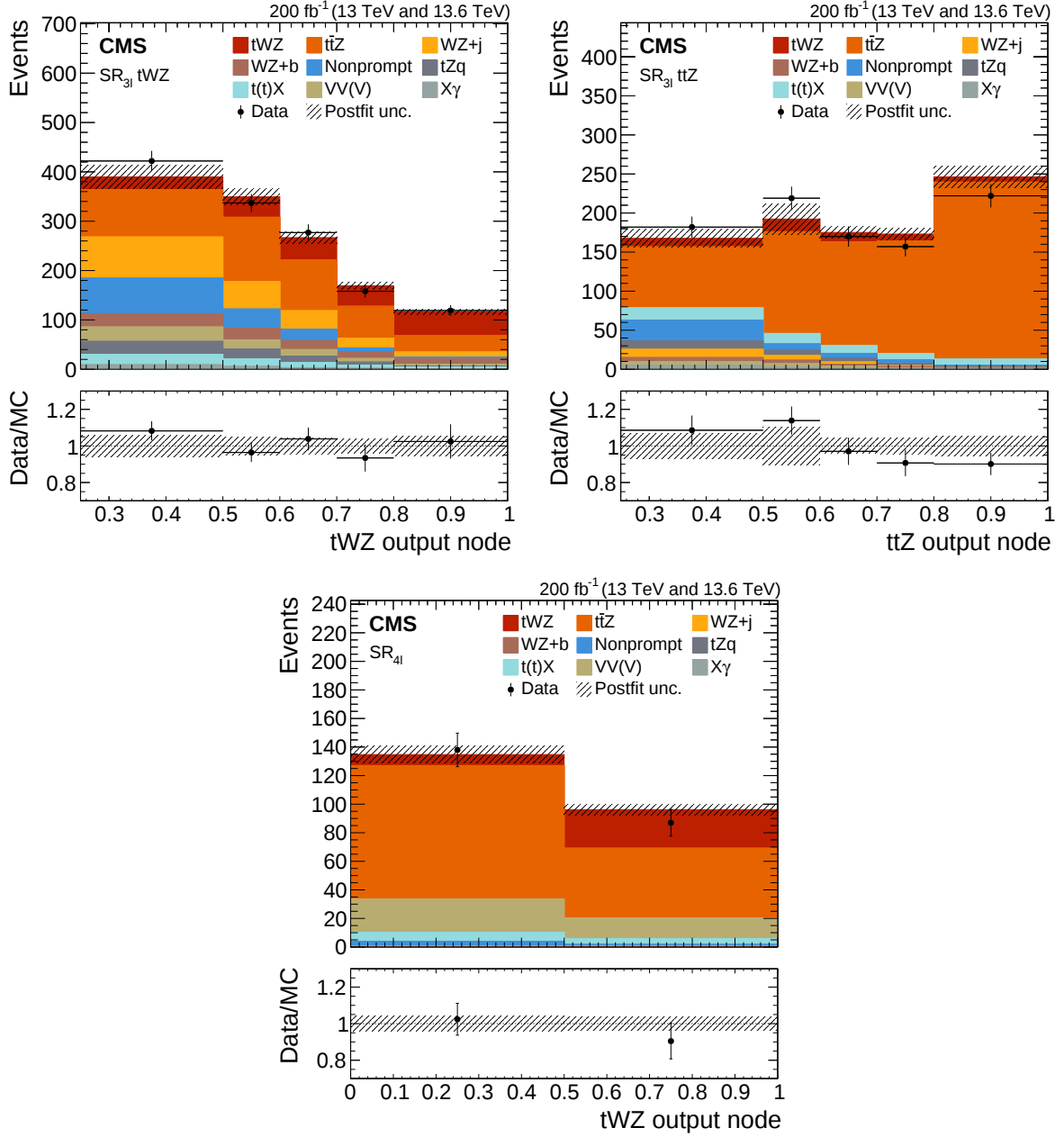
Figure 2: Distributions in the classifier output nodes for the tWZ (upper left) and t\bar{t}Z (upper right) nodes in SR_{3\ell} , and in the classifier output node in SR_{4\ell} (lower) after a fit to the data. The dashed band shows the postfit uncertainty. The results from fits to 13 and 13.6 TeV data are combined for illustration purposes. The ratio of data to the predictions from MC simulation is shown below the distributions.
