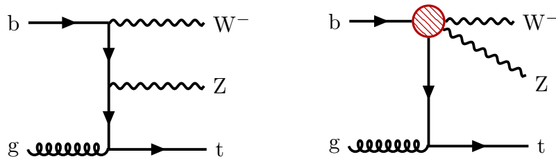
Figure 1: Example Feynman diagrams for tWZ production in the SM (left) and for anomalous tWZ production through an effective interaction (right). Charge conjugate versions of these diagrams are implied.
