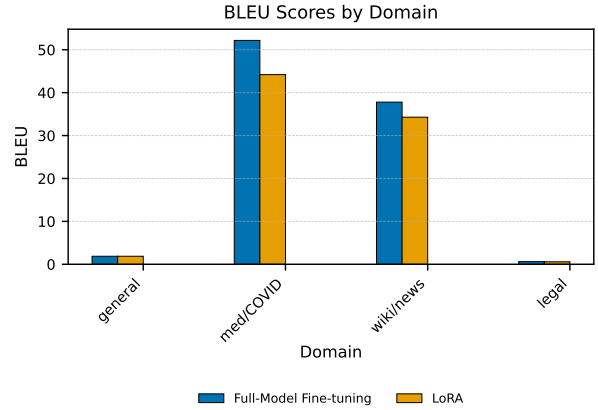
Figure 4: BLEU scores by domain comparing full-model fine-tuning and LoRA-based models on the domain-by-dataset split.
