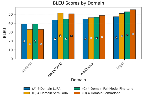
Figure 3: BLEU scores by domain comparing full-model fine-tuning and LoRA-based models trained on four domains.
