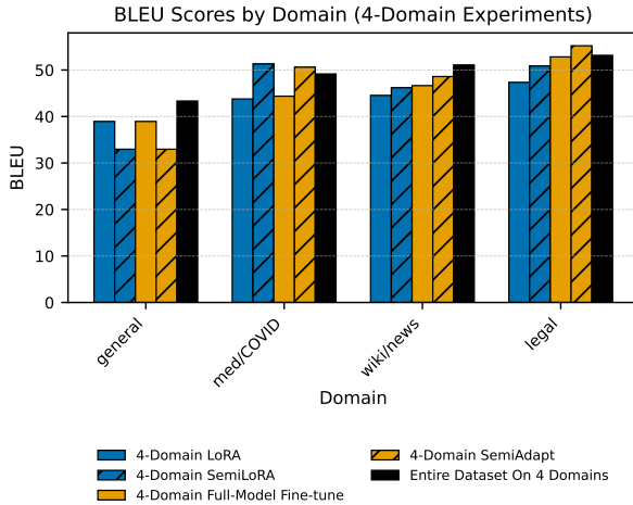
Figure 5: BLEU scores by domain comparing full-dataset fine-tuning, full-model domain fine-tuning, and LoRA-based models on the four-domain split.
