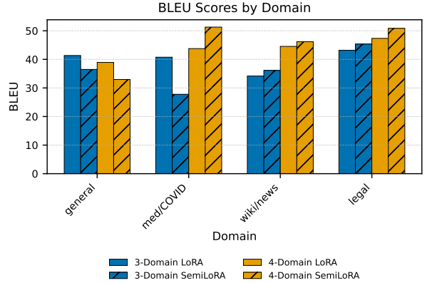
Figure 1: Comparison of BLEU scores by domain for LoRA and SemiLoRA models trained on three and four domains.
