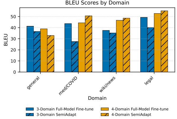
Figure 2: BLEU scores by domain comparing full-model fine-tuning and SemiAdapt models trained on three and four domains.
