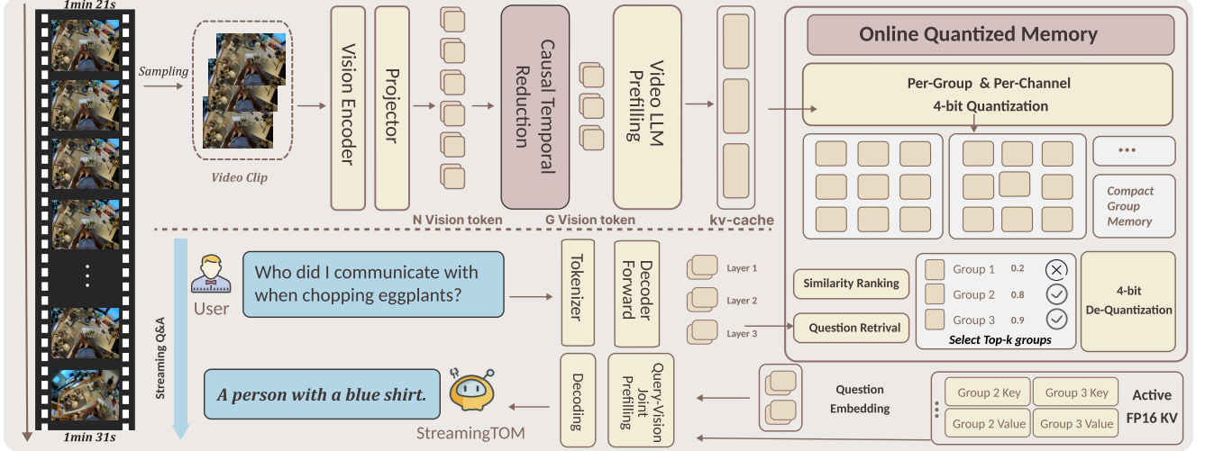
Figure 2. Overview of the StreamingTOM architecture. The framework consists of two coordinated pipelines. The vision pipeline encodes each frame and applies Causal Temporal Reduction to condense redundant tokens into compact groups, which are written to an online memory for reuse. The query pipeline processes questions and drives the decoder to interact with the memory through Online Quantized Memory, which stores groups at 4-bit precision, retrieves at most k groups on demand, and dequantizes them for efficient generation.
