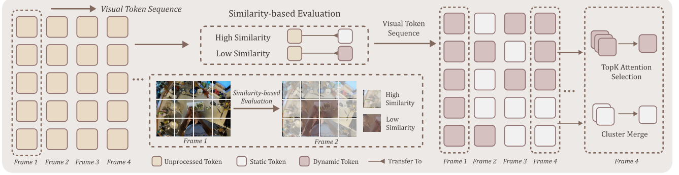
Figure 3. Overview of the CTR compression pipeline. The algorithm processes visual tokens from consecutive frames using a 2-frame window (current and previous), producing a binary classification (static, dynamic) through similarity comparison. The adaptive budget allocation dynamically distributes compression resources based on content, followed by dual-path processing: dpc clustering for static tokens and attention-based selection for dynamic tokens.
