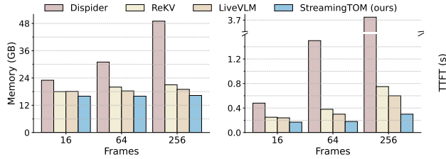
Figure 6. Memory and TTFT comparison across frame budgets. StreamingTOM outperforms all baselines in both metrics.
