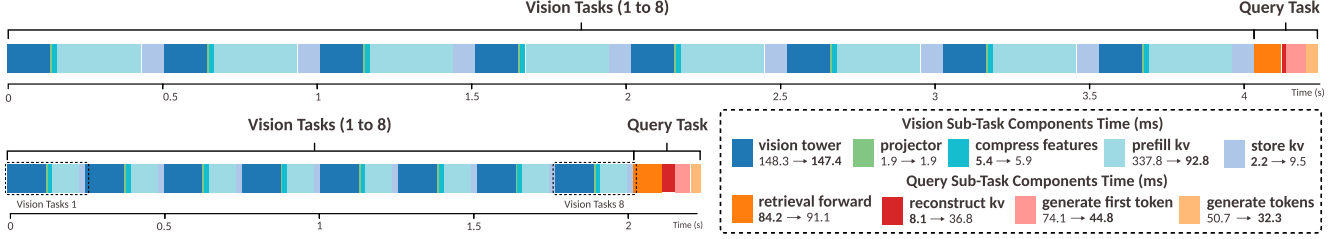
Figure 5. Complete processing timeline comparison. The top row shows the baseline, while the bottom row shows StreamingTOM. For a 64-frame stream at batch size 8 with 50 tokens per frame, StreamingTOM incurs minimal overhead: OQM introduces 7.3ms for kv storage, 6.9ms for retrieval, and 28.7ms for 4-bit reconstruction. In contrast, CTR delivers 3.6 \times prefill acceleration from 337.8ms to 92.8ms, yielding an efficient 0.20s query TTFT and demonstrating substantial performance gains at negligible cost.
