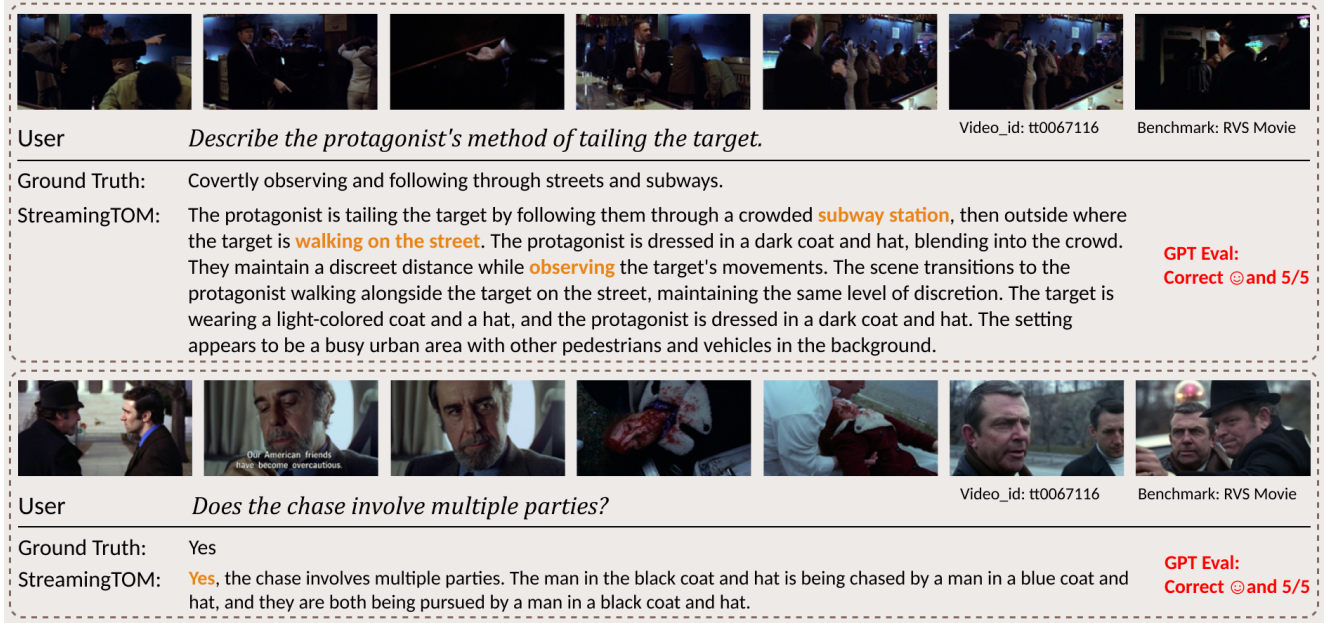
Figure 4. Two qualitative examples from RVS Movie requiring long-horizon reasoning. StreamingTOM provides faithful answers consistent with ground truth, accurately capturing fine-grained semantics such as “subway station” and multi-party interactions. These results illustrate the model’s ability to maintain causal reasoning and long-horizon consistency in real streaming scenarios.
