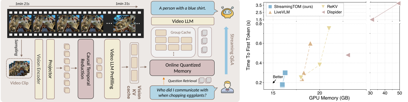
Figure 1. Left: StreamingTOM (streaming token compression) is a training-free, two-stage framework for efficient streaming video understanding: Causal Temporal Reduction selects pre-LLM tokens with a causal, fixed-budget policy, and Online Quantized Memory maintains compact kv-cache via 4-bit quantization with on-demand retrieval. Right: on LLaVA-OV-7B, StreamingTOM achieves a 15.7\times kv-cache compression ratio; compared to prior SOTA (LiveVLM), it delivers 1.2\times lower peak memory and 2\times faster TTFT.
