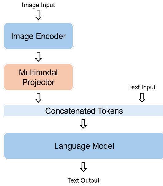
Figure 7: Structure of Multimodal LM. Multimodal projector aligns the visual and textual embedding space and reduces the number of image tokens.
