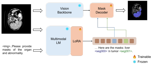
Figure 2: Architecture of RadDiagSeg-M . Our model supports multi-target flexible segmentation.
