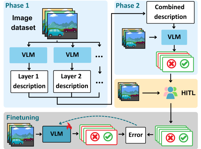
Fig. 1. Overview of the SAVANT framework. Driving images are processed in two phases: (1) Scene Description Extraction, where a VLM generates textual descriptions of scene layers (street, infrastructure, movable objects, environmental); (2) Scene Evaluation, where the original image and aggregated descriptions are jointly analyzed for anomaly classification. The resulting classifications undergo human verification and correction through Human-in-the-Loop (HITL) curation to create a high-quality training dataset, which is subsequently used to fine-tune an enhanced VLM capable of single-shot anomaly detection while maintaining compatibility with the original multi-phase framework.
