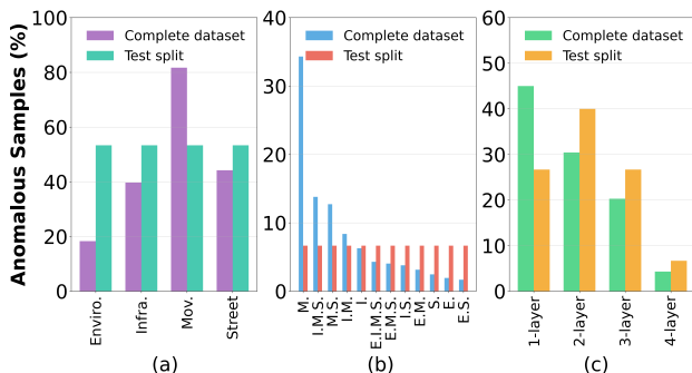
Fig. 3. Layer-wise anomaly distribution comparing CODALM_medium dataset (5,078 samples) and its test split (1020 samples):(a) Individual layer frequency across the four semantic layers, (b) Anomaly layer combination frequency, (c) Multi-layer anomaly frequency distribution.
