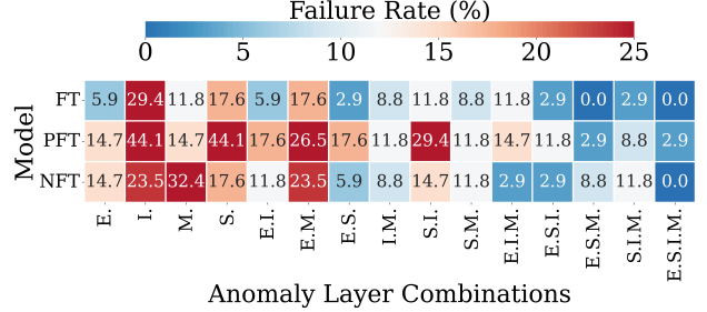
Fig. 5. Failure rates (%) across semantic layer combinations for three Qwen2.5-VL-7B variants: FT (Fine-Tuned), PFT (Pipeline Fine-Tuned), and NFT (Non-Fine-Tuned). Layer abbreviations: S (Street), I (Infrastructure), M (Movable Objects), E (Environmental). Multi-layer combinations (e.g., E.S.I.M) represent anomalies spanning multiple semantic contexts.
