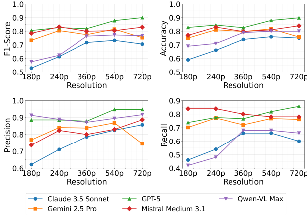
Fig. 4. Resolution comparison analysis across different image resolutions for the best-performing models of each family. Performance shows significant improvements up to 360p with diminishing returns (or worse performance) at higher resolutions.
