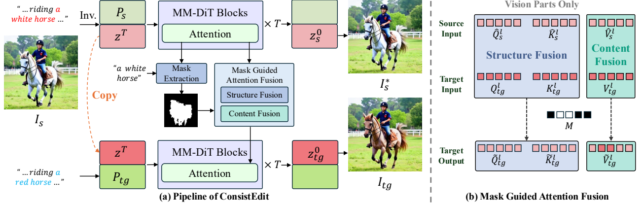
Fig. 3. (a) shows the ConsistEdit pipeline. Given a real image or video I_s and source text tokens P_s , we first invert the source to obtain the vision tokens z_s^T , which is concatenated with the target prompt tokens P_{tg} and passed into the generation process to produce the edited image or video I_{tg} . During inference, a mask M generated by our extraction method delineates editing and non-editing regions. We apply structure and content fusion to enable prompt-aligned edits while preserving structural consistency within edited regions and maintaining content integrity elsewhere. (b) illustrates the mask-guided attention fusion for timesteps where t > (1 - \alpha)T , which is applied exclusively to the vision parts, while the text parts remain unchanged.
