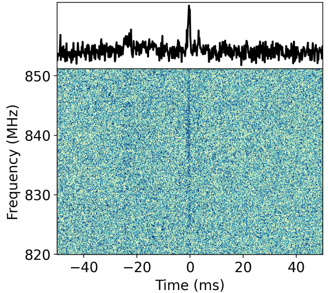
Figure 5. The discovery pulse of MTP0068 at UTMOST. The top panel shows the frequency-averaged pulse profile, while the bottom panel shows the dynamic spectrum. The data have been dedispersed to the detection DM of 11.5 pc cm ^{-3} .
