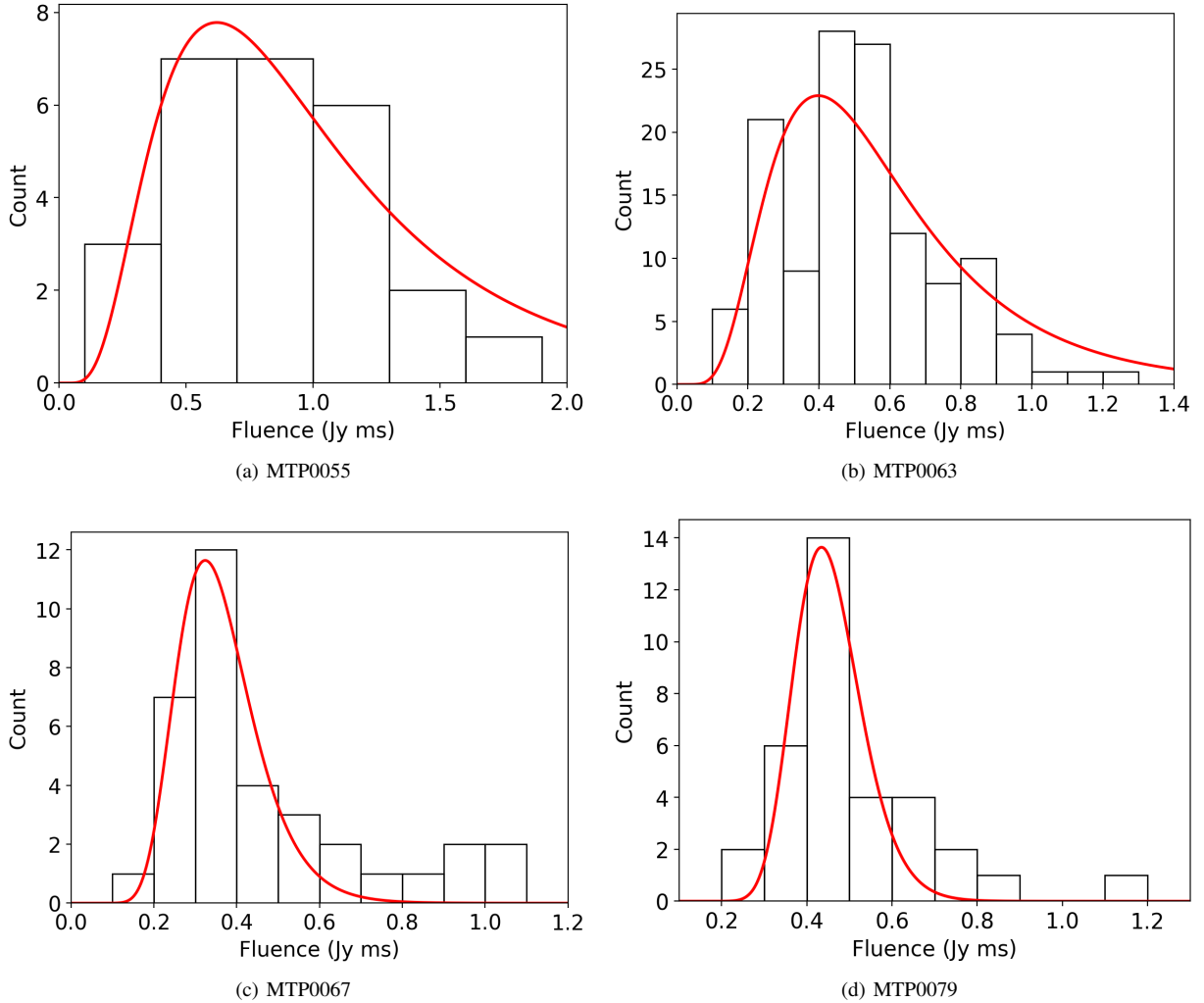
Figure 3. Fluence distributions of individual pulses for the MeerTRAP sources with imaging localisation and more than 20 pulse detections. MTP0055 is detected in both UHF (17 pulses) and L-band (9 pulses), while the other three sources are detected only in the L-band. The red line shows the best-fit lognormal distribution for the observed pulse fluences of each source.
