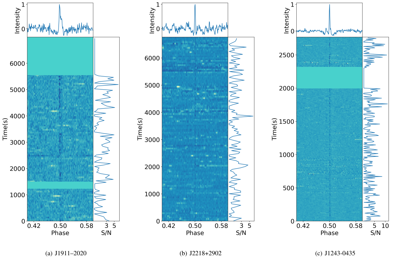
Figure 7. Three MeerTRAP sources detected in the Effelsberg follow-up observations. For each source, the main left panel shows the pulse-stack in the phase-time space, and the top panel shows the averaged pulse profile. The right panel shows the evolution of S/N with time, with the noise calculated from the off-pulse region. Blank horizontal lines in the time-phase plot represent intervals masked due to RFI. The pulsed emission of the three sources is intermittent and shows hints of nulling features.
