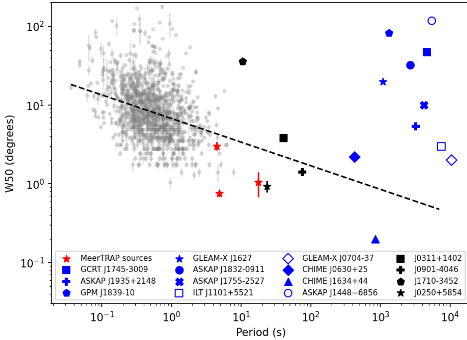
Figure 8. Duty cycle vs. pulsar period. The gray dots represent pulsars from the Thousand-Pulsar-Array programme on MeerKAT (Posselt et al. 2021), the black points represent the three long-period pulsars (Tan et al. 2018; Caleb et al. 2022; Surnis et al. 2023; Wang et al. 2025b), the blue points represent the ULP transients (Hyman et al. 2005; Caleb et al. 2024; Hurley-Walker et al. 2022, 2023; Wang et al. 2024; McSweeney et al. 2025; de Ruiter et al. 2025; Hurley-Walker et al. 2024; Dong et al. 2025a,b; Anumalapudi et al. 2025), and the red points represent the three MeerTRAP sources with persistent emission observed by Effelsberg (see Section 3.7). We indicate the ULPs with optical counterparts in empty markers. The dashed line shows the empirical relation W \propto P^{-0.3} between the observed profile width and pulsar spin period (Johnston & Karastergiou 2019).
