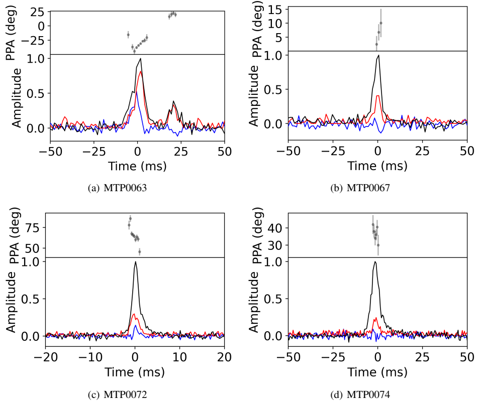
Figure 4. Polarisation profiles of bright pulses created from the transient buffer data. Each panel shows the PPA (top) and the frequency averaged pulse profile (bottom) for total intensity ( I , black), linear polarisation ( L , red) and circular polarisation ( V , blue). The polarisation data are Faraday corrected to the RM values given in Table 4. Vertical error bars indicate the 1\sigma uncertainties in the PPA.
