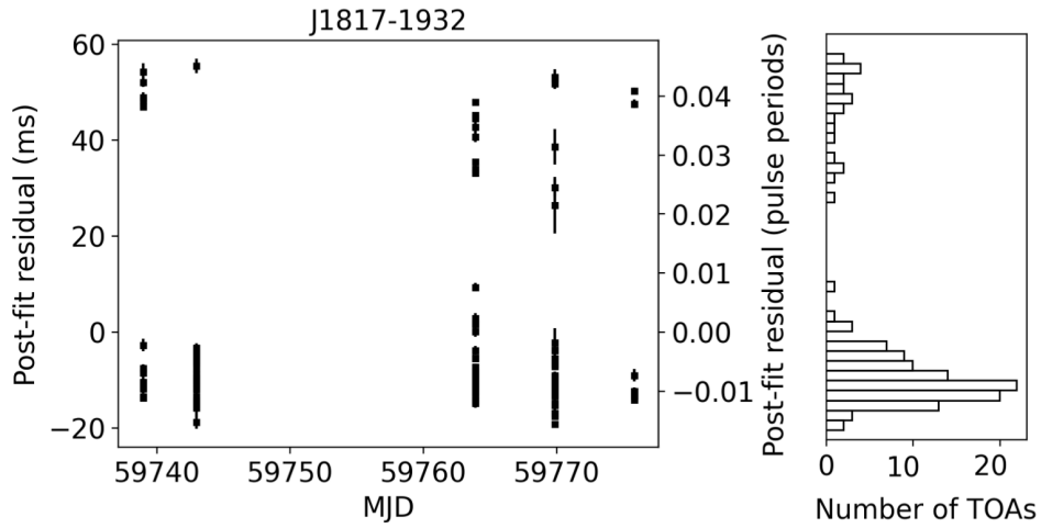
Figure 2. Best-fit timing residuals of MTP0063/PSR J1817-1932 (left) and distribution of residuals (right).
