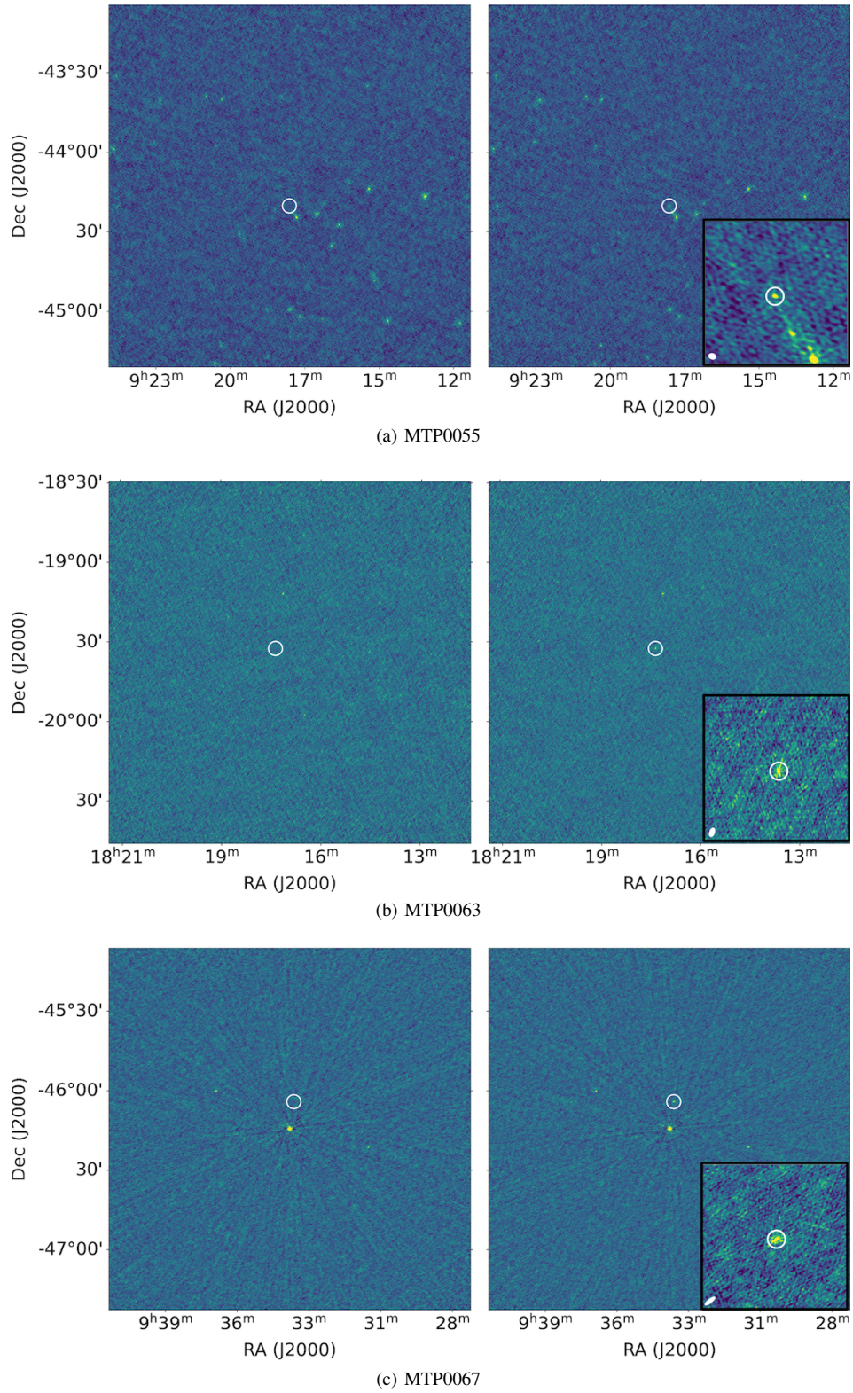
Figure A1. Images of the 9 MTP sources that triggered the transient buffer to save voltage data (see Section 2.1.3). For each source, we show the image integrated over the duration of the pulse (right) and before the pulse detection (left). The magenta circle in the on-pulse image marks the transient source identified at the pulse detection, and the inset at the bottom right corner is a zoomed-in view of the source. The synthesised beam is shown at the bottom left corner of the inset.
