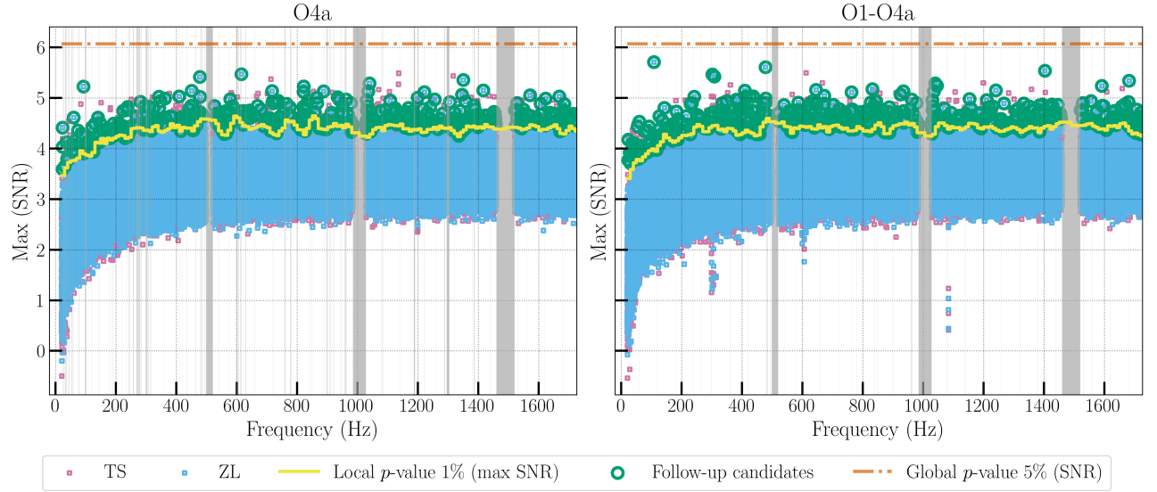
FIG. 6. Follow-up sub-threshold candidates: Left Panel: Distribution of the maximum SNR statistic (y-axis) as a function of frequency (x-axis) obtained with O4a observing run, where Max (SNR) denotes the maximum SNR across the sky within each frequency bin. Scatter points for the zero-lag and time-shifted datasets are shown in blue and magenta, respectively. Gray vertical lines indicate vetoed frequency bins excluded due to known instrumental artifacts. The brown horizontal line indicates the SNR threshold corresponding to a 5% 1-sided global p -value. The yellow curve shows the maxSNR threshold corresponding to a 99% local p -value in each 10-Hz band, smoothed over three neighboring bands. While the zero-lag data is consistent with Gaussian noise, we identify 505 sub-threshold follow-up candidates marked with teal circles, which may be further analysed using matched-filtering-based CGW search pipelines. Right Panel: Same as the left panel, but using data from O1-O4a observing runs.
