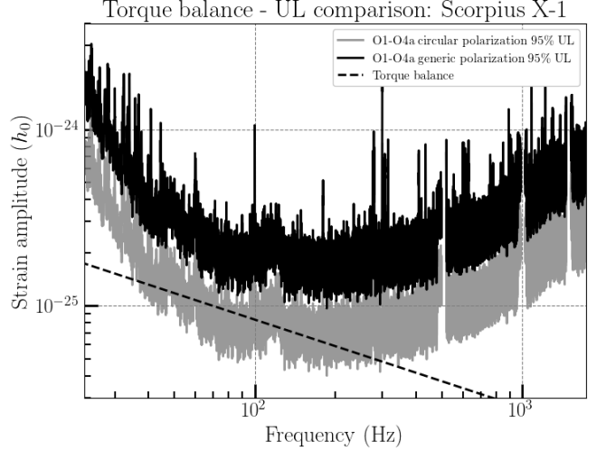
FIG. 8. Comparison of the UL for generic polarization (solid black line) and a circularly polarized signal (solid gray line) with the torque-balance level from Eq. (C12) (dashed black line). While the former does not reach the torque-balance threshold, the latter lies well below it.
