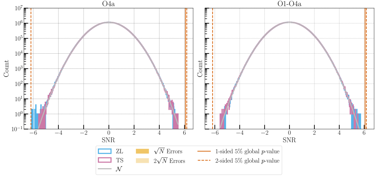
FIG. 5. ASAF search results — Significance: Left Panel: Distribution of SNR for the zero-lag (blue) and time-shifted (magenta) datasets with O4a observing run. The time-shifted (unphysical) distribution is consistent with a Gaussian (gray line) with mean -5 \times 10^{-4} and standard deviation 0.98. Poisson 1- and 2-sigma uncertainties for the time-shifted histogram are shown as a yellow-shaded region. The zero-lag histogram is largely consistent with the time-shifted data, except for non-Gaussian excess at negative SNR. Vertical brown lines (solid and dashed) indicate the 1- and 2-sided 5% global p -value SNR thresholds. Although an astrophysical signal is expected to yield a positive SNR, we investigate the origin of the observed negative SNR feature. Right Panel: Same as the figure in the right panel but with O1-O4a data.
