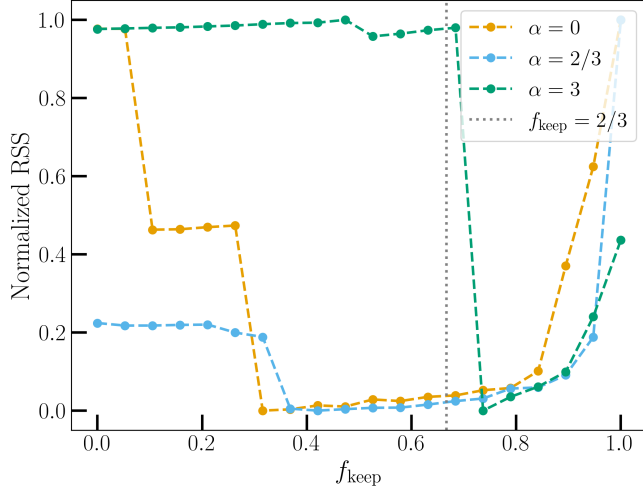
FIG. 9. Normalized RSS as a function of f_{\text{keep}} for each \alpha value.
