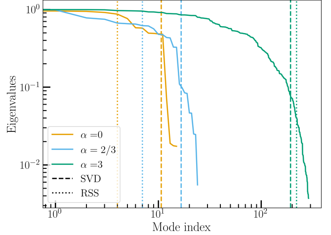
FIG. 10. Distribution of eigenvalues for the Fisher matrix with different \alpha values combining O1 to O4a data. The two dashed lines with each color compare the number of modes to keep between the conventional ( f_{\text{keep}} = 2/3 ) and new (RSS) regularization methods.
