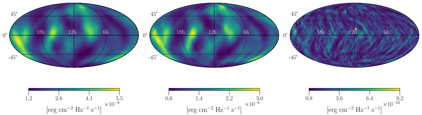
FIG. 3. 95% confidence Bayesian UL skymaps from a BBR search for point-like sources. The maps are presented in the equatorial coordinate system and show UL skymaps of the GW energy flux from the combination of all the data from O1 to O4a LIGO observing runs and the Virgo O3 data. \alpha = 0, 2/3 , and 3 are represented from left to right.
