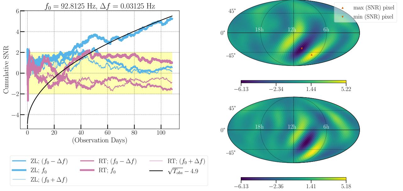
FIG. 7. Details of O4a marginal outlier towards negative SNR tail: The SNR skymap for 92.8125 Hz marginal outlier in O4a is shown in the top right panel. The positive and negative SNR blobs may be correlated through the point spread function: a GW source at the location of maximum SNR could produce a corresponding negative SNR feature next to it. To test this, we simulate skymap by injecting a source in the positive SNR direction and recover a map similar to the observed map, as shown in the bottom right panel. This motivates further investigation of both blobs. In the left panel, we show the evolution of cumulative SNR in the direction of maximum SNR (marked by an up triangle in the top right panel) as a function of observing days during O4a. The thick blue indicates the outlier frequency bin, while the two other thin blue curves represent the adjacent frequency bins immediately before and after the outlier. The magenta lines represent SNR evolution for random timeshifted data.
