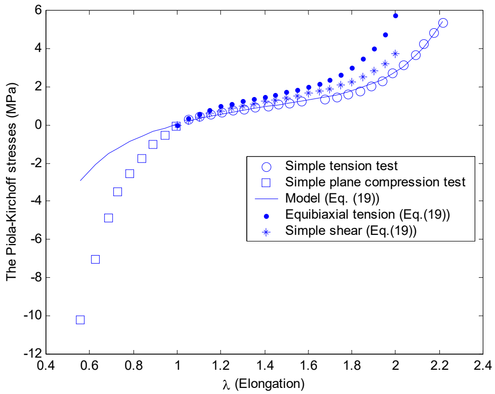
Figure 9: Stress-strain results measured in simple tension and in simple plane compression on NR 70, and the predictions of our Model.
