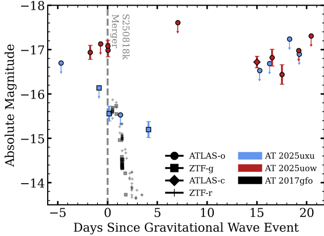
Figure 10. Light curves of the publicly available data from ATLAS and TNS on AT 2025uxu (blue) and AT 2025uow (red) as compared to AT 2017gfo (black; V. A. Villar et al. 2017). We scale the observed magnitudes of AT 2025uxu and AT 2025uow to the mean distance in the corresponding HEALPix tile in the localization map of S250818k. The merger date associated with S250818k is shown as a grey dashed vertical line. Different markers indicate different telescope filters.
