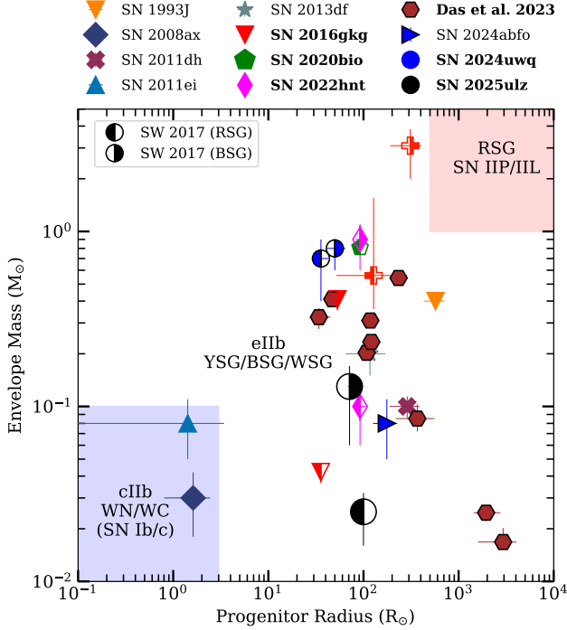
Figure 6. The shock cooling model envelope mass vs. progenitor radius for SN 2025ulz as compared to a population of SNe I Ib. SN 2025ulz lies in a similar region of parameter space to the other SNe I Ib and is in nearly the same region as SN 2016gkg using the same model. SNe highlighted in bold have values derived from similar shock-cooling modeling, while the others adopt values from alternate methods. Points with the right half filled are from the N. Sapir & E. Waxman (2017) BSG model and points with the left half filled are from the N. Sapir & E. Waxman (2017) RSG model. Published values for other SNe in this figure are obtained from: SN 1993J: S. E. Woosley et al. 1994; SN 2008ax: A. Pastorello et al. 2008; R. A. Chevalier & A. M. Soderberg 2010; SN 2011dh M. C. Bersten et al. 2012; SN 2011ei: D. Milisavljevic et al. 2013; SN 2011fu: A. Morales-Garoffolo et al. 2015; SN 2013df: A. Morales-Garoffolo et al. 2014; SN 2016gkg: I. Arcavi et al. 2017; SN 2017jgh: P. Armstrong et al. 2021; SN 2020bio: C. Pellegrino et al. 2023; SN 2022hnt: J. R. Farah et al. 2025; SN 2024uwq: B. M. Subrayan et al. 2025, SN 2024abfo: A. Reguitti et al. 2025; and K. K. Das et al. 2023.
