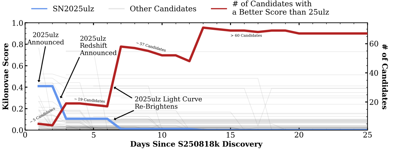
Figure 12. The evolution of the SN 2025ulz score (blue) as compared to the evolution of the scores of the rest of our candidates (grey). The red line shows the number of candidates with a better score than SN 2025ulz over time (right y-axis). The labels near the red line are the number of candidates with a score greater than SN 2025ulz at that time.
