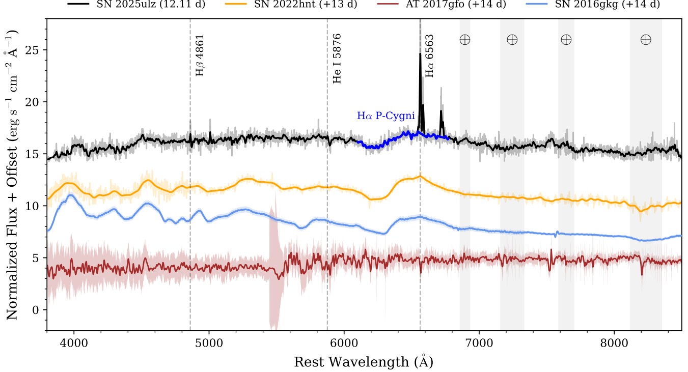
Figure 4. Comparison of the MMT optical spectrum of SN 2025ulz (black) to the type IIb SN 2022hnt (orange; J. R. Farah et al. 2025), SN 2016gkg (sky blue; L. Tartaglia et al. 2017) and the kilonova AT 2017gfo (red; E. Pian et al. 2017), all at similar phases. The low opacity colored regions behind the spectra show the 1-sigma uncertainty and the grey vertical strips are regions of telluric features. The spectral features from SN 2025ulz appear most similar to SN 2022hnt and do not show any similarity with AT 2017gfo. Most notably, the broad P-Cygni H\alpha feature highlighted in dark blue, present in both SN 2025ulz and SN 2022hnt, is not expected, nor seen, in the KN spectrum.
