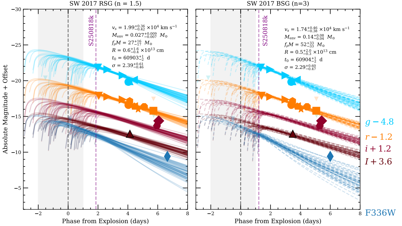
Figure 5. Fits of the griI and HST F336W (which is comparable to Swift/UVOT U -band) light curves of SN 2025ulz with a shock cooling modeling (N. Sapir & E. Waxman 2017), assuming two polytropic indices: n = 3/2 (left) and n = 3 (right). The best-fit explosion date, with uncertainties, and the detection date of S250818k are shown as grey and purple dashed lines, respectively.
