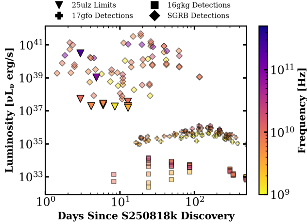
Figure 8. The radio light curves of SN 2025ulz (downward triangles as limits) as compared to SN 2016gkg (squares; N. A. J. et al. 2022 ), a sample of short SGRB radio detections (diamonds; E. Berger et al. 2005 ; A. M. Soderberg et al. 2006 ; W. Fong et al. 2014, 2015 ; G. P. Lamb et al. 2019 ; W. Fong et al. 2021 ; T. Laskar et al. 2022 ; W.-f. Fong et al. 2022 ; A. E. Nugent et al. 2024 ; G. Schroeder et al. 2024 ; A. J. Levan et al. 2024 ; G. Schroeder et al. 2025c ; Dimple et al. 2025 ; A. J. Nayana & P. Chandra 2014 ; G. E. Anderson et al. 2024 ; J. An et al. 2025b ; G. Schroeder et al. 2025a ; R. Ricci et al. 2025a ; W. Fong et al. 2025 ; G. Schroeder et al. 2025b ; L. Rhodes et al. 2023 ; A. J. Levan et al. 2009 ; R. Ricci et al. 2025c ), and AT 2017gfo (plus signs; K. D. Alexander et al. 2017 ; G. Hallinan et al. 2017 ; S. Kim et al. 2017 ; S. Makhathini et al. 2021 ; G. Hallinan et al. 2017 ; K. P. Mooley et al. 2018a,b,c ; L. Resmi et al. 2018 ; K. P. Mooley et al. 2018b,a ; D. Dobie et al. 2018 ; K. P. Mooley et al. 2018a,a ; R. Margutti et al. 2018 ; J. W. Broderick et al. 2020 ; D. Dobie et al. 2018 ; G. Ghirlanda et al. 2019 ; K. D. Alexander et al. 2018 ; E. Troja et al. 2019 ; A. Hajela et al. 2019 ). The color of the point is the representative frequency of the receiver used for the observation. Our radio limits on SN 2025ulz rule out an SGRB-like on-axis jet but do not rule out SN IIB-like or late-rising AT2017gfo-like radio emission.
