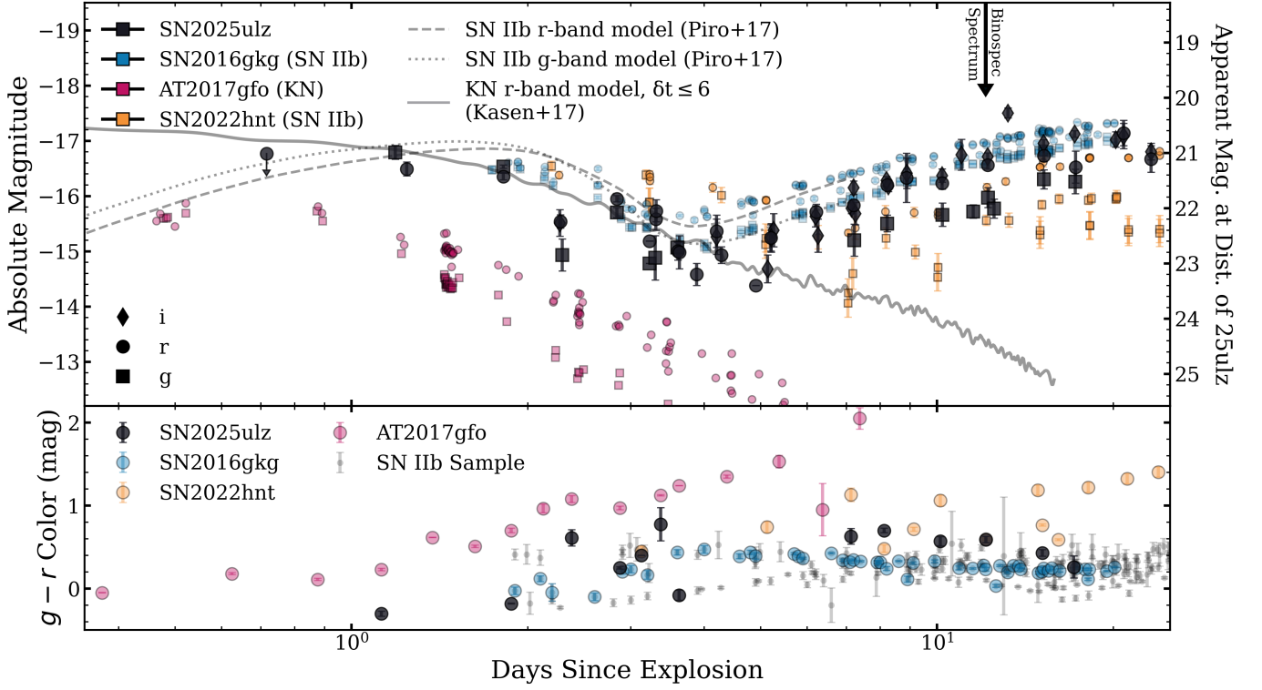
Figure 3. Top: A comparison of the gri light curves for SN 2025ulz (black), SN 2016gkg (blue; L. Tartaglia et al. 2017 ), SN 2022hnt (orange; J. R. Farah et al. 2025 ), and AT2017gfo (red; V. A. Villar et al. 2017 ). For SN 2025ulz, We choose an explosion date of MJD=60904 based on our shock cooling modeling (see subsection 4.2 ). The best fit ( i.e. , lowest sum of the residual squared) r -band KN model (from D. Kasen et al. 2017 ) to SN 2025ulz for the early time ( \delta t \leq 6 days) light curve decline is shown as a solid line. We also show the r - (black dashed line) and g -band (black dotted line) models for SN 2016gkg from A. L. Piro et al. (2017) . At phase \delta t \lesssim 6 days all four observed light curves appear to redden as they fade rapidly at around the same rate. At \delta t \gtrsim 6 days, the light curves of SN 2025ulz and the other SNe I Ib begin to re-brighten while the KN light curve continues to fade rapidly. Bottom: The g-r color evolution of SN 2025ulz as compared to AT 2017gfo, SN 2016gkg, SN 2022hnt, and 7 other SNe I Ib (SN 1993J, M. W. Richmond et al. 1994 ; SN 2008ax, A. Pastorello et al. 2008 ; SN 2011dh, I. Arcavi et al. 2011 ; SN 2011ei, D. Milisavljevic et al. 2013 ; SN 2011fu, A. Morales-Garoffolo et al. 2015 ; SN 2013df, A. Morales-Garoffolo et al. 2014 ; SN 2024uwq, B. M. Subrayan et al. 2025 ). The color evolution of SN 2025ulz is very similar to the rest of the SNe I Ib population.
