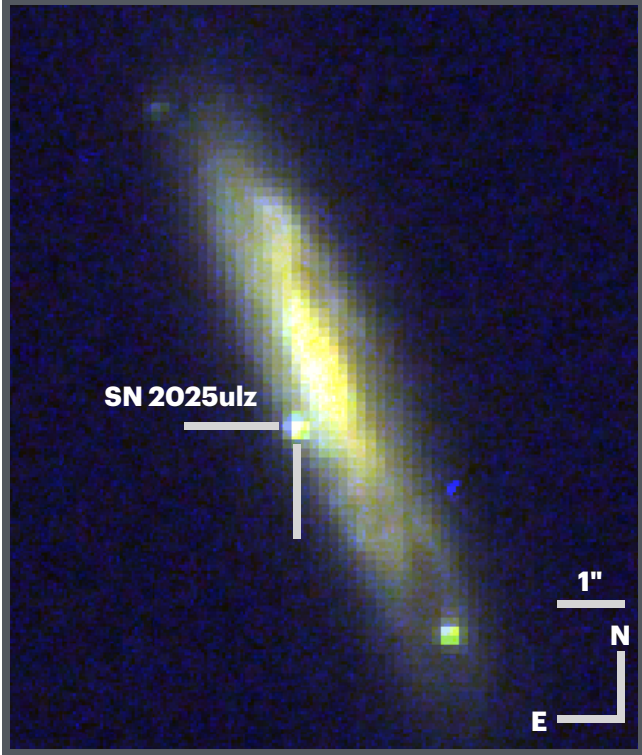
Figure 2. A false color image of the HST WFC3 observations of SN 2025ulz. We include the F606W image from 26 Aug (blue; \delta t \sim 8 days), the F110W image from 27 Aug (green; \delta t \sim 9 days), and the F160W image from 28 Aug 2025 (red; \delta t \sim 10 days). We highlight the position of SN 2025ulz showing its close in projection to the core of its host galaxy.
