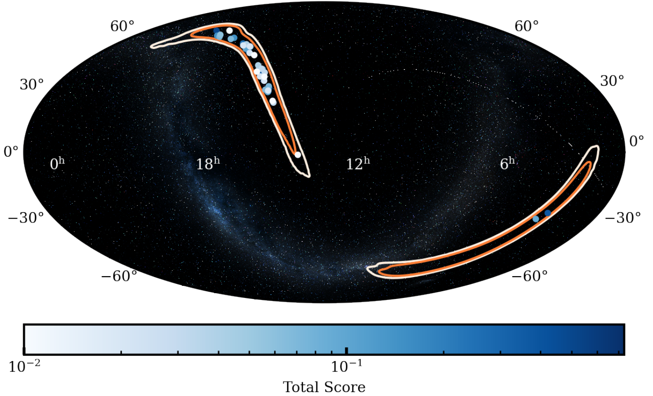
Figure 1. The IGWN (International Gravitational Wave Network) skymap credibility contours (orange: 50%, white: 90%) of S250818k, and the locations of all 121 candidates we found within the 95% credibility region from the Transient Name Server (TNS). The color of the point represents the overall score from our vetting, which is described in section 5 .
