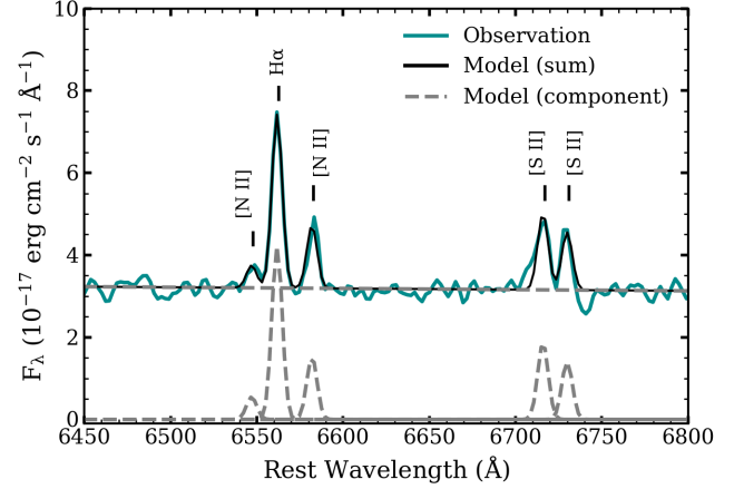
Figure 7. Model of our Keck spectrum that is dominated by emission from the SN 2025ulz host. We use this model to derive a star formation rate for the host galaxy for comparison with our radio derived star formation rate.
