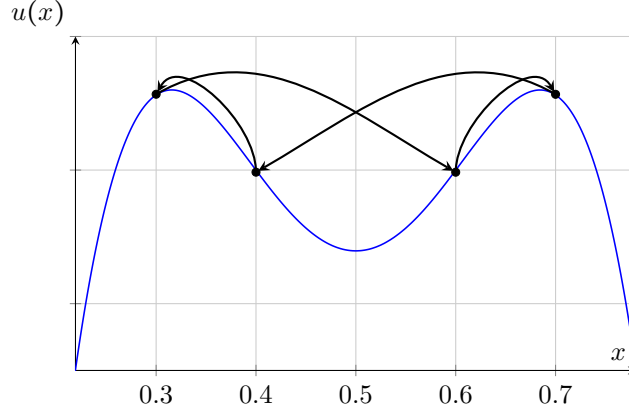
Figure 2: The example corresponding to Proposition 3.2 , demonstrating that having zero regret, let alone sublinear, has no implications concerning convergence in terms of KKT gap.
