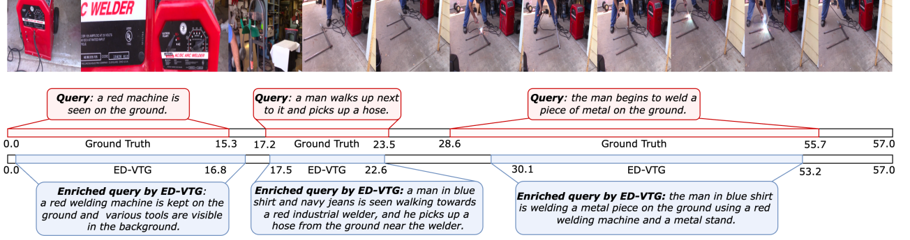
Figure 3. Example of query enrichment and detection made by ED-VTG on video paragraph grounding (VPG) task from the ActivityNet-Captions [36] dataset. In this specific sample, three different queries are enriched and localized together.
