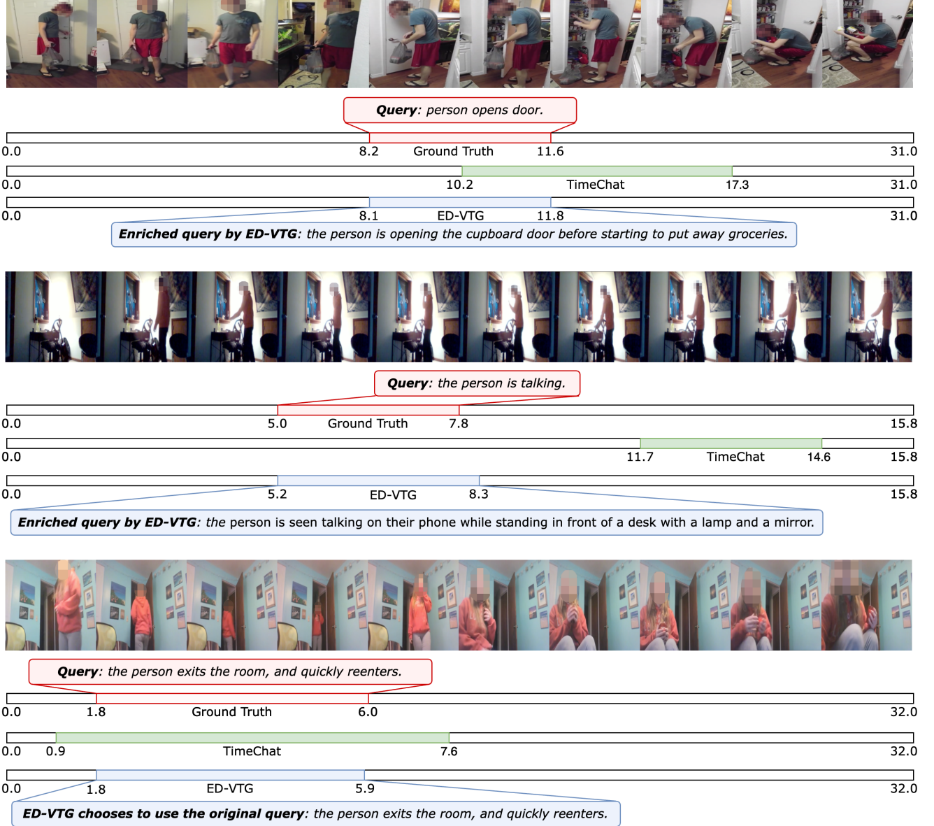
Figure A.1. Examples of query enrichment and localization made by ED-VTG on single-query temporal grounding (STG) task from the Charades-STA [18] dataset. We also show the prediction made by one baseline model, TimeChat [82], which directly ground the input queries using raw-text timestamp representation. Since we train ED-VTG using the MIL paradigm, the model can choose to use the input query directly or enrich it during evaluation. In the last example, since the input query is clear and explicit, the model directly localizes it.
