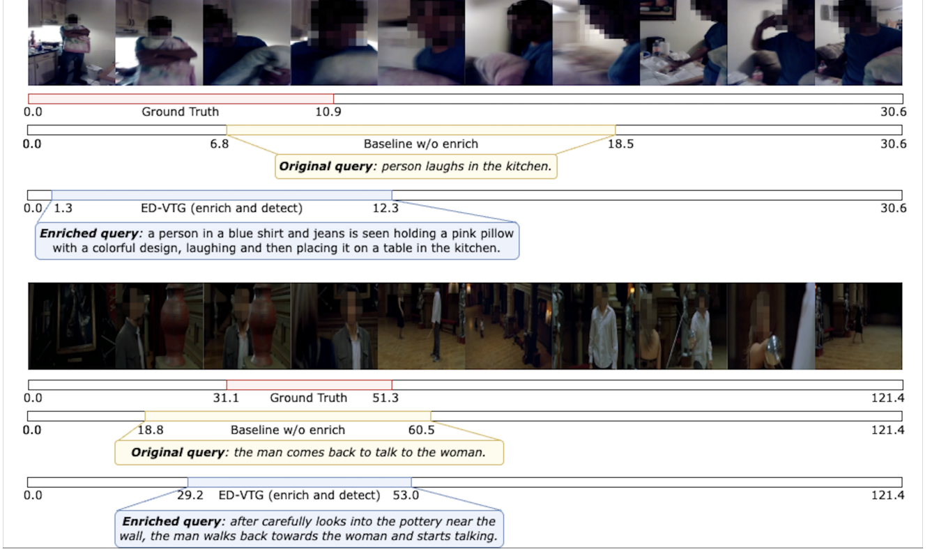
Figure A.2. Comparison of detections of ED-VTG using its predicted enriched queries against a baseline version trained to always use the original queries. The enriched queries contain additional relevant details and context that enable ED-VTG to perform more accurate temporal localization. In the first example, which is taken from Charades-STA [18], the additional details in the enriched query provide a more complete description of objects and actions that is more easily groundable. In the second example, sourced from the ActivityNet-Captions [36] dataset, the enriched query provides additional temporal context which leads to more precise temporal boundary prediction.
