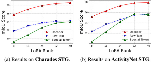
Figure B.1. Ablation study on timestamp representation by the interval decoder. We compare performance of our proposed lightweight decoder vs timestamp as raw text [26, 46, 57, 82] vs timestamp representation by special tokens [27, 73, 98], and find the decoder to be significantly better than both other techniques. Reported results are in FT w/o PT setting.
