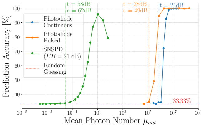
FIG. 10: Prediction accuracy in relation to the mean photon number \mu_{out} , after normalizing the average power to 10 W for thermal damages ( t ) and 1 MW for ablation damages ( a ), for which the respective countermeasure attenuation is reported at the top.
