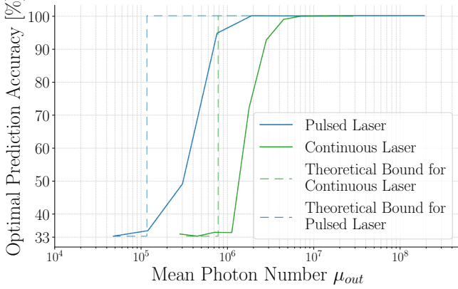
FIG. 8: Results on optimal prediction accuracy based on the mean photon number \mu_{out} for the continuous and pulsed laser attack.
