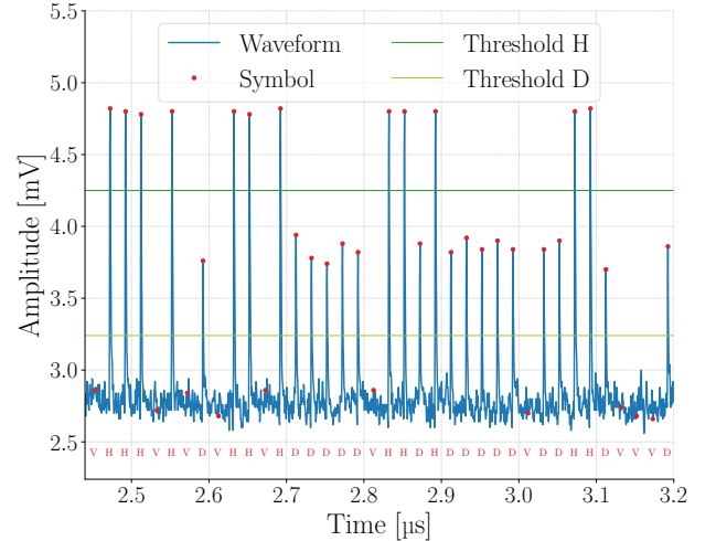
FIG. 7: Waveform with calculated symbol positions and classified symbols for the pulsed laser attack. Red dots show estimated symbol locations, thresholds are used to classify the symbol as |H\rangle , |V\rangle , or |D\rangle (if the symbol is above the threshold H, the symbol is classified as |H\rangle , between the thresholds H and D, it is classified as |D\rangle , otherwise it is classified as |V\rangle ).
