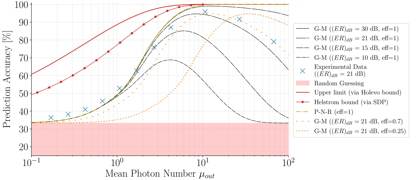
FIG. 2: Theoretical prediction accuracy with respect to the mean photon number \mu_{out} , varying different POVMs, extinction ratios of the projective measurements, efficiencies, and experimental data for comparison.
