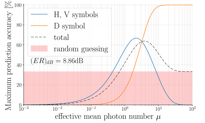
FIG. 3: Theoretical detection probabilities for each state and the total with respect to the mean photon number \mu_{out} in the use-case of only two detectors (Extinction Ratio = 8.86 dB).
