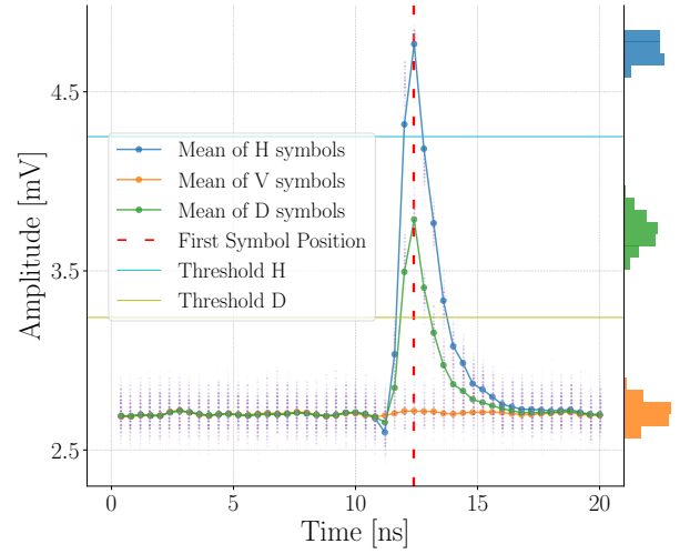
FIG. 6: Mean of |H\rangle , |V\rangle , and |D\rangle symbols in time modulo period, result of the optical modulation in pulsed regime by the iPOGNAC during the THA. Data points are reported in purple. Red vertical line shows the detected position of the first symbol in the original waveform. Statistical distributions of these symbols are displayed on the right.
