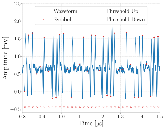
FIG. 5: Waveform with calculated symbol positions and classified symbols for the CWLA. Red dots show the estimated symbol locations, while thresholds are used to classify the symbol as |H\rangle , |V\rangle , or |D\rangle (if the symbol location is above the threshold up, the symbol is classified as |V\rangle , if it is between the thresholds up and down, it is classified as |D\rangle , and if it is below the threshold down, it is classified as |H\rangle ).
