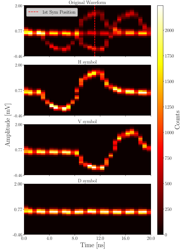
FIG. 4: 2D-histogram of the waveform resulting from the oscilloscope, result of the optical modulation in continuous wavefront by the iPOGNAC during the THA, and |H\rangle , |V\rangle and |D\rangle symbols separately. All the waveforms presented are calculated by performing a modulo-period operation. In the top plot, the red vertical line shows the detected position of the first symbol in the original waveform.
