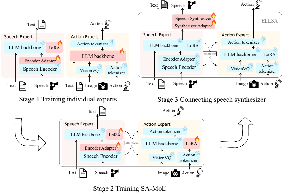
Figure 3: The training strategy of ELLSA. First train individual experts, then build SA-MoE backbone by integrating these experts, finally connect speech synthesizer. Across these stages, both training tasks and trainable parameters evolve to suit the model’s growing capabilities.
