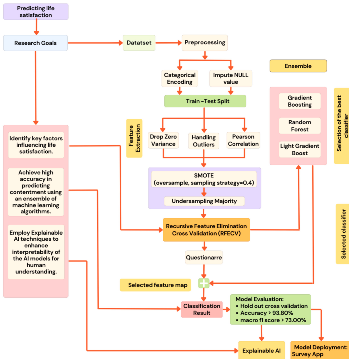
Fig. 1. Workflow diagram that outlines the key steps used in applying machine learning algorithms, addressing research objectives, and highlighting the main evaluation results.
