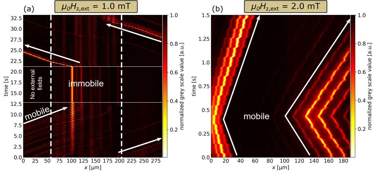
Figure 3: Motion behavior of SPBs dispersed in water on top of a magnetically patterned substrate with increasing stripe domain width for two different external magnetic field amplitudes in z -direction. A qualitative impression of the SPB transport is given by presenting averaged lateral intensity profiles of each recorded image frame as a function of recording time. The color scale indicates the image intensity; high intensity represents the background and low intensity the presence of SPB rows. For weak external magnetic field pulses of \mu_0 H_{z,\text{ext}} = \mu_0 H_{x,\text{ext}} = 1.0 \text{ mT} magnitude (a), fractions of mobile and immobile SPBs were distinguishable in dependence on the substrate position. The immobilization of SPBs occurred at a substrate area between \approx 60 \mu\text{m} and \approx 200 \mu\text{m} lateral x -position (marked by dashed white lines), coinciding with the substrate region of largest stripe domain width. Mobile SPBs were initially transported from left to right until immobilization. After a pause, the external field sequence was modified so that SPB transport from right to left was initiated. Most of the previously mobile SPBs regained their mobility by this. Stronger field pulses of \mu_0 H_{z,\text{ext}} = 2 \text{ mT} magnitude (b) lead to mobilization of SPBs even for the region of largest stripe domain width.
