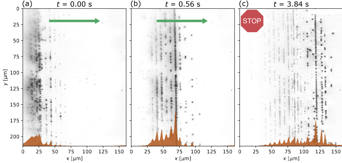
Figure 5: Fractionation of differently sized SPB populations on top of a magnetically stripe domain patterned substrate with increasing stripe width. (a) All SPBs are assembled on the left edge of the microscope's field of view, resembling minimal stripe domain width in the underlying substrate. (b) Upon application of an external magnetic field pulse sequence of constant frequency, all SPBs are transported to the right side of the field of view. (c) After a short time, the SPBs are immobilized (oscillatory motion) at specific locations. Statistically, smaller SPBs ( d = 1 \mu\text{m} ) are immobilized earlier (at lower lateral x -position) than larger SPBs ( d = 2.8 \mu\text{m} ). The two SPB populations were spatially separated into distinguishable fractions. Averaged intensity profiles (brown-filled curves) indicate the lateral extent of each fraction above the substrate surface.
