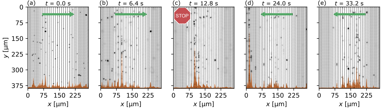
Figure 2: Optical analysis for the motion behavior of SPBs dispersed in water on top of a magnetic stripe domain pattern with gradually varied stripe width. Shown are single optical microscope images (a)-(e) obtained at different recording times t of a video recording taken with a frame rate of 25 fps. For the recorded experiment, a periodic sequence of trapezoidal magnetic field pulses with T/4 = 0.1 s and \mu_0 H_{\max,x} = \mu_0 H_{\max,z} = 1 mT was applied. The stripe domain pattern within the underlying substrate is indicated in each displayed frame by black dashed lines. For frames (a) and (b), SPBs (black spots) are transported from left to right across the substrate (see green arrows), leading eventually to immobilization at a lateral x -position of ca. 100 \mu\text{m} , prominently visible in (c). Here, the external field sequence was stopped and paused for 8 s, resulting in a halted SPB motion. Upon re-initialization of the external field sequence with inverted phase relation between field pulses in z - and x -direction, SPBs are transported into the opposite direction, emphasized in (d) and (e) by the green arrows. Frame (e) highlights the immobilization of SPBs this time around ca. 200 \mu\text{m} x -position. Lateral particle density profiles, averaged along the y -dimension, are included as brown-filled curves in each frame.
