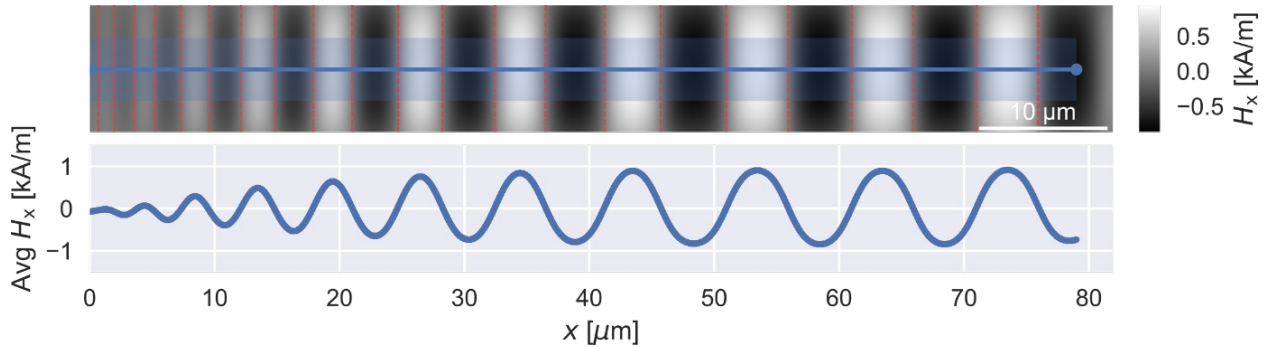
Figure S4: Spatial distribution of the magnetic stray field component H_x emerging from an exchange-biased thin film system patterned with magnetic parallel stripe domains with gradually increasing stripe width. Red dashed lines indicate boundaries of stripe domains (domain walls). The field distribution was derived from micromagnetic simulations for a distance of 2500 nm above the magnetic thin film system. A line profile visualizes the lateral evolution of H_x , averaged over the blue-shaded area.
