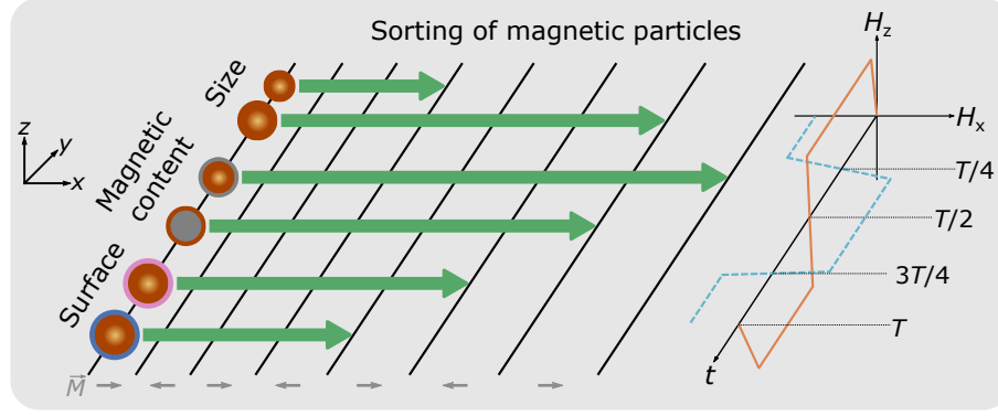
Figure 1: Schematic concept for the spatial fractionation of MPs in a microfluidic environment based on their directed transport above a magnetic stripe domain pattern with gradually increasing stripe width. MPs of varying characteristics (size, magnetic content distribution, surface properties) are expected to be immobilized at a locally different position along the domain pattern, depending on the respective stripe width. In this work, we experimentally demonstrate the feasibility of the fractionation concept by separating differently-sized MPs. The domains are magnetized as indicated by the grey arrows, resulting in a head-to-head (hh)/tail-to-tail (tt) magnetization configuration. A periodic sequence of trapezoidal magnetic field pulses in the vertical z -direction (solid, orange line) and the lateral x -direction (blue, dashed line) with a fixed alteration frequency is applied to achieve MP separation.
