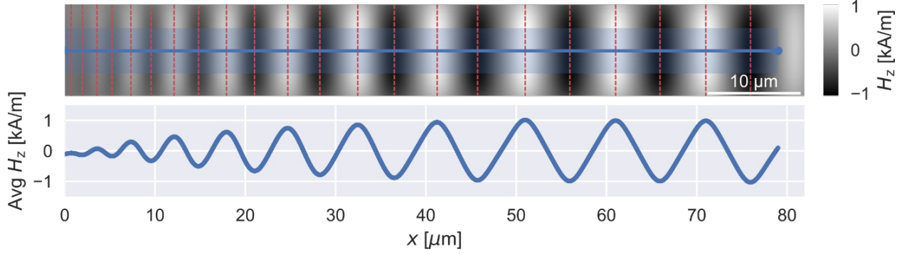
Figure S3: Spatial distribution of the magnetic stray field component H_z emerging from an exchange-biased thin film system patterned with magnetic parallel stripe domains with gradually increasing stripe width. Red dashed lines indicate boundaries of stripe domains (domain walls). The field distribution was derived from micromagnetic simulations for a distance of 2500 nm above the magnetic thin film system. A line profile visualizes the lateral evolution of H_z , averaged over the blue-shaded area.
