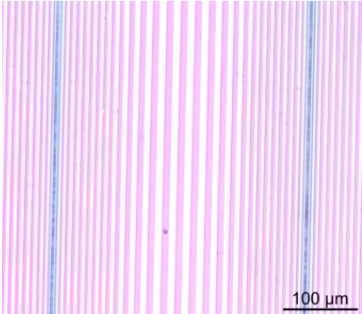
Figure S1: Image of lithographically structured resist utilized for the ion bombardment induced magnetic patterning of an exchange-biased thin film system, obtained by optical microscopy.
