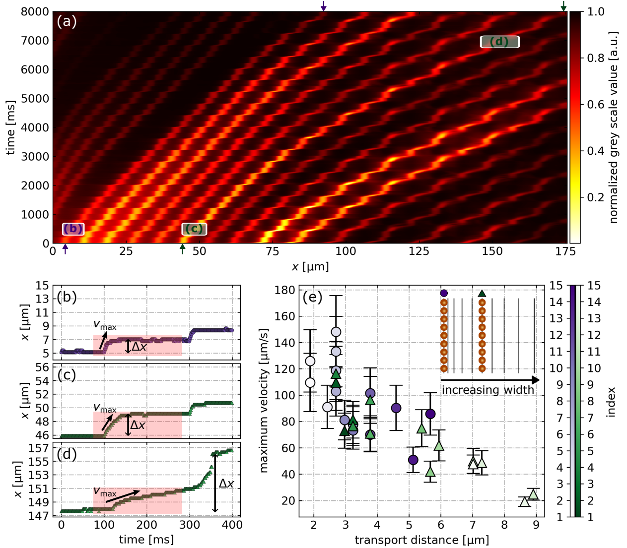
Figure 4: Quantitative analysis of SPB motion dynamics in water above a magnetically patterned substrate with increasing stripe domain width. Starting from the evolution of averaged lateral intensity profiles acquired from each recorded image frame during the experiment (a), three SPB row trajectory snippets highlighted with white-framed rectangles were picked as examples for the identification of maximum particle velocity in (b) - (d). The period of the external magnetic field pulse sequence was chosen to be T = 0.8 s with pulse magnitudes of \mu_0 H_{z,\text{ext}} = \mu_0 H_{x,\text{ext}} = 1 mT to initiate SPB transport from left to right throughout all domain widths present in the underlying substrate (no immobilization). Maximum SPB row motion velocities, as a measure for their averaged mobility, were determined for the transport step initiated after changing the sign of the external field in z -direction. The red-marked areas for the exemplary trajectory data x(t) in (b) - (d) were considered for the velocity calculation by fitting a Gaussian error function to the marked data and subsequently obtaining the velocity as the maximum of the fit's time derivative. Each velocity is assigned a transport step distance \Delta x , which corresponds to the difference between two consecutive plateaus in the trajectory data (see further explanation in the text). Plotting the obtained velocities as a function of the respective transport distance for the two SPB row trajectories that contain the exemplary steps of (b) - (d), a decreasing tendency for the velocity with larger transport steps (larger domain width) is observable (e).
