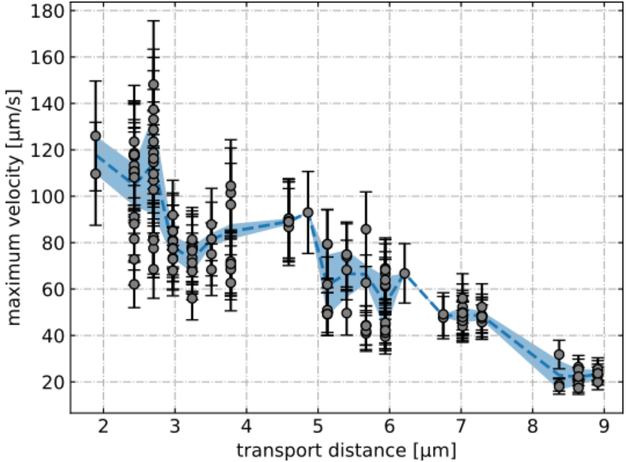
Figure S2: Maximum step velocity as a function of transport step distance determined for micron-sized superparamagnetic beads moving on top of a magnetically stripe domain patterned substrate with gradually increasing stripe width. Error bars indicate the uncertainty of velocity for a single transport step. The blue dashed line marks the development of the average maximum velocity with an overall decreasing tendency with increasing transport step distance/stripe domain width. The blue shaded area indicates the standard deviation of the average velocities.
