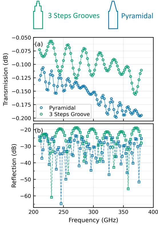
Fig. 2. Co-polar performance of two broadband AR unit cells at normal incidence. (a) Transmission Tx and (b) reflection Rx for a pyramidal profile and a three-step groove profile. Curves for both incident linear polarizations (TE: E \parallel \text{grooves} , TM: E \perp \text{grooves} ) are overlaid; co-polar transmission/reflection are indistinguishable at normal incidence. Both unit cells share the same pitch ( p ) and depth ( h ); the three-step layer heights/widths were chosen to approximate the triangular effective-index gradient.
