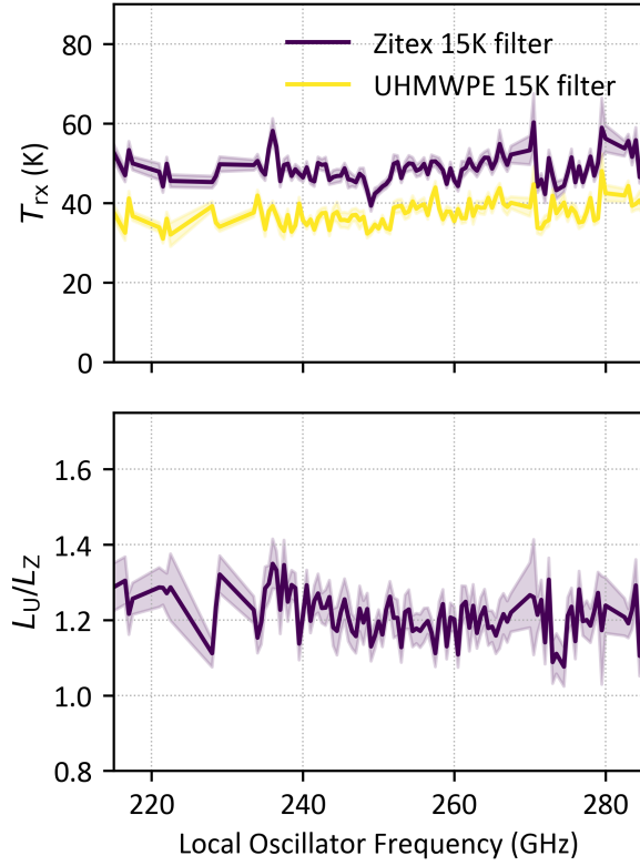
Fig. 10. a) Measured double-sideband noise temperature T_{rx} as a function of the local oscillator frequency for the heterodyne receiver loaded with a single-sheet Zitex filter or a UHMWPE filter, both mounted at the 15 K thermal shield. b) Relative insertion loss between the Zitex and UHMWPE filters across the same band.
