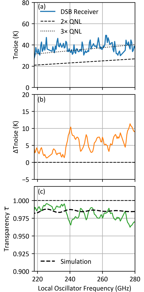
Fig. 8. DSB receiver performance and window characterization in Band 6 frequency range. (a) Measured DSB noise temperature as a function of local oscillator frequency for the bare receiver, with 2 \times and 3 \times quantum-noise limits overlaid ( h\nu/2k_B ). In these measurements, the receiver was already equipped with a structured UHMWPE infrared filter placed at the 15K stage (see Fig 10) (b): Change in DSB noise temperature ( \Delta T_{noise} ) upon insertion of UHMWPE windows with front-surface corrugations oriented perpendicular to the polarisation direction of the receiver. (c) Derived optical transparency \eta of the window, computed from the baseline noise difference at T_{phys} = 290\text{K} along with the simulated transmission.
