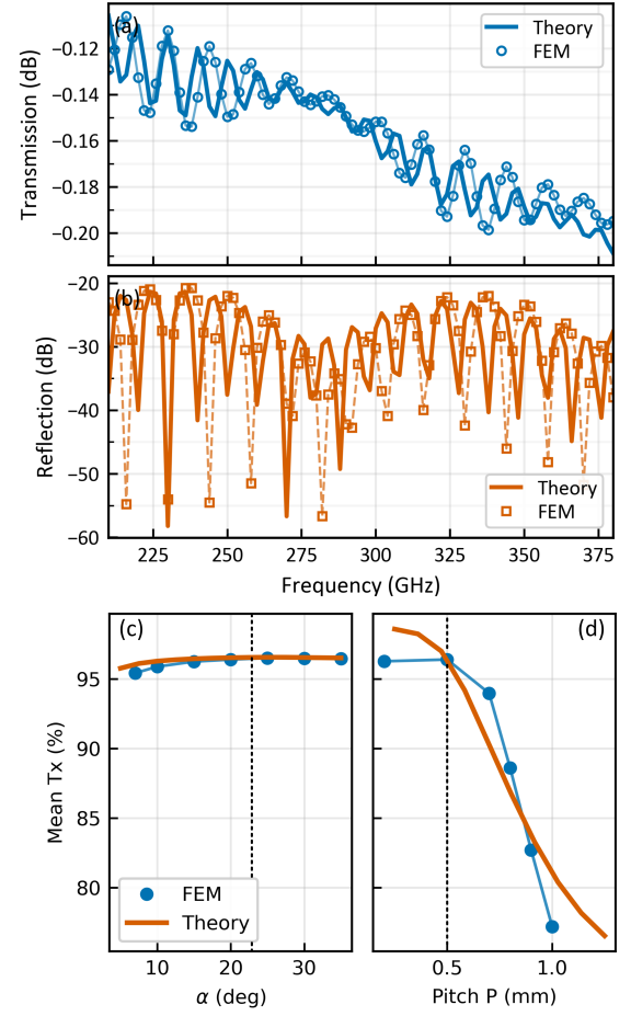
Fig. 3. Comparison of full-wave (FEM) and effective-medium (EMT) models for the UHMWPE pyramidal AR window and parametric sensitivity of the mean transmission. TE and TM polarisation are perfectly overlaid. (a) Normal-incidence co-polar transmission T(f) from 211–373 GHz for a single unit cell solved with FEM (periodic boundaries, Floquet ports) and with EMT (staircase discretization of the graded profile and transfer-matrix propagation). (b) Corresponding co-polar reflection R(f) over the same band. (c) Band-averaged transmission \bar{T}_{211-373\text{GHz}} versus apex angle \alpha at fixed pitch p=0.5\text{mm} . (d) Band-averaged transmission versus pitch p at fixed \alpha = 22^\circ . The dashed lines indicate the nominal design values used for fabrication of the AR structure.
