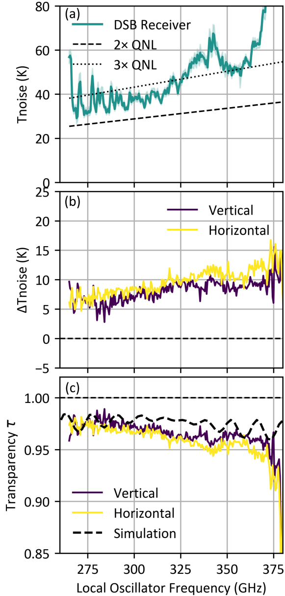
Fig. 9. DSB receiver performance and window characterization in the Band 7 frequency range. Caption details as in Fig.8, but measurements correspond to the higher frequency band (275–373 GHz). Additionally, measurements in (b) and (c) include tests with the window grooves oriented both vertically (aligned) and horizontally (orthogonal) to the receiver’s polarization.
