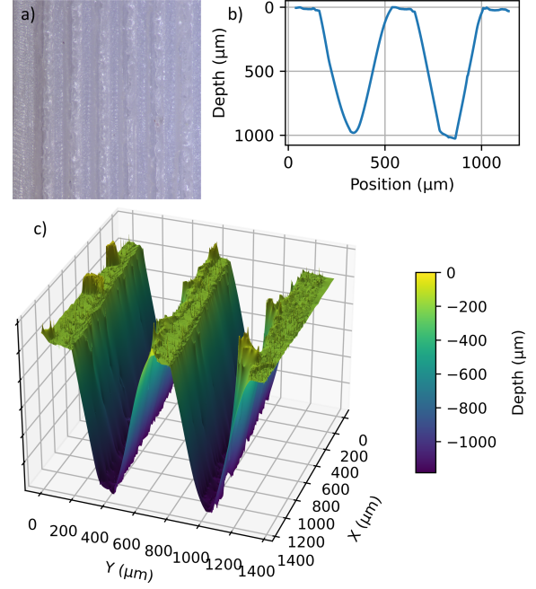
Fig. 5. a) Top-view optical image of the machined pyramidal corrugation on the UHMWPE window, showing the uniform two-dimensional array of grooves. (b) Optical-profilometer cross-section cut through adjacent grooves, showing a valley flat width of approximately 50 \mu\text{m} , a truncated pyramid apex flat of 150 \mu\text{m} , and an apex angle of 15^\circ . (c) Three-dimensional optical-profilometer rendering of the corrugation, showing the uniform facet slopes.
