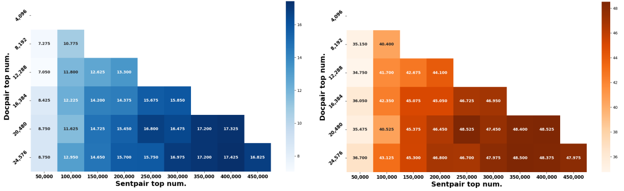
Figure 5: Results of Avg BLEU (left) and Avg ChrF (right) for OT w/Mean with OFLS (40, 0.5).
