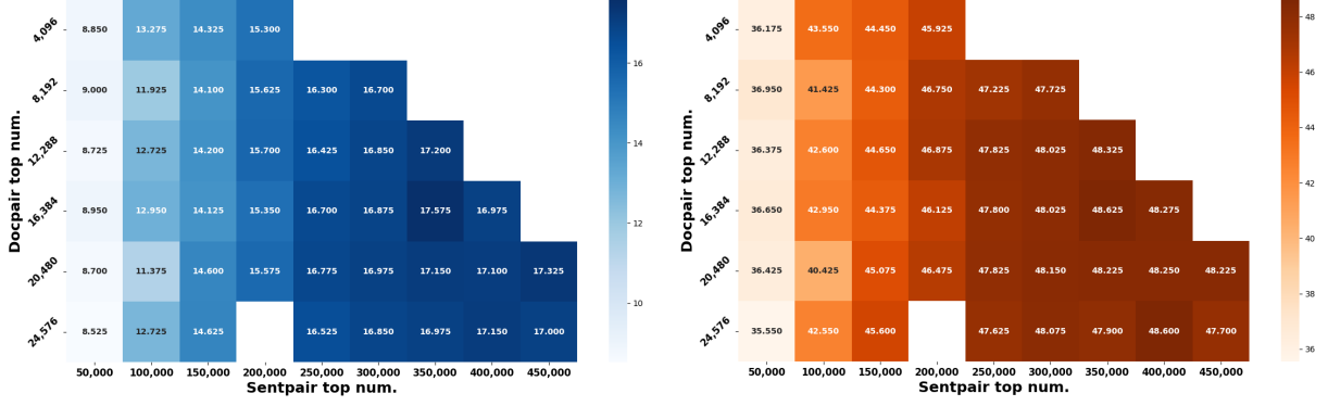
Figure 4: Results of Avg BLEU (left) and Avg ChrF (right) for Mean-Pool with OFLS (40, 0.5).
