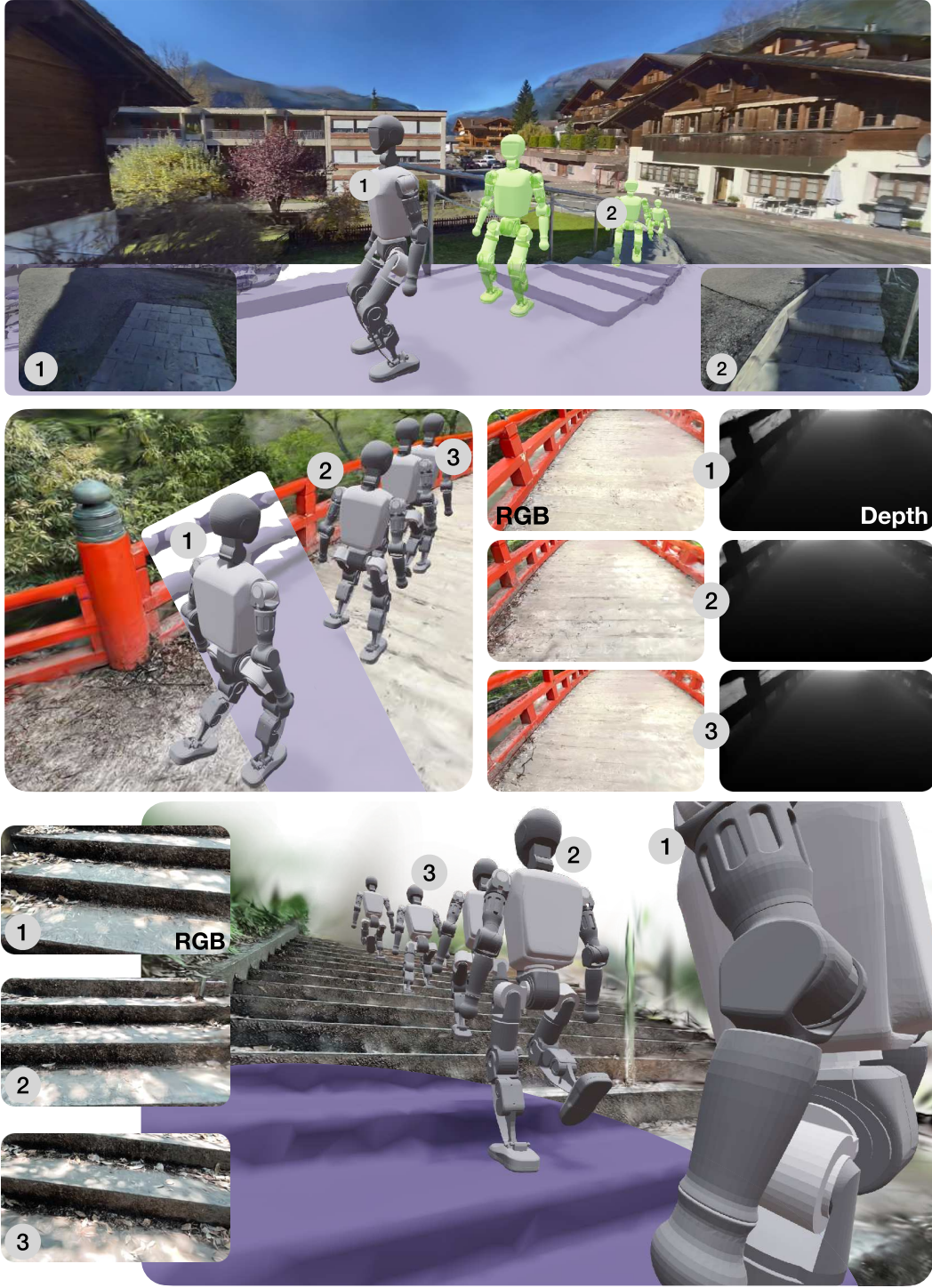
Figure 3: Velocity-tracking policies trained directly from pixels in GaussGym : Photorealistic environments provide diverse training scenes, enabling policies to follow commanded velocities from RGB input. GaussGym supports large-scale training with synchronized RGB and depth at over 100\text{K} \frac{\text{steps}}{\text{s}} across 4,096 parallel environments on an RTX4090 rendering at 640 \times 480 .
