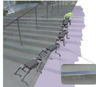
(a) RGB policy pre-trained in GaussGym.
