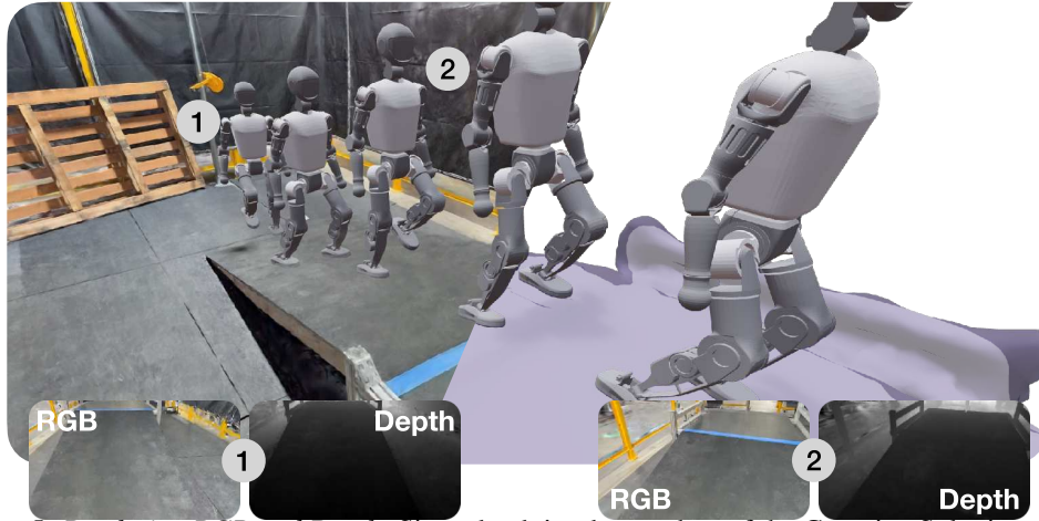
Figure 5: Rendering RGB and Depth : Since depth is a by-product of the Gaussian Splatting rasterization process, GaussGym also renders depth without increasing rendering time.
