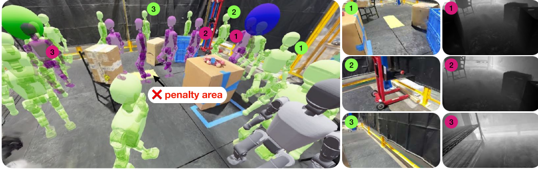
Figure 8: Semantic reasoning from RGB : In the sparse goal tracking task, the robot must cross an obstacle field where a yellow floor patch incurs penalties. The RGB-trained policy ( green ) perceives and avoids the patch, while the depth-only policy ( purple ) cannot detect it and walks through. This highlights how RGB provides semantic cues beyond geometric depth.
