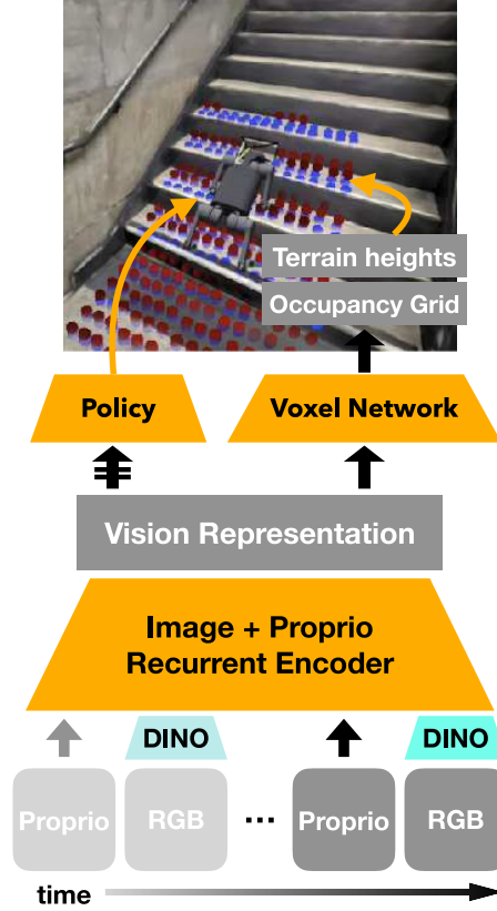
Figure 7: Architecture for Visual Locomotion : An LSTM encoder fuses proprioception with DinoV2 RGB features. Outputs feed into a 3D transpose conv head for occupancy and terrain prediction, and a policy LSTM that outputs Gaussian action distributions.
