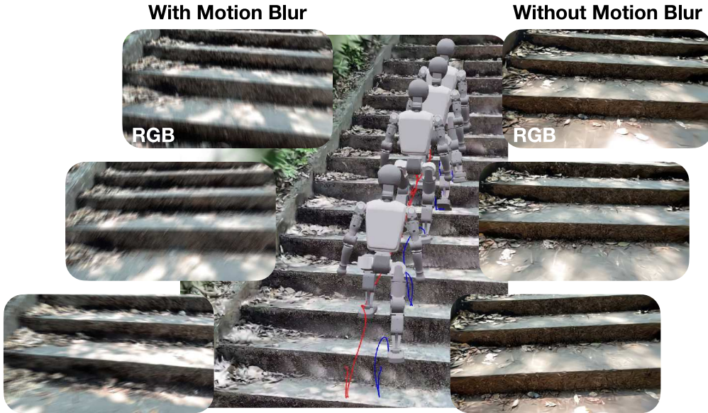
Figure 10: GaussGym proposes a simple yet novel to simulate motion blur. Given the shutter speed and camera velocity vector, GaussGym alpha blends various frames along the direction of motion. The effect is pronounced in jerky motions, for example when the foot comes into contact with stairs.
