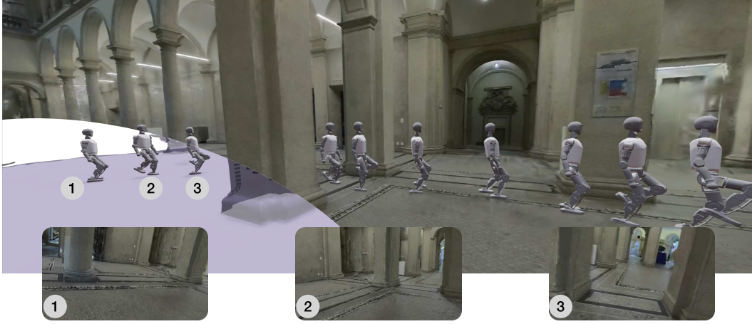
Figure 9: Large photorealistic worlds : GaussGym incorporates open-source datasets, such as GrandTour (Frey et al., 2025), which contains high quality scans of large areas. Shown above is a 20 m 2 GaussGym scene derived from GrandTour, including the mesh (purple) and robot POV renders.
