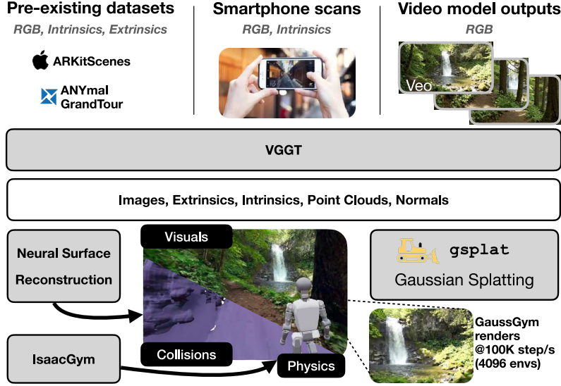
Figure 2: Data collection overview : GaussGym ingests data from various data sources and processes them with VGGT (Wang et al., 2025) to obtain extrinsics, intrinsics, and point clouds with normals. The former two data products are used to train 3D Gaussian Splats for rendering, while the latter two are used to estimate the scene collision mesh.
