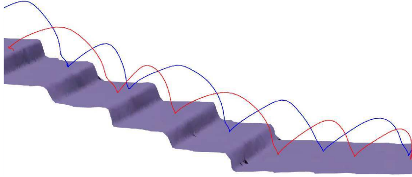
Figure 11: A1 foot swing trajectory : Foot trajectories for the visual locomotion policy in sim. The A1 learns to correctly place its front (red) and hind (blue) feet without stumbling on the stair edge. When approaching the stairs, A1 leads with the front foot, taking a large step to land securely in the middle of the second step, indicating that safe footholds can be directly inferred from vision.
