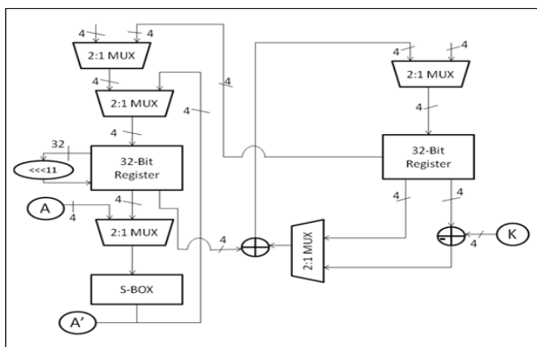
Fig.7. Data Path for LiCi-2 Cipher for 128 bit Key Scheduling
