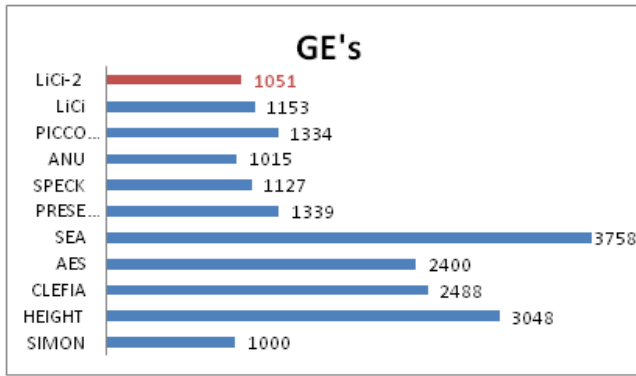
Fig.9. GE's Comparison of LiCi-2 with existing Ciphers
