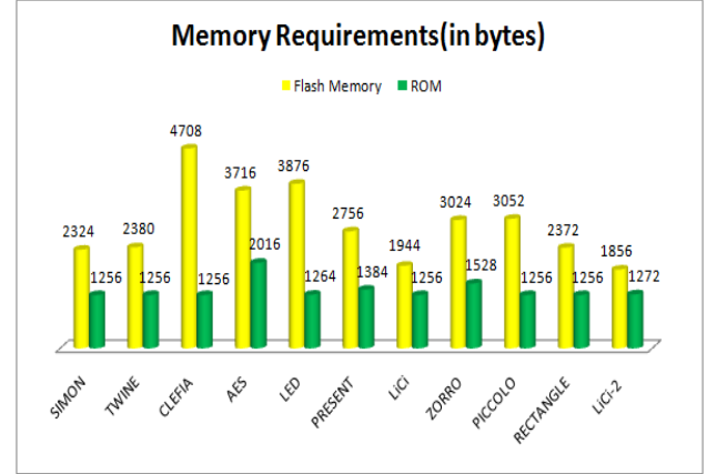
Fig. 5. Memory Requirements Comparison of LiCi-2 with existing Light Weight Ciphers
