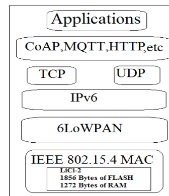
Fig. 3. Light Weight 6LoWPAN Protocol Stack
