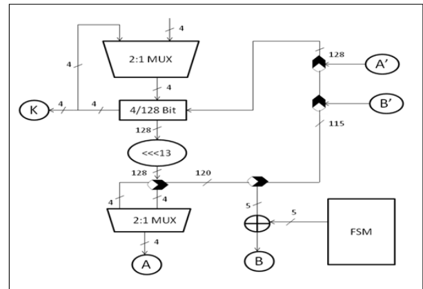
Fig.8. Key Path for LiCi-2 Cipher for 128 bit Key Scheduling
