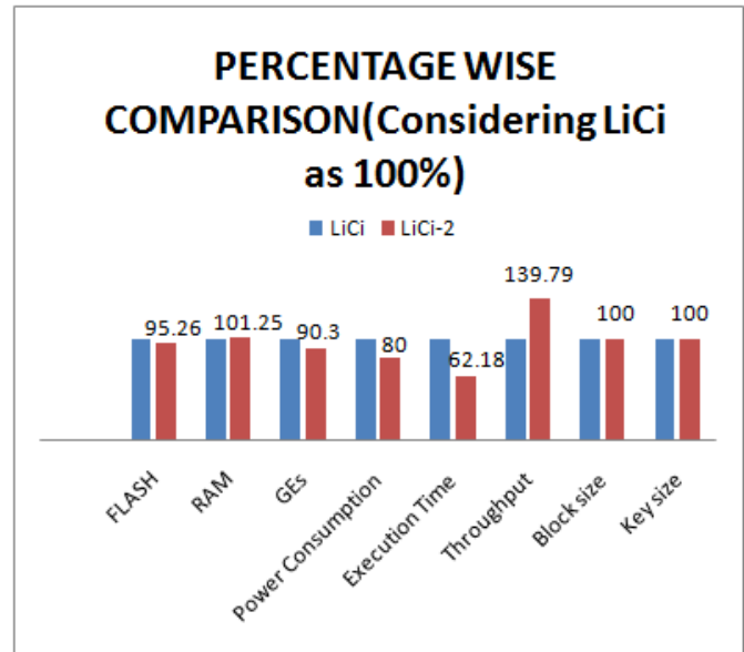
Fig.10. Statistical Comparison of LiCi and LiCi-2
