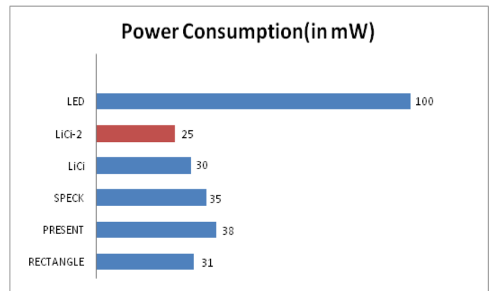
Fig. 6. Power Consumption Comparison of LiCi-2 with existing Light Weight Ciphers on Xilinx Platform.
