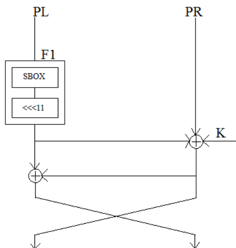
Fig. 4. A Block Cipher LiCi-2
