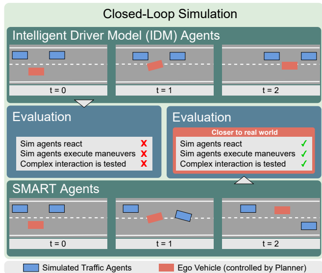
Fig. 1: Intelligent Driver Model (IDM) vs. SMART agents: same scene, different world. Starting with the same real-world scene state, the two traffic agent models lead to different scene developments when evaluating the same ego trajectory planner in a closed-loop simulation. Since the IDM cannot see vehicles in adjacent lanes it does not react to the ego vehicle’s lane change attempt and behaves passively. In contrast, SMART agents trained from real traffic data behave less passive, react to other agents across lanes and execute driving maneuvers themselves. These characteristics of the sim agents are important for testing complex interactions and for assessing a planner’s driving behavior in real-world traffic.
