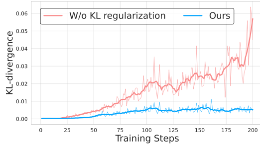
Figure 3: The effect of KL regularization on KL divergence across training steps. The model trained with KL regularization (blue) maintains a low and stable divergence, whereas the model without regularization (red) exhibits a rapid and volatile increase.
