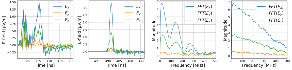
Figure 5: Left: Time-domain electric field traces for two antennas at different lateral distances from the shower core (at 50 m and at 200 m). Right: Corresponding Fourier transforms of the electric field components. A frequency dip around 100 MHz is clearly visible for the closer antenna.
