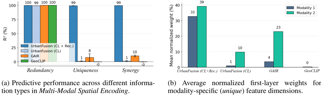
Figure 3: Empirical results on synthetic data analyzing the preservation of redundant , unique , and synergistic information using the Partial Information Decomposition (PID) framework.
