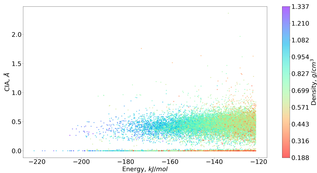
Fig. 17. CIA vs energy plot for simulated T2 crystals, coloured by their density
