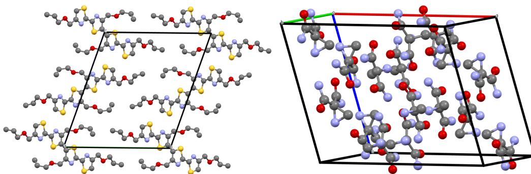
Fig. 13. Some crystals from Table 2. Left: ABEDIU01. Right: BIPCOS02.
