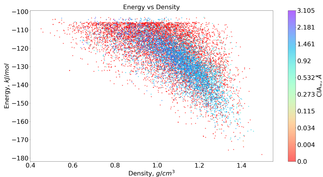
Fig. 23. Energy vs density plot for simulated and experimental T0 crystals, coloured by their CIA ∞
