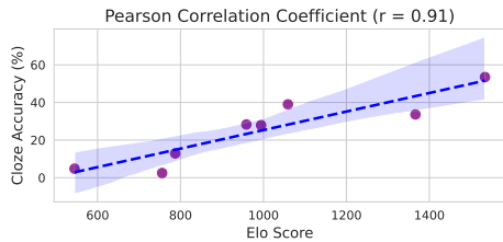
(a) Scatter plot between Elo scores and Omni-Cloze accuracy across models.
