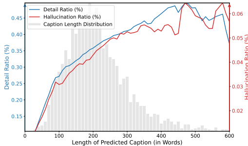
Figure 2: Relationship between caption length, detail coverage, and hallucination on Gemini-2.5-Pro in the detailed captioning task.
