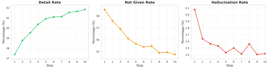
Figure 6: Trends of detail rate, not given rate, and hallucination rate vs steps in Omni-Detective.
