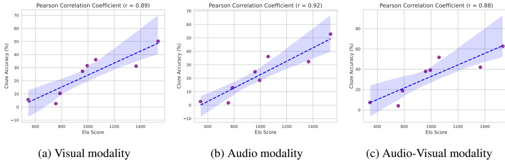
Figure 9: Scatter plots showing the relationship between Elo scores and Omni-Cloze accuracy across different modalities: (a) visual, (b) audio, and (c) audio-visual.
